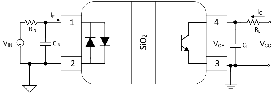
図 8-5. ISOM811(5-8) Test Circuit for Bandwidth
