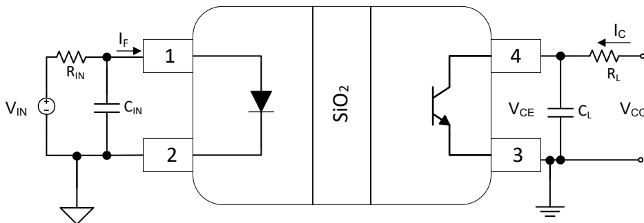
図 8-4. ISOM811(0-3) Test Circuit for Bandwidth
