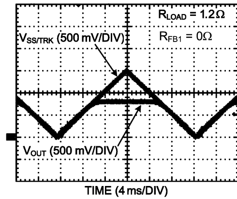
Start-Up (Tracking)
