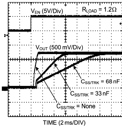
Start-Up (Soft-Start)
