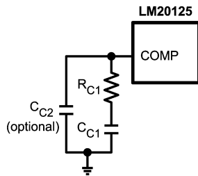
FIGURE 5. Compensation Network for LM20125
