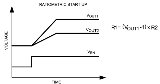
FIGURE 8. Common Start Up Sequences
