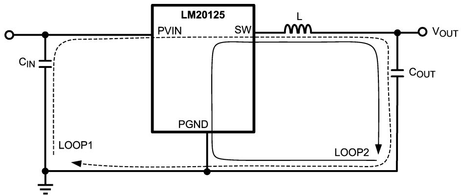
FIGURE 10. Schematic of LM20125 Highlighting Layout Sensitive Nodes
