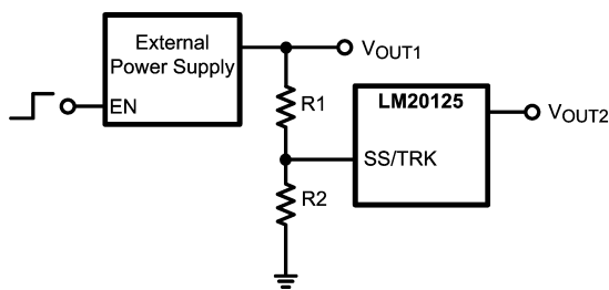
FIGURE 7. Tracking an External Supply
