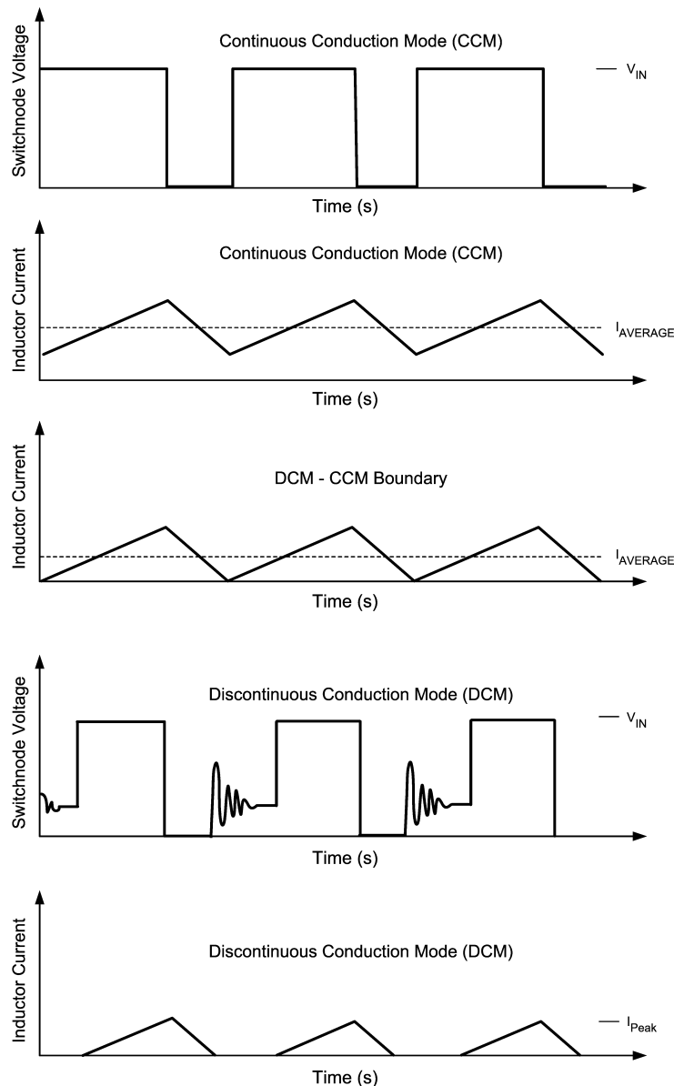
FIGURE 1. Modes of Operation for LM20125
