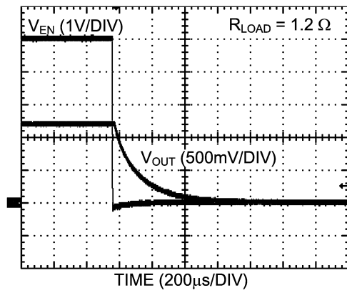
Power Down
