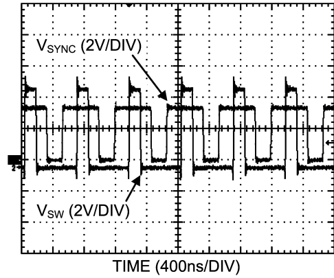
Switch Synchronization
