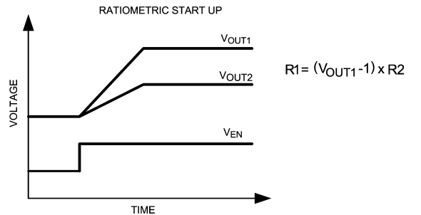
FIGURE 8. Common Start Up Sequences
