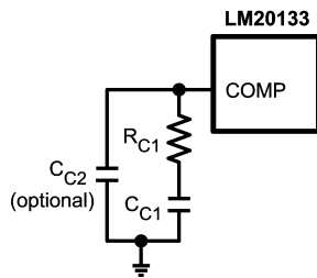
FIGURE 5. Compensation Network for LM20133
