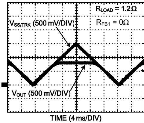
Start-Up (Tracking)
