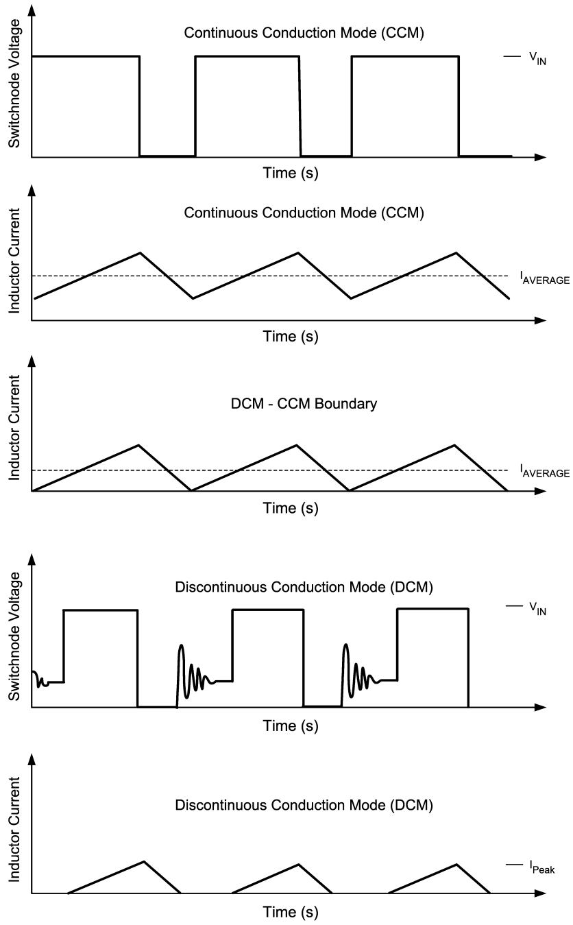
FIGURE 1. Modes of Operation for LM20133
