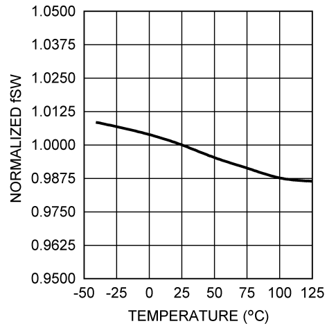
6-2. Normalized Switching Frequency vs Temperature
