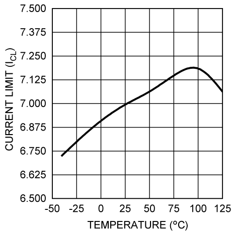
6-3. Current Limit vs Temperature
