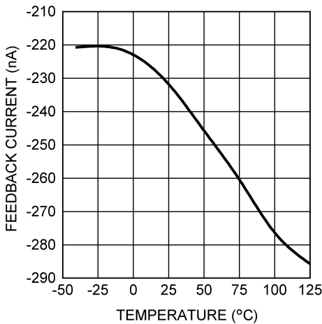
6-5. Feedback Bias Current vs Temperature
