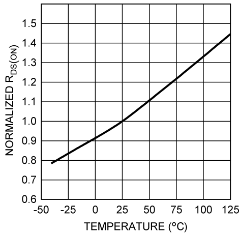
6-4. Normalized R_{DS(ON)} vs Temperature
