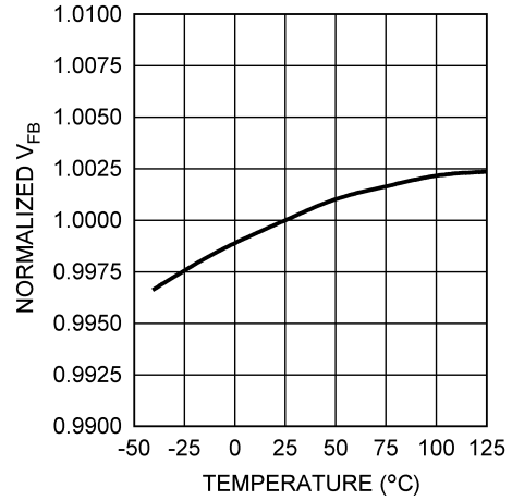
6-8. Normalized Feedback Voltage vs Temperature
