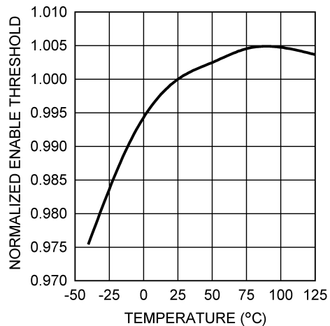
6-6. Normalized Enable Threshold Voltage vs Temperature
