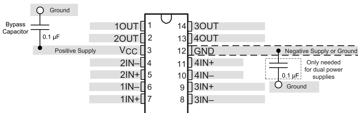
10-1. LM2901x-Q1 Layout Example
