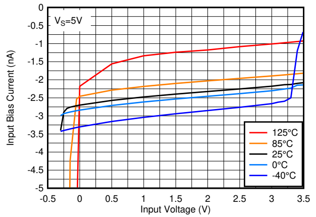
6-16. Input Bias Current vs. Input Voltage at 5V
