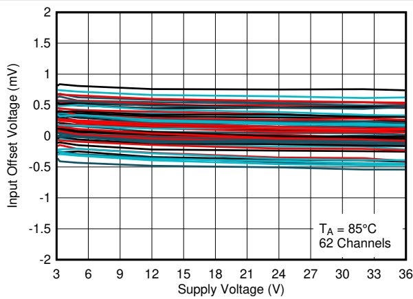
6-13. Input Offset Voltage vs. Supply Voltage at 85°C
