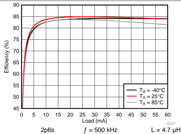
109. Backlight Boost Efficiency
