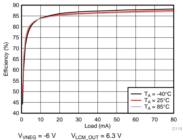
129. VNEG Efficiency
