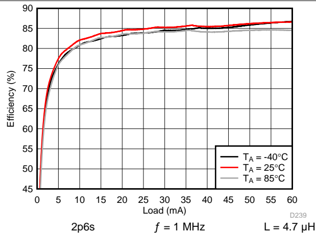
107. Backlight Boost Efficiency
