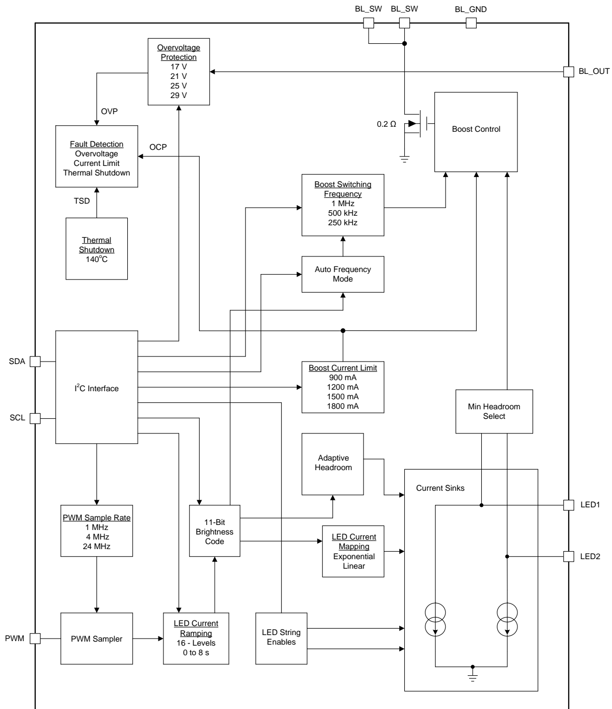
30. Backlight Block Diagram
