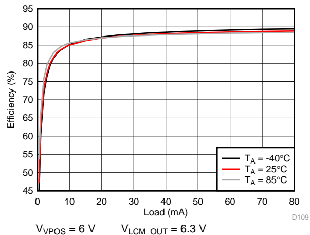
123. VPOS Efficiency
