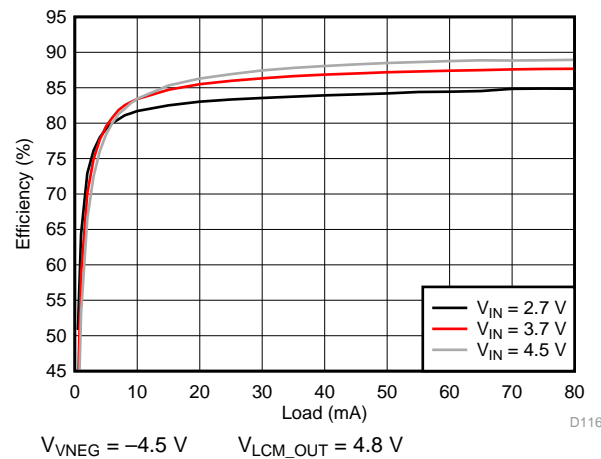
130. VNEG Efficiency
