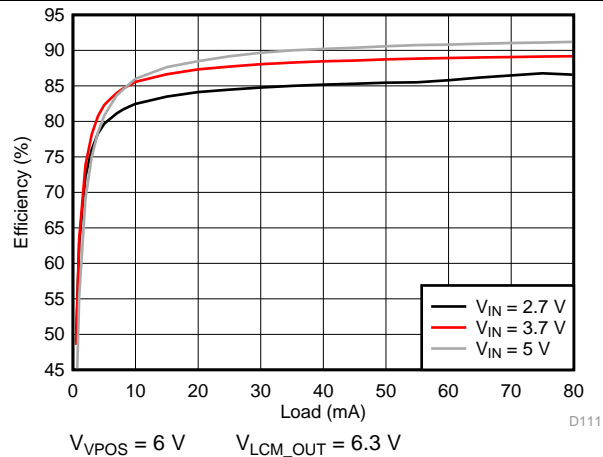
125. VPOS Efficiency
