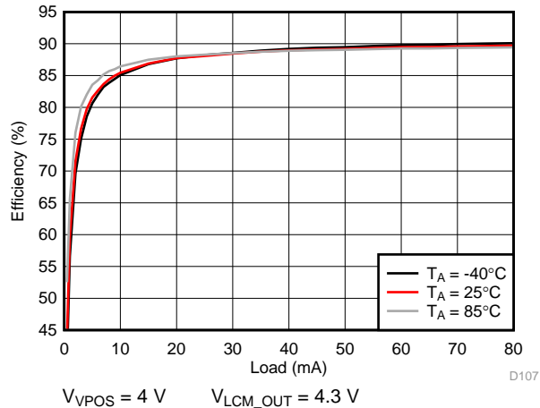
121. VPOS Efficiency
