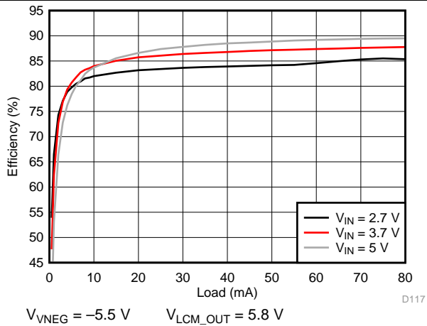
131. VNEG Efficiency
