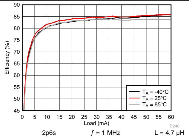
108. Backlight System Efficiency
