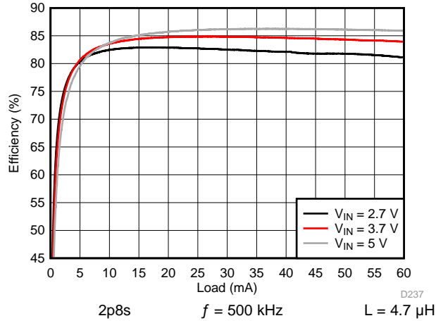
105. Backlight Boost Efficiency
