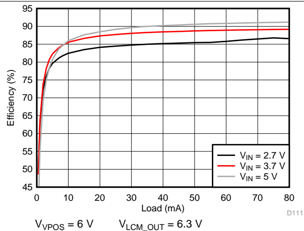
161. VPOS Efficiency
