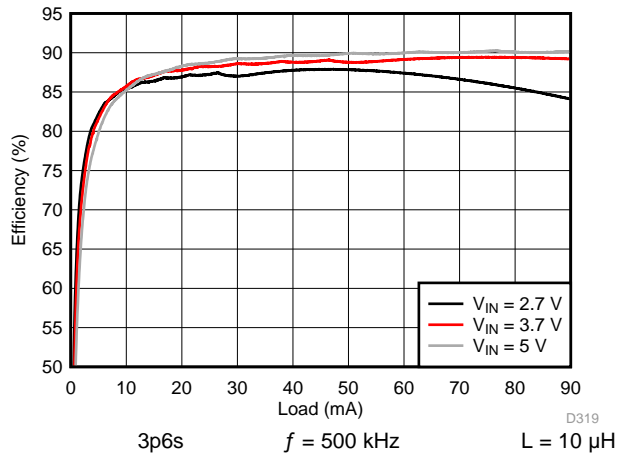
133. Backlight Boost Efficiency
