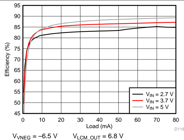
168. VNEG Efficiency
