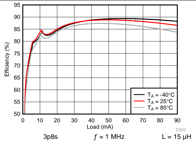
134. Backlight System Efficiency
