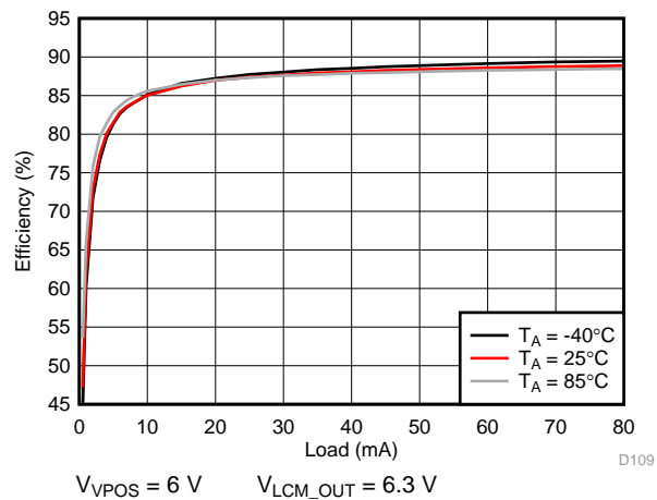
159. VPOS Efficiency
