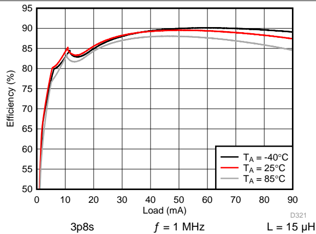
133. Backlight Boost Efficiency
