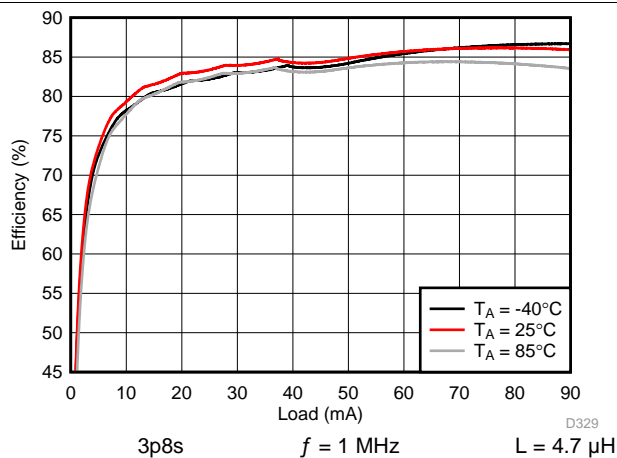
141. Backlight Boost Efficiency
