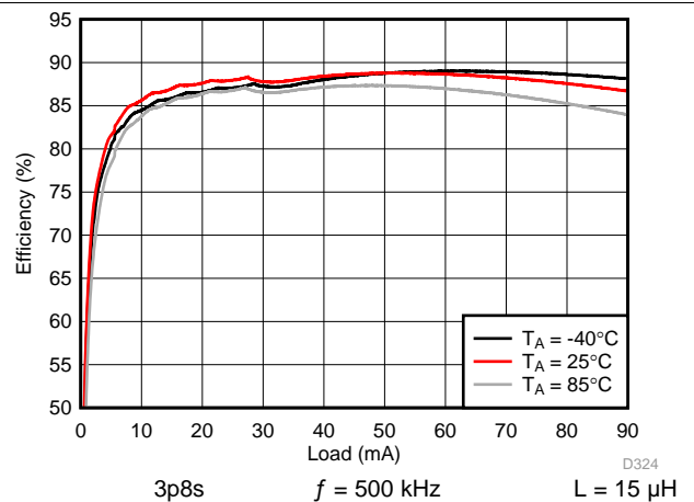
136. Backlight System Efficiency
