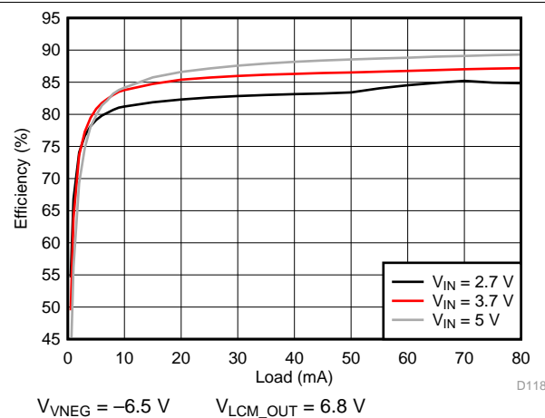
204. VNEG Efficiency
