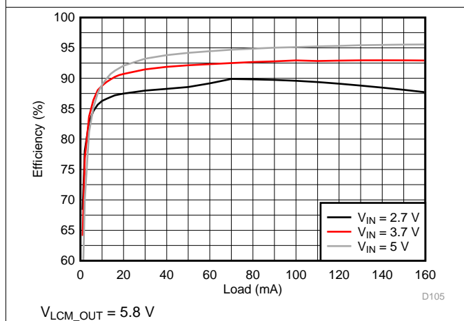
图 191. LCM Boost Efficiency
