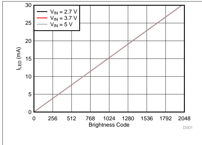
图 2. Backlight LED Current, Linear Control
