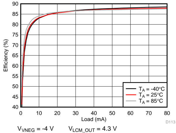
199. VNEG Efficiency
