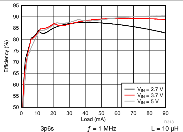
130. Backlight System Efficiency
