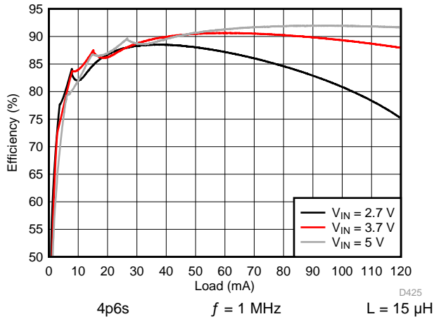
175. Backlight Boost Efficiency
