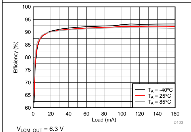
图 189. LCM Boost Efficiency
