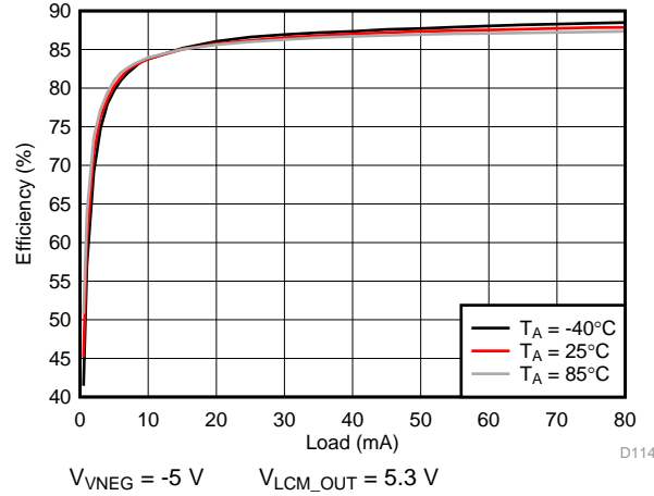
200. VNEG Efficiency
