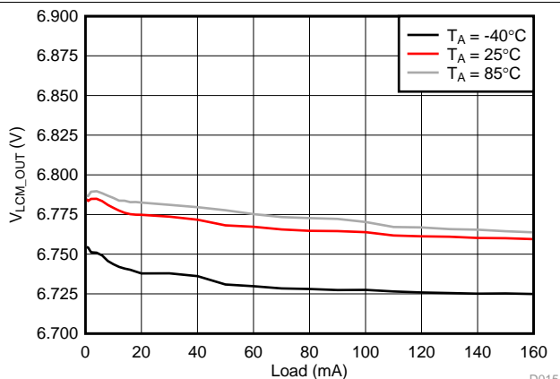
16. V_{LCM\_OUT} Load Regulation
