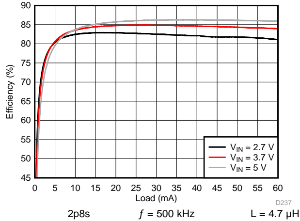
105. Backlight Boost Efficiency
