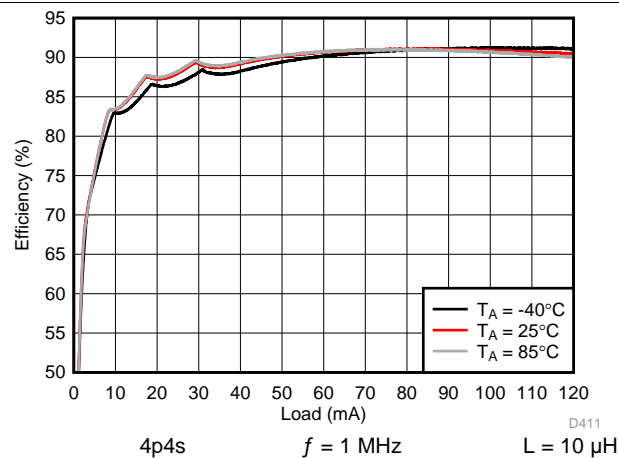
159. Backlight Boost Efficiency
