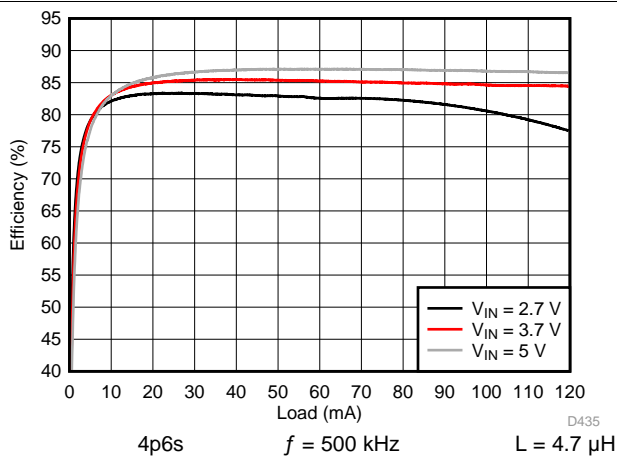
183. Backlight Boost Efficiency
