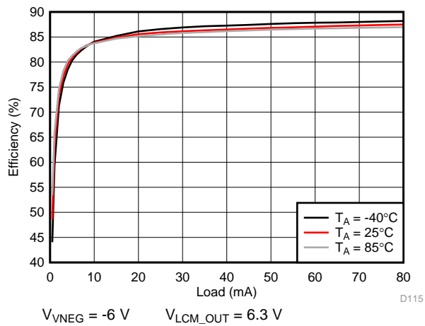
201. VNEG Efficiency
