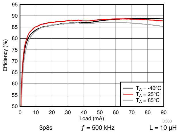
115. Backlight Boost Efficiency
