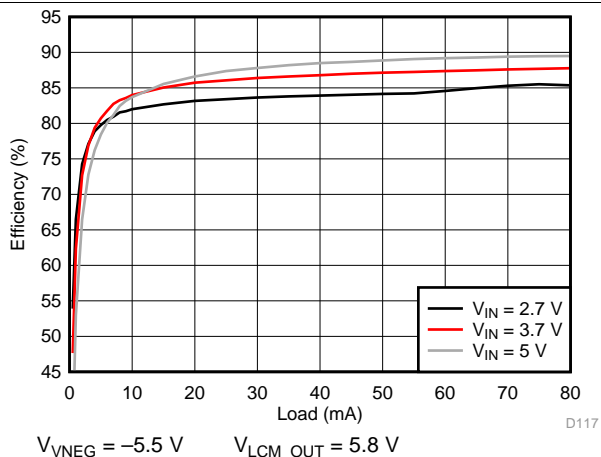
203. VNEG Efficiency
