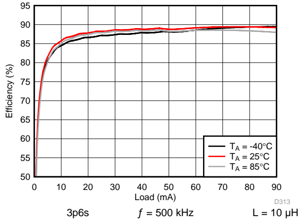
127. Backlight Boost Efficiency
