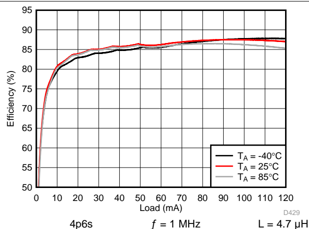
177. Backlight Boost Efficiency
