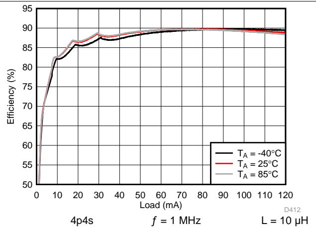
160. Backlight System Efficiency
