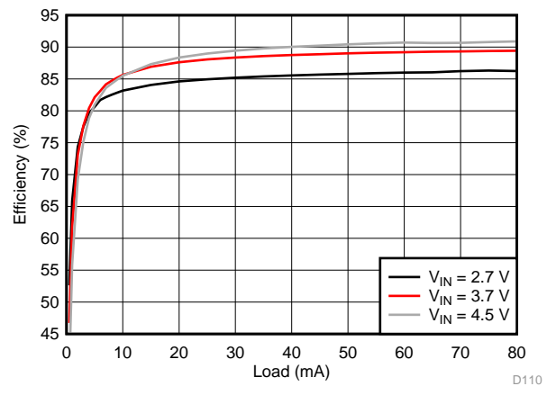
196. VPOS Efficiency
