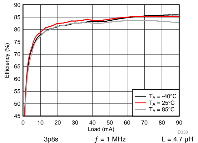
142. Backlight System Efficiency
