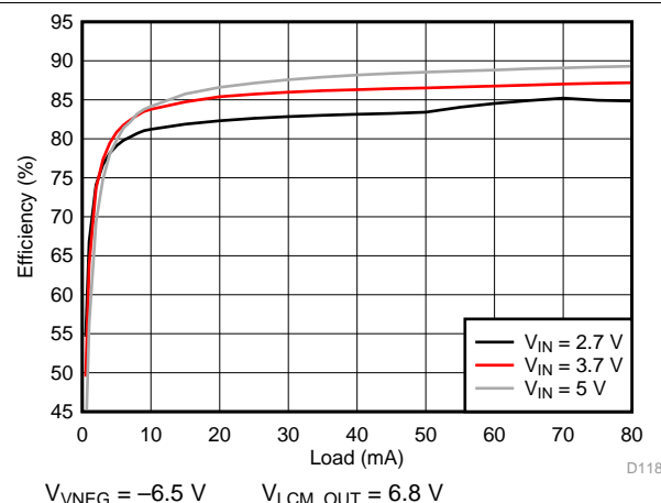
204. VNEG Efficiency
