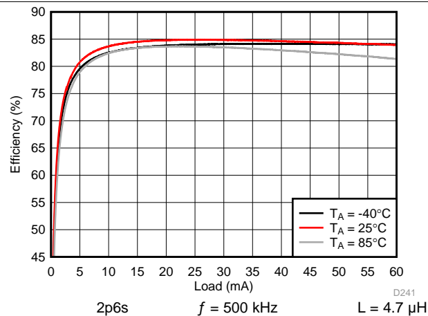
109. Backlight Boost Efficiency
