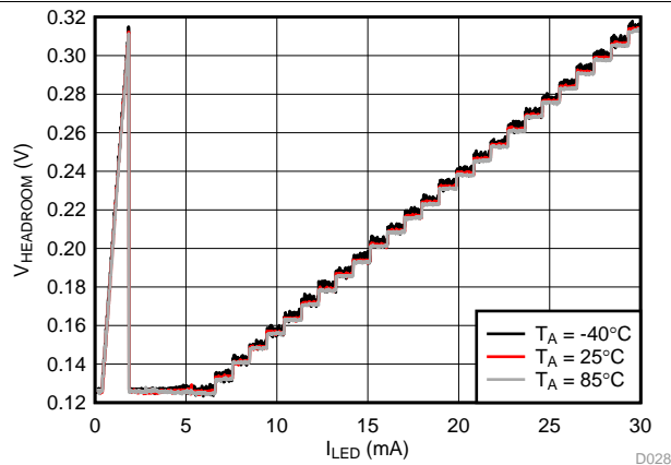
14. Backlight Regulated Headroom Voltage
