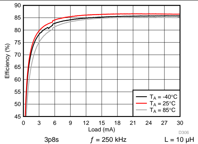
118. Backlight System Efficiency
