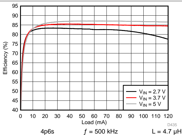
183. Backlight Boost Efficiency
