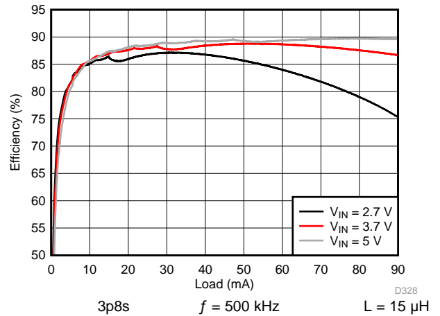
140. Backlight System Efficiency
