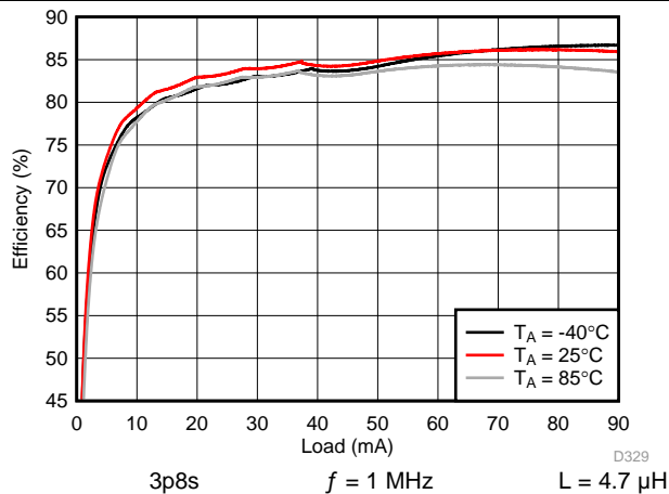
141. Backlight Boost Efficiency
