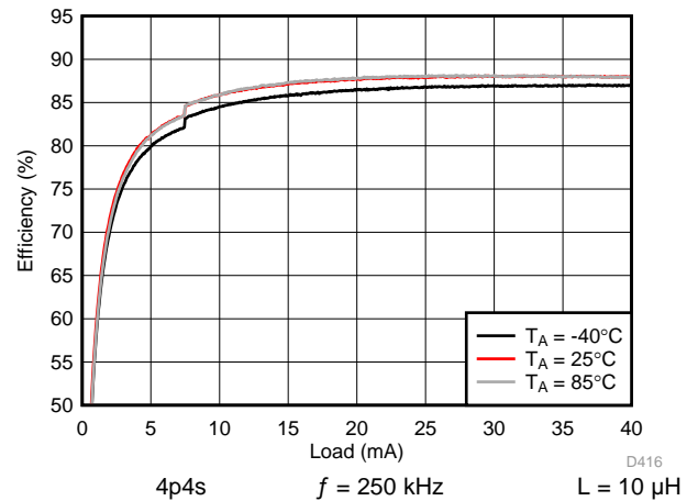
164. Backlight System Efficiency
