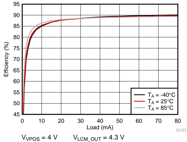
193. VPOS Efficiency
