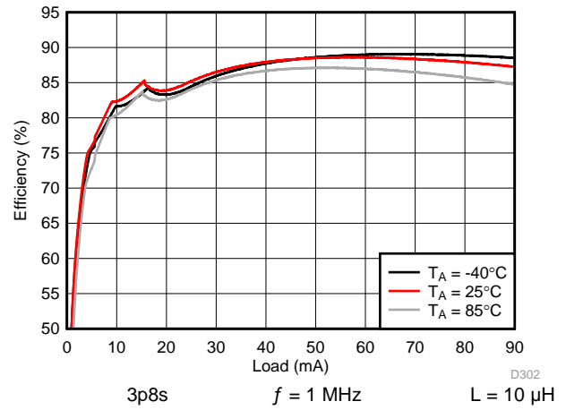
116. Backlight System Efficiency
