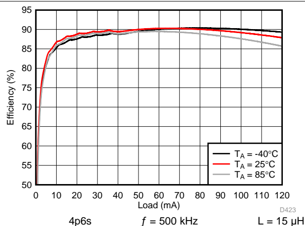
图 171. Backlight Boost Efficiency
