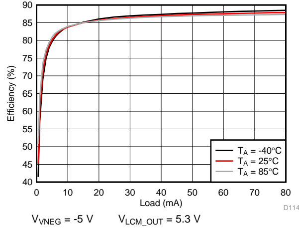
200. VNEG Efficiency
