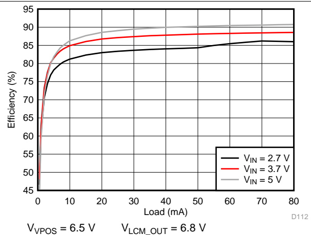
198. VPOS Efficiency
