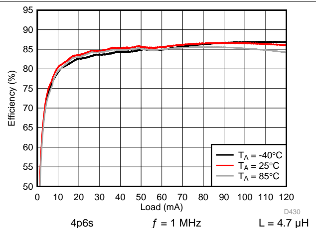
178. Backlight System Efficiency
