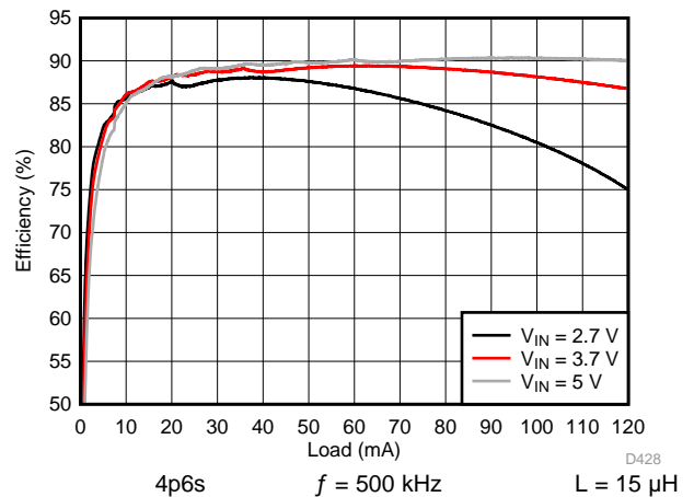
176. Backlight System Efficiency
