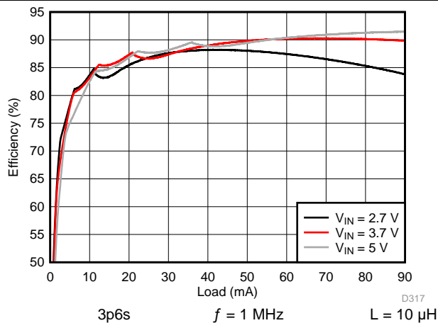
129. Backlight Boost Efficiency
