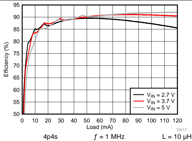
165. Backlight Boost Efficiency
