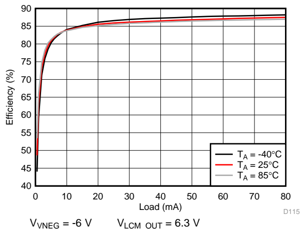
201. VNEG Efficiency
