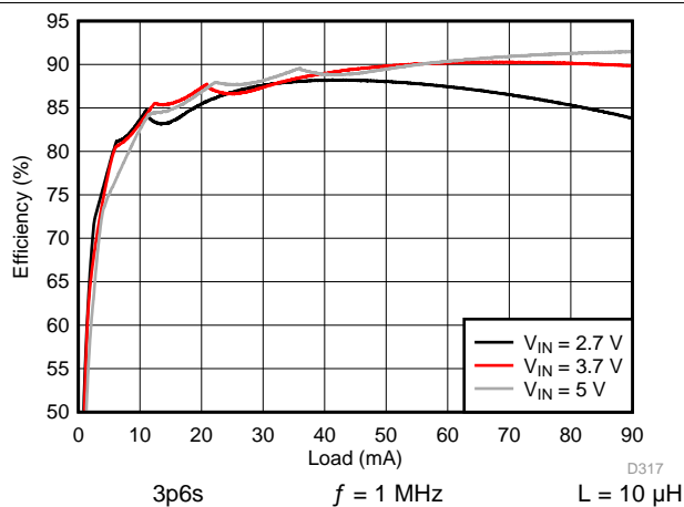
129. Backlight Boost Efficiency
