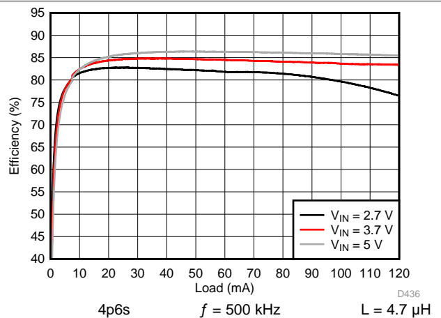
184. Backlight System Efficiency
