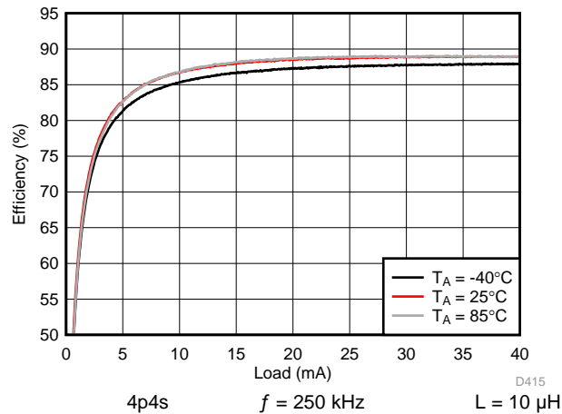
163. Backlight Boost Efficiency
