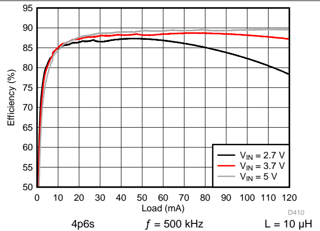
158. Backlight System Efficiency
