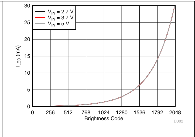
图 3. Backlight LED Current, Exponential Control
