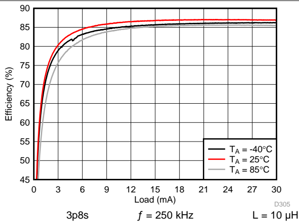
117. Backlight Boost Efficiency
