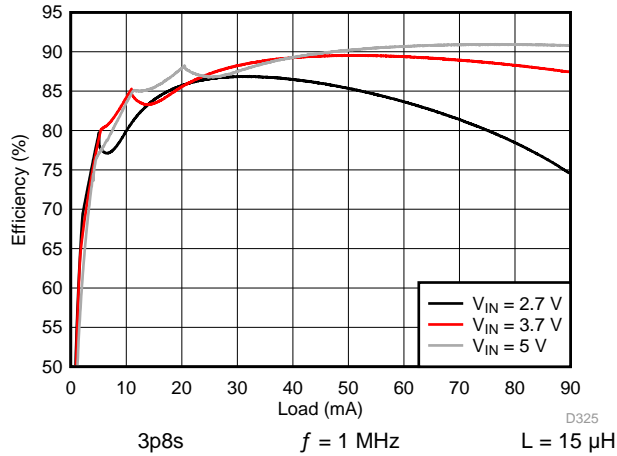
139. Backlight Boost Efficiency
