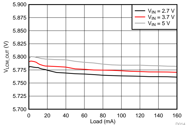
15. V_{LCM\_OUT} Load Regulation
