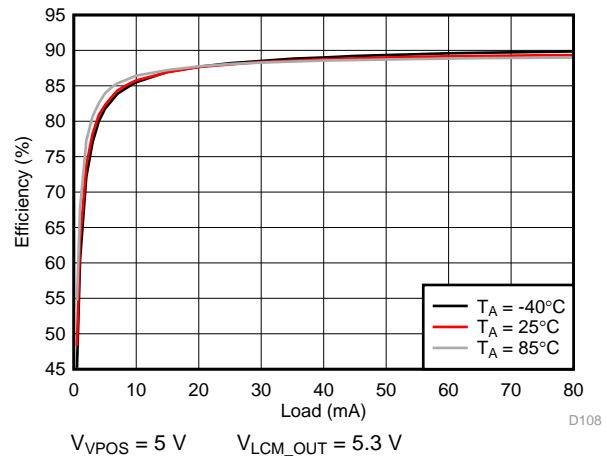
194. VPOS Efficiency
