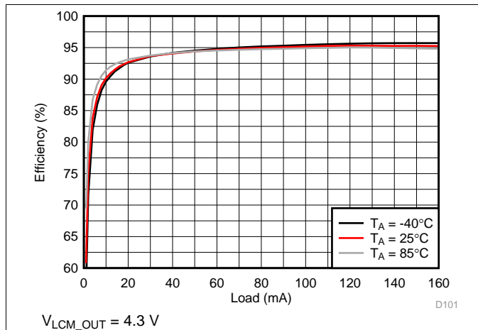
图 187. LCM Boost Efficiency
