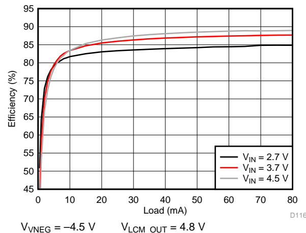
202. VNEG Efficiency
