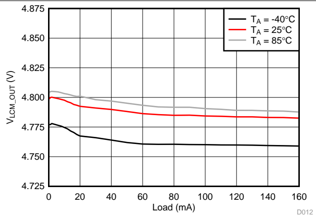
15. V_{LCM\_OUT} Load Regulation
