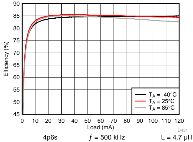
181. Backlight Boost Efficiency
