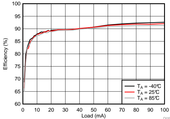
V_{LCM\_OUT} = 5.5 V
