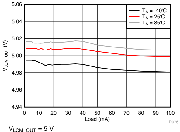
Figure 97. V_{LCM\_OUT} Load Regulation
