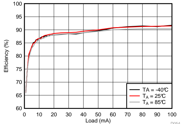
V_{LCM\_OUT} = 6 V
