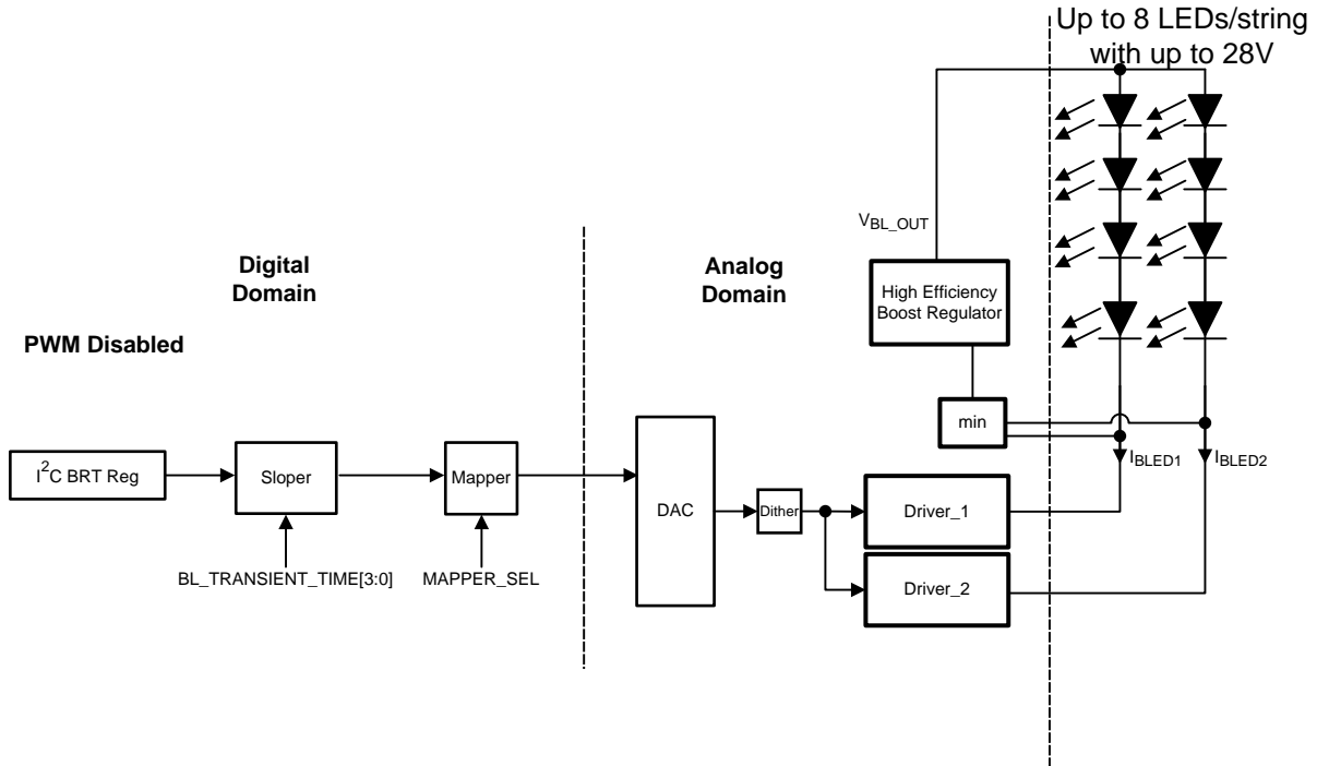
Figure 24. Brightness Control with PWM Bit Disabled
