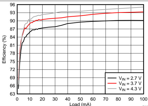
V_{LCM\_OUT} = 4.8 V
