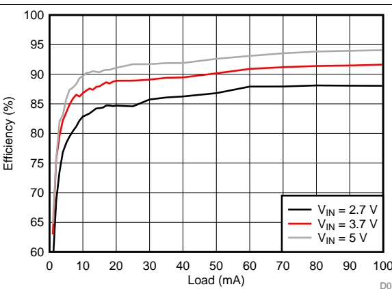
V_{LCM\_OUT} = 5.9 V
