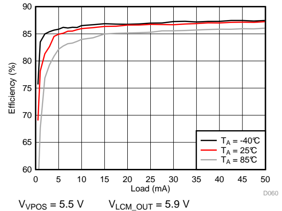
Figure 81. VPOS Efficiency
