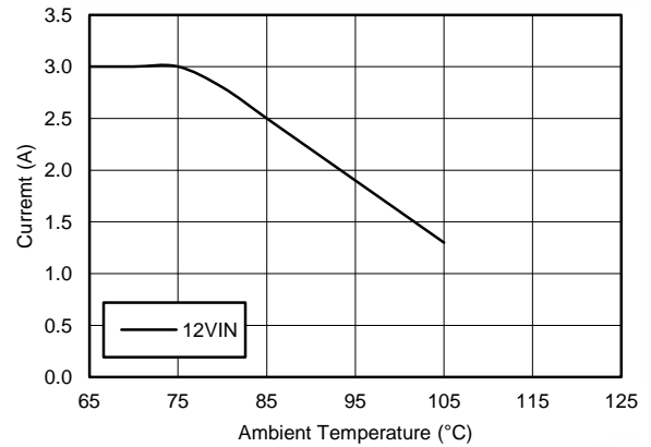
Figure 90. Derating Curve
