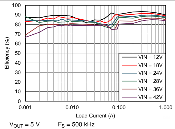
Figure 2. Efficiency
