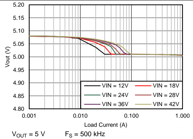
Figure 8. V_{OUT} Regulation
