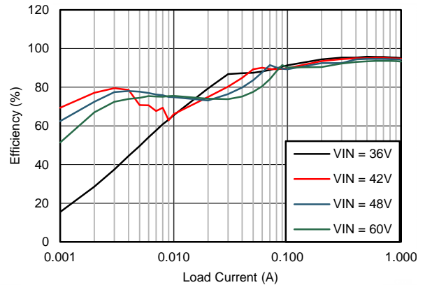
Figure 78. Efficiency
