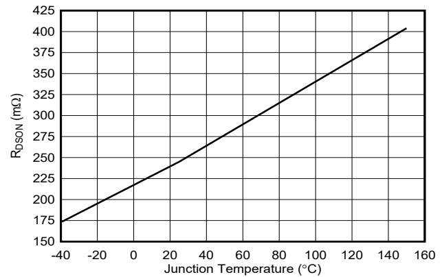
6-6. MOSFETs On-State Resistance Versus Temperature
