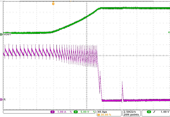
8-8. Short Circuit Recovery
