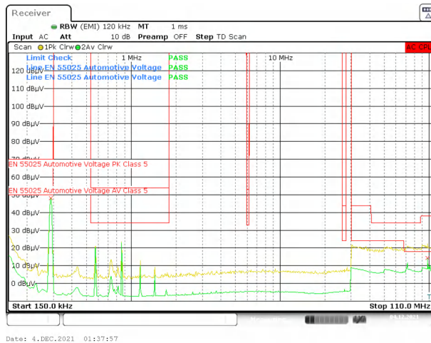
8-10. Full-Load Switching
