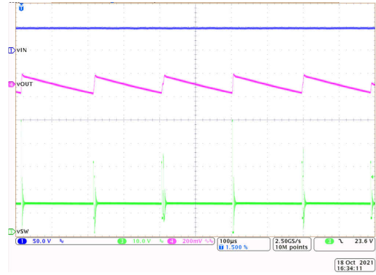
8-9. Light-Load Switching
