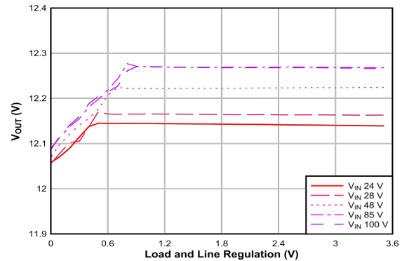
6-2. Load and Line Regulation
