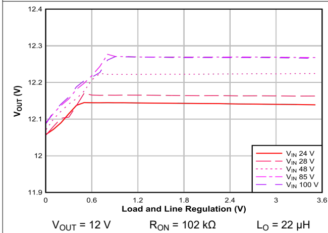
8-4. Load and Line Regulation Performance
