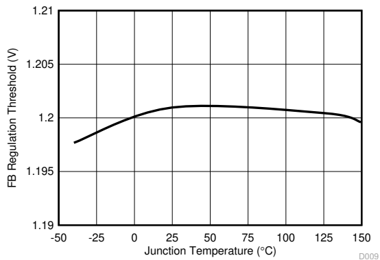
6-5. Feedback Comparator Threshold Versus Temperature
