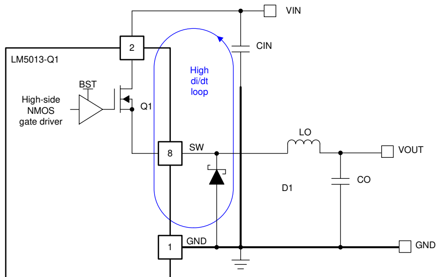
FIG 10-1. DC/DC Buck Converter With Power Stage Circuit Switching Loop
