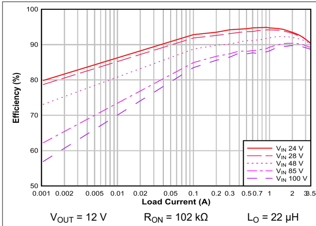
8-2. Conversion Efficiency (Log Scale)
