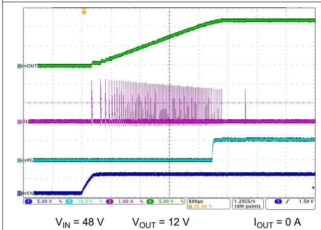
8-6. No-Load Start-Up with EN/UVLO
