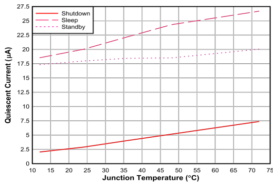
6-3. Shutdown, Sleep, and Supply Current Versus Temperature
