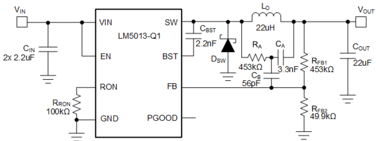
図 8-1. Typical Application, V_{IN(nom)} = 48\text{ V} , V_{OUT} = 12\text{ V} , I_{OUT(max)} = 3.5\text{ A} , F_{SW(nom)} = 300\text{ kHz}
