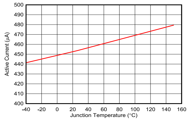
6-4. V_{IN} Active Current Versus Temperature
