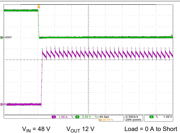
8-7. Short Circuit Applied
