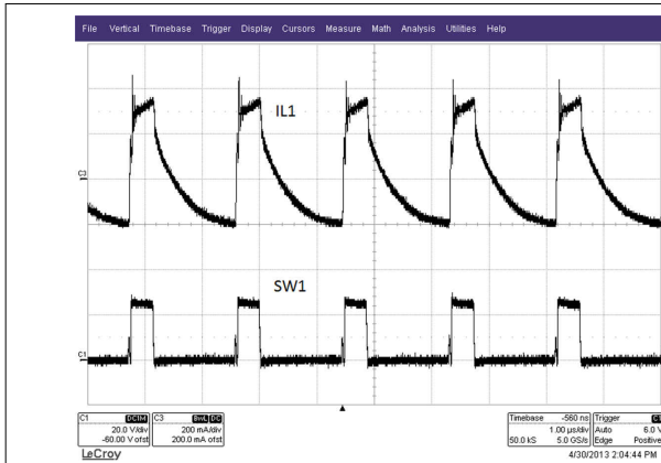
8-9. Steady State Waveform (V IN = 48 V, I OUT1 = 100 mA, I OUT2 = 200 mA)
