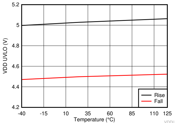
6-12. VDD UVLO Threshold
