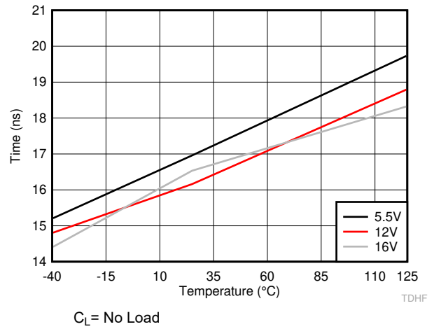
6-21. HO Falling Propagation Delay (TDHFF)
