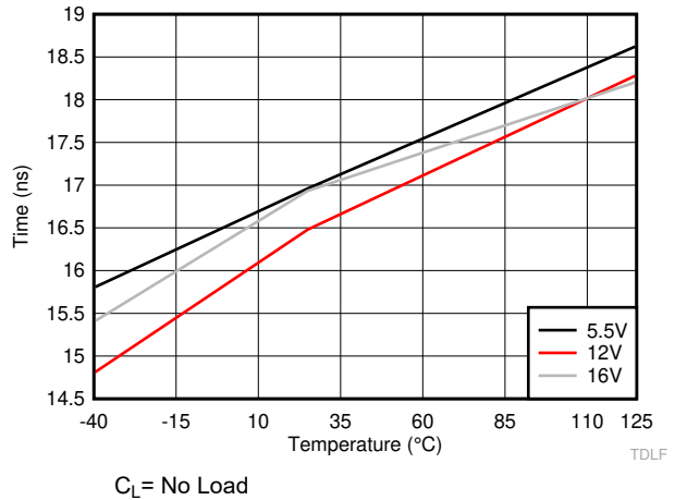
6-23. LO Falling Propagation Delay (TDLFF)
