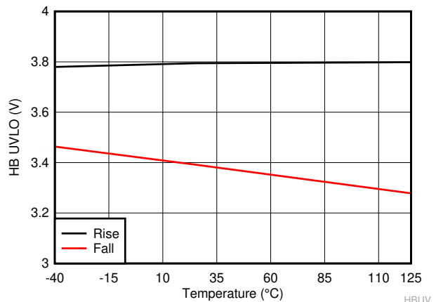
6-13. HB UVLO Threshold
