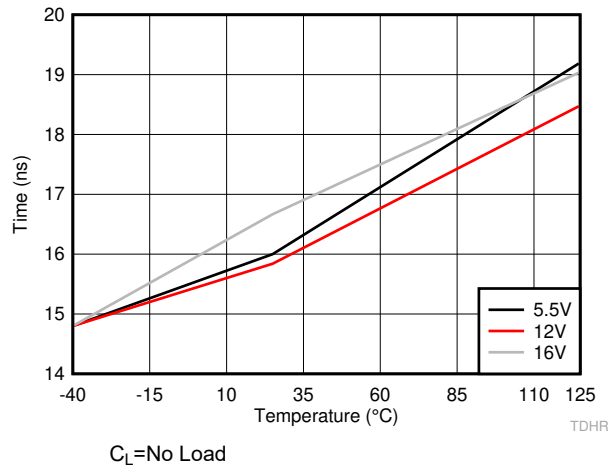
6-20. HO Rising Propagation Delay (TDHRR)
