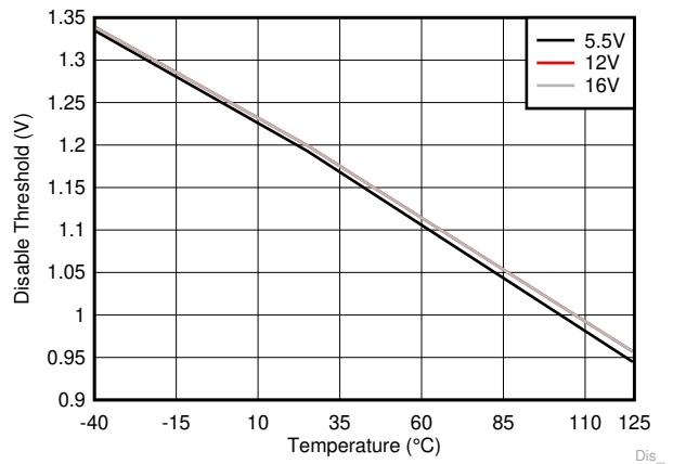
6-11. Disable Threshold
