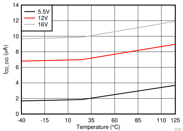
C_L = 0\text{ F} V_{EN} = 0\text{ V} 6-6. VDD Current When Disabled
