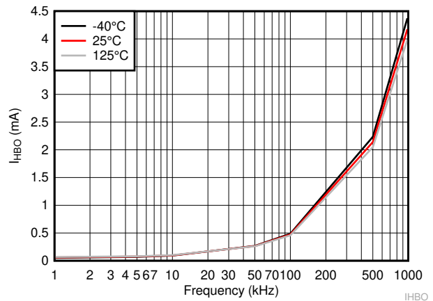
C_L = 0\text{ F} V_{DD} = V_{HB} = 12\text{ V} 6-5. HB Operating Current
