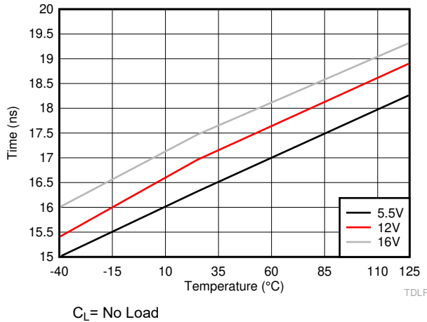
6-22. LO Rising Propagation Delay (TDLRR)
