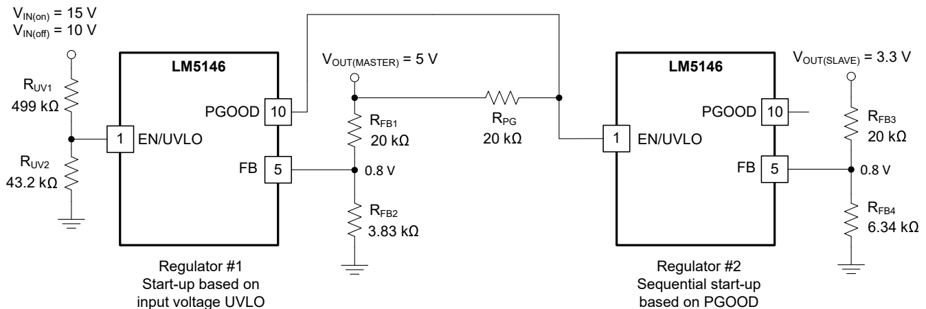
8-4. Master-Slave Sequencing Implementation Using PGOOD and EN/UVLO
