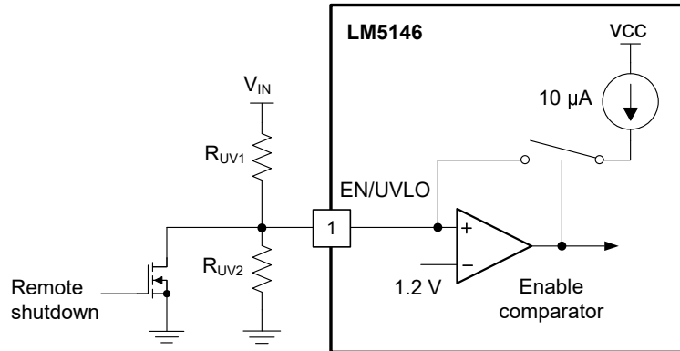
8-3. Programmable Input Voltage UVLO Turn-on and Turn-off
