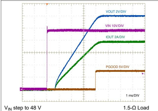
图 9-19. Start-Up, 8-A Resistive Load
