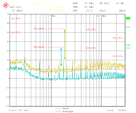
8-14. No-Load Switching
