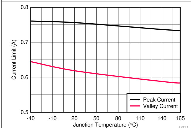
6-9. Peak and Valley Current Limit versus Temperature
