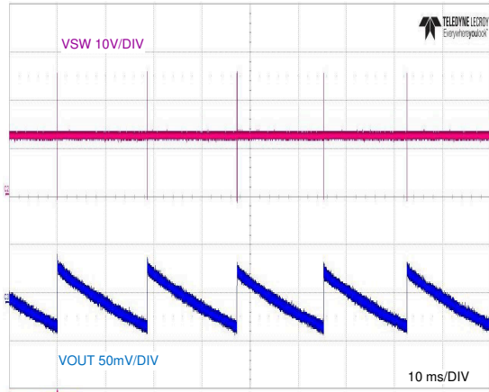
8-14. No-Load Switching
