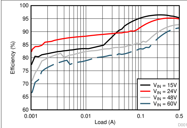
Figure 6-1. Conversion Efficiency (Log Scale)
