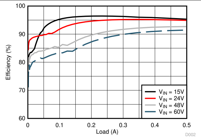
Figure 6-2. Conversion Efficiency (Linear Scale)
