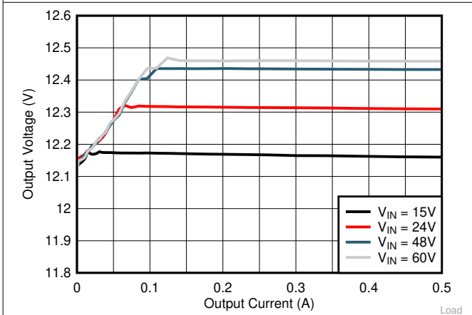
8-4. Load and Line Regulation Performance
