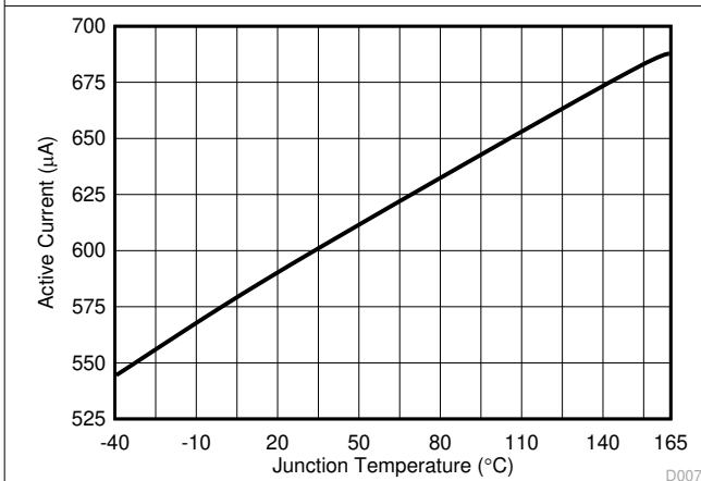
Figure 6-5. V_{IN} Active Current versus Temperature
