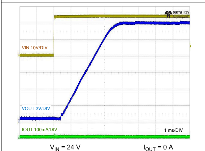
8-6. No-Load Start-up with VIN
