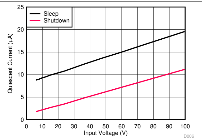
Figure 6-4. V_{IN} Shutdown and Sleep Supply Current versus Input Voltage
