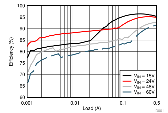
8-2. Conversion Efficiency (Log Scale)
