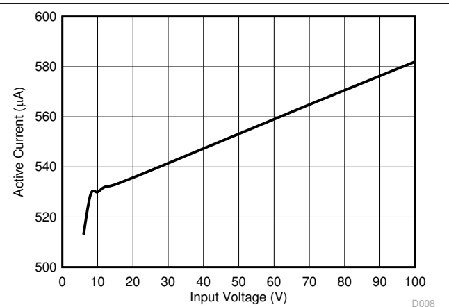
Figure 6-6. V_{IN} Active Current versus Input Voltage
