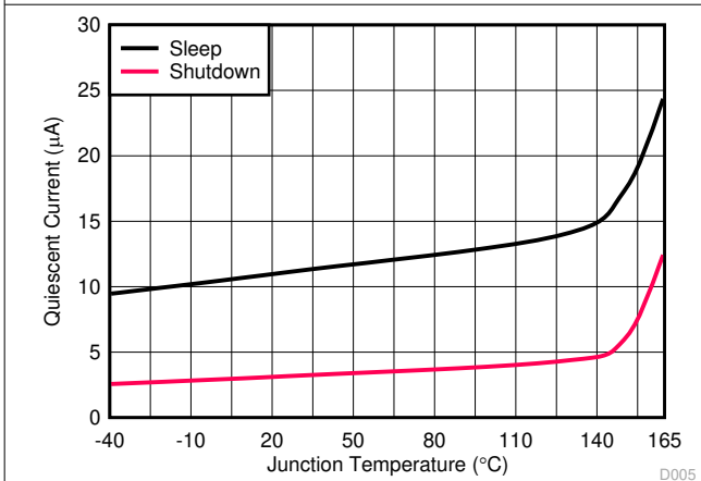
Figure 6-3. V_{IN} Shutdown and Sleep Supply Current versus Temperature
