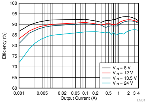
图 9-5. LM61440 Efficiency
