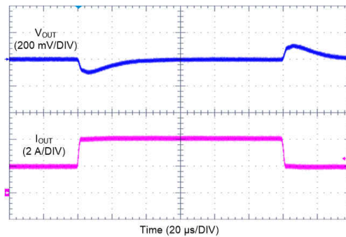
9-32. LM61440 Load Transient
