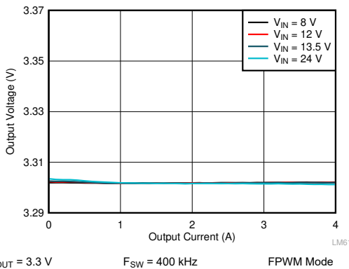
图 9-9. LM61440 Load and Line Regulation
