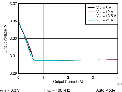
图 9-8. LM611440 Load and Line Regulation
