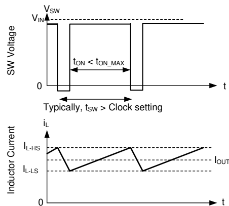
☒ 9-12. Current Limit Waveforms
