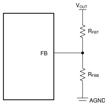
☒ 9-11. Setting Output Voltage of Adjustable Versions
