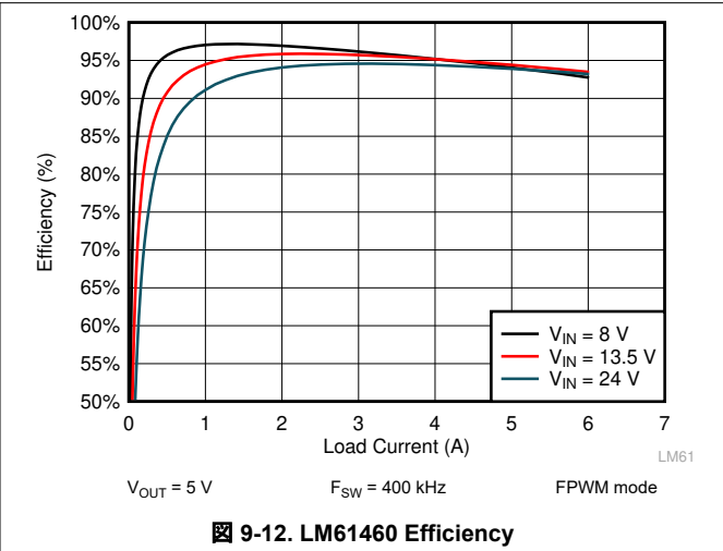
9-12. LM61460 Efficiency
