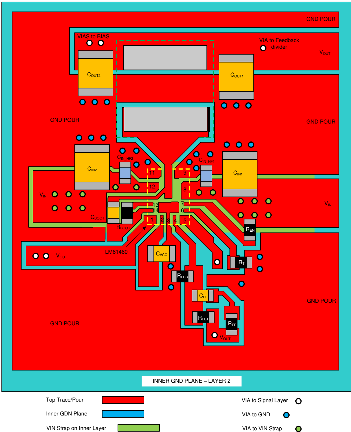
11-2. Layout Example
