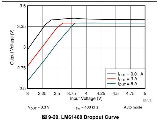
9-29. LM61460 Dropout Curve
