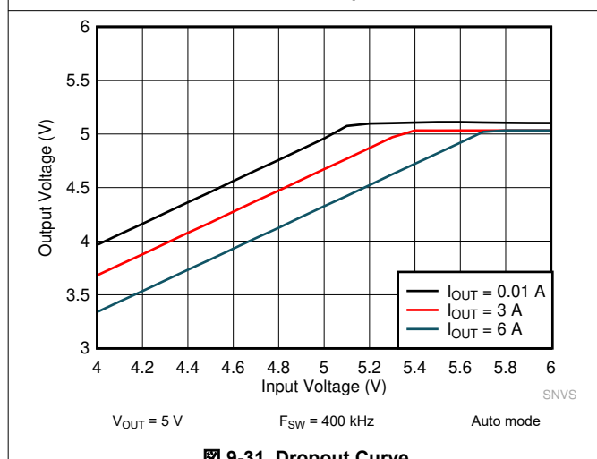
9-31. Dropout Curve
