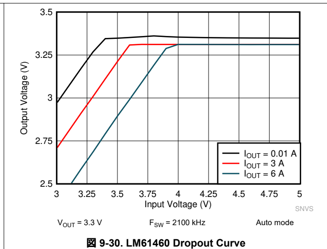
9-30. LM61460 Dropout Curve
