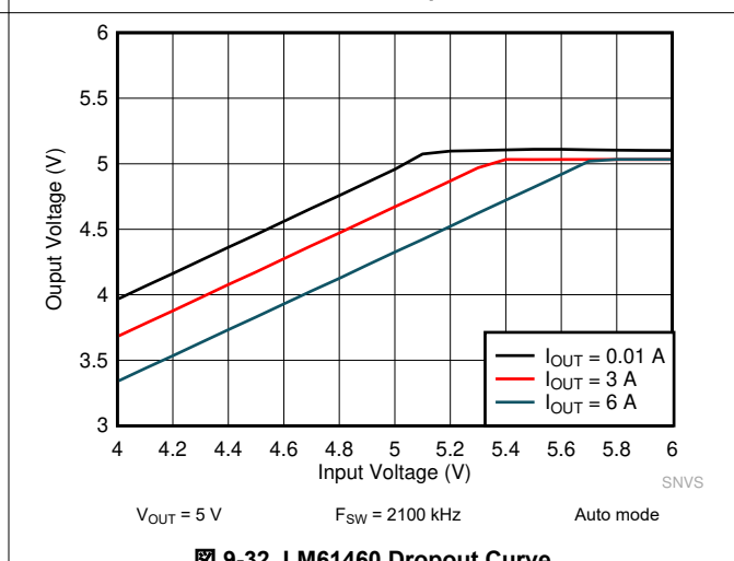
9-32. LM61460 Dropout Curve
