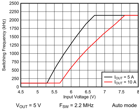
9-27. Frequency Dropout
