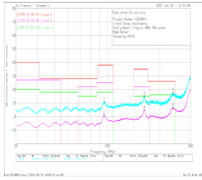
9-47. Radiated EMI Bicon Horizontal versus CISPR25 Class 5 Limits
