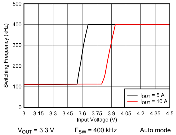
9-26. Frequency Dropout
