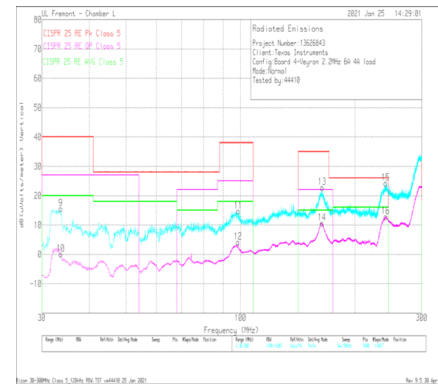
9-54. Radiated EMI Bicon Vertical versus CISPR25 Class 5 Limits
