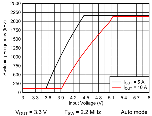
9-28. Frequency Dropout
