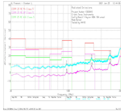
9-48. Radiated EMI Bicon Vertical versus CISPR25 Class 5 Limits
