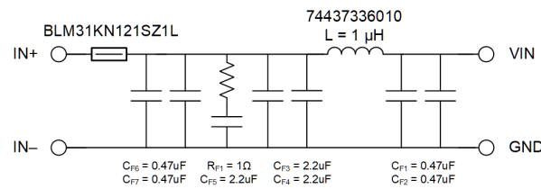
9-57. Recommended Input EMI Filter
