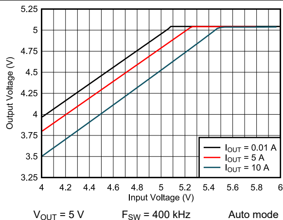
9-21. Dropout
