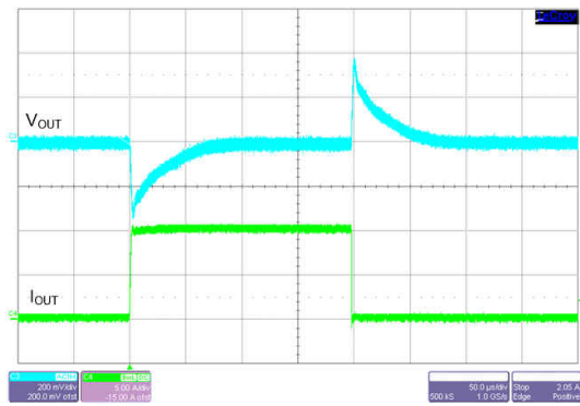
9-41. Load Transient
