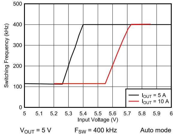
9-25. Frequency Dropout
