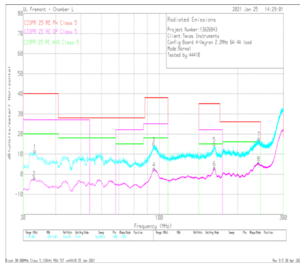
9-53. Radiated EMI Bicon Horizontal versus CISPR25 Class 5 Limits
