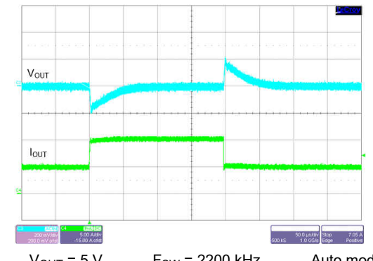
9-43. Load Transient
