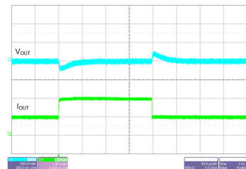
9-42. Load Transient
