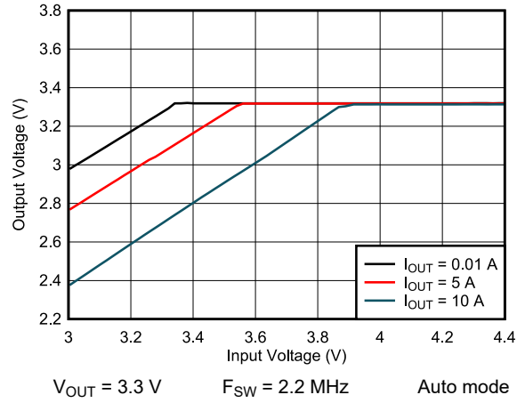
9-24. Dropout
