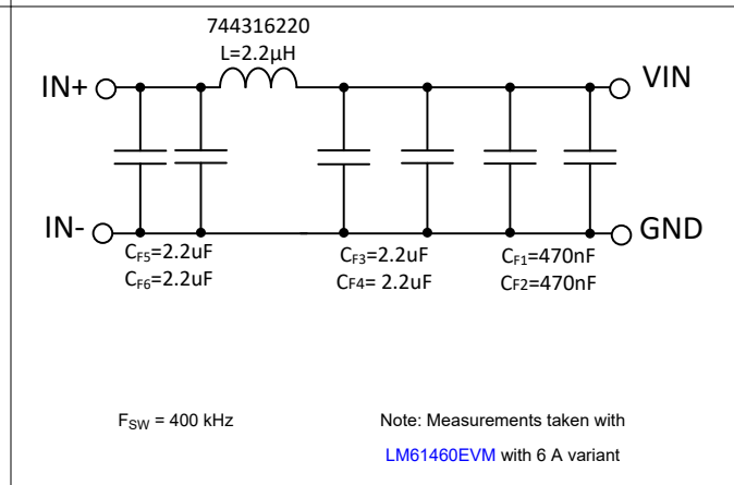
9-32. Recommended Input EMI Filter
