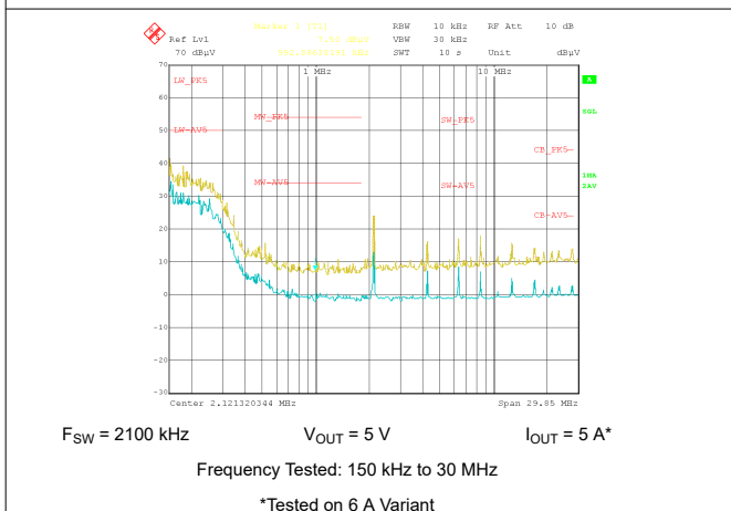
9-33. Conducted EMI versus CISPR25 Limits (Yellow: Peak Signal, Blue: Average Signal)
