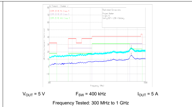
9-30. Radiated EMI Log Vertical versus CISPR25 Limits
