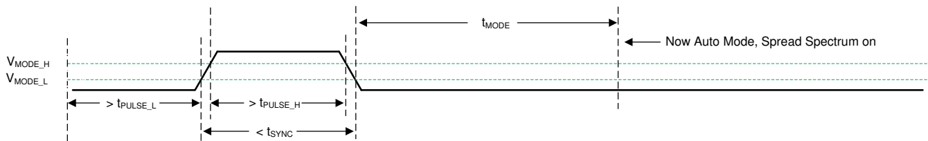
8-10. Transition from SYNC Mode to Auto Mode
