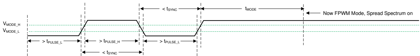
8-11. Transition from SYNC Mode to FPWM Mode
