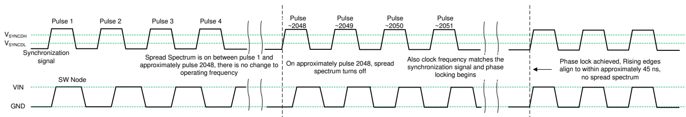
8-12. Synchronization Process
