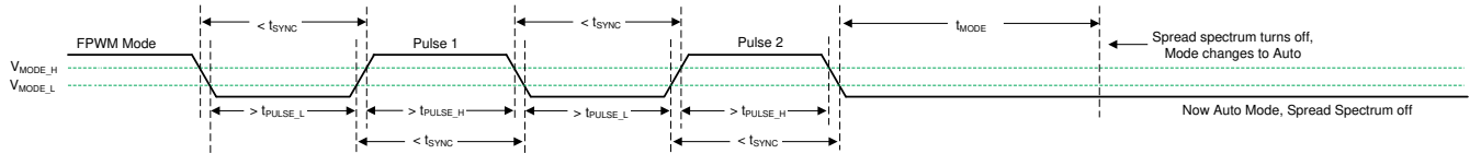
8-8. Spread Spectrum Disabled in Transition from FPWM Mode to Auto Mode
