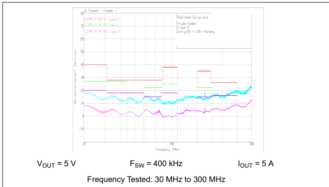
9-29. Radiated EMI Bicon Horizontal versus CISPR25 Limits
