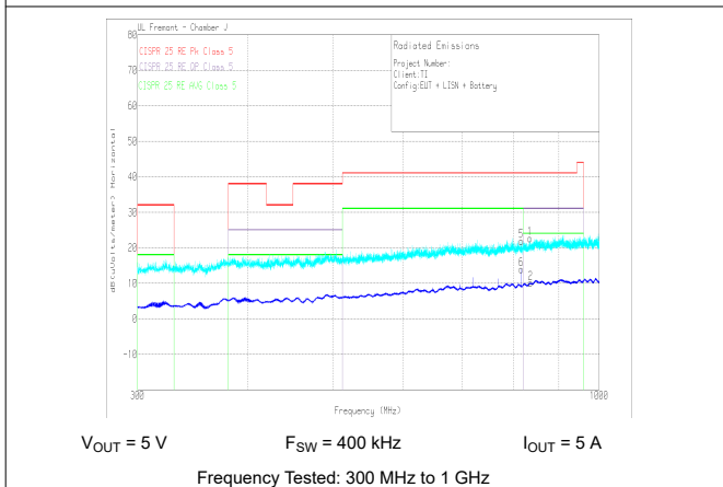
9-31. Radiated EMI Log Horizontal versus CISPR25 Limits
