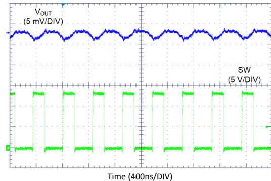
图 9-18. LM62435-Q1 Switching Waveform and V_{OUT} Ripple
