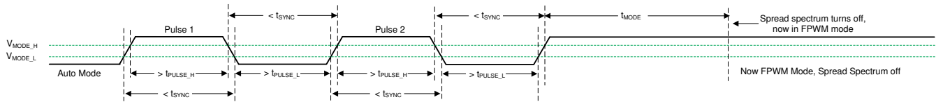
8-9. Spread Spectrum Disabled in Transition from Auto Mode to FPWM Mode
