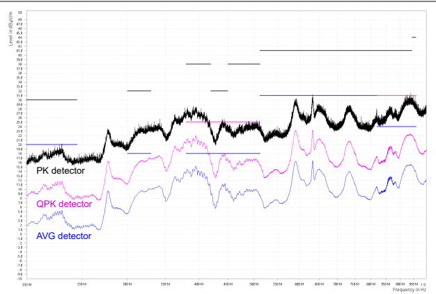
9-19. CISPR 25 Class 5 Radiated EMI, Log Antenna, Vertical Polarization, 200 MHz to 1 GHz
