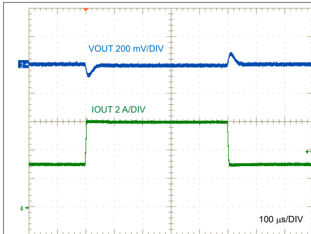
図 9-25. LM63460-Q1 Load Transient, I_{OUT} = 3 \text{ A to } 6 \text{ A}
