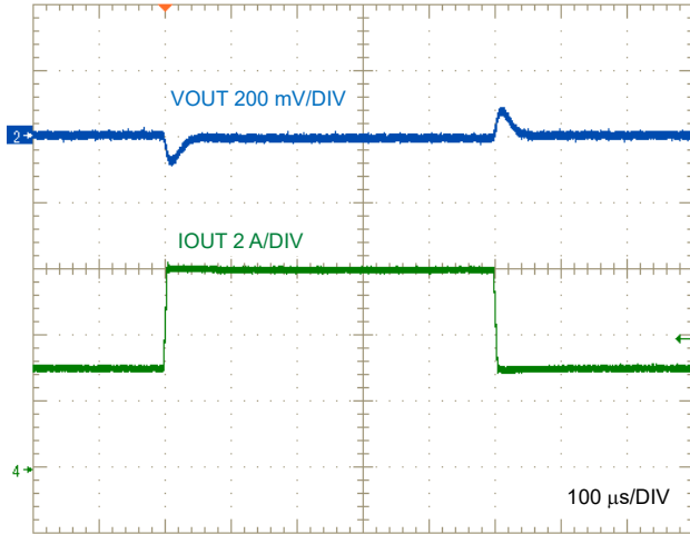
8-26. LM634x0-Q1 Load Transient, I_{OUT} = 3A to 6A
