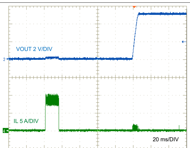
Figure 8-11. Short-Circuit Recovery
