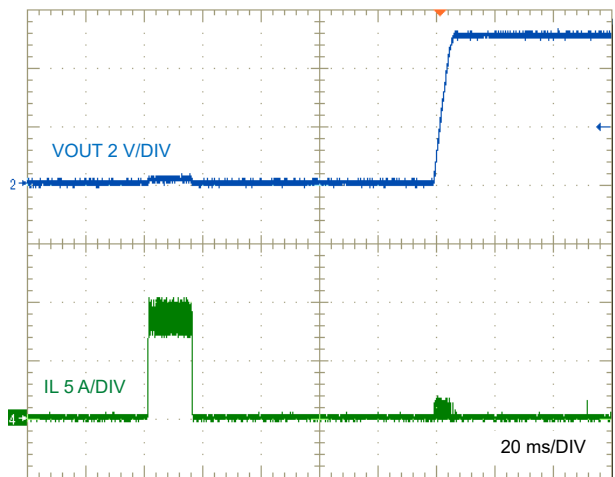
図 8-10. LM634x0-Q1 Short-Circuit Recovery to No Load
