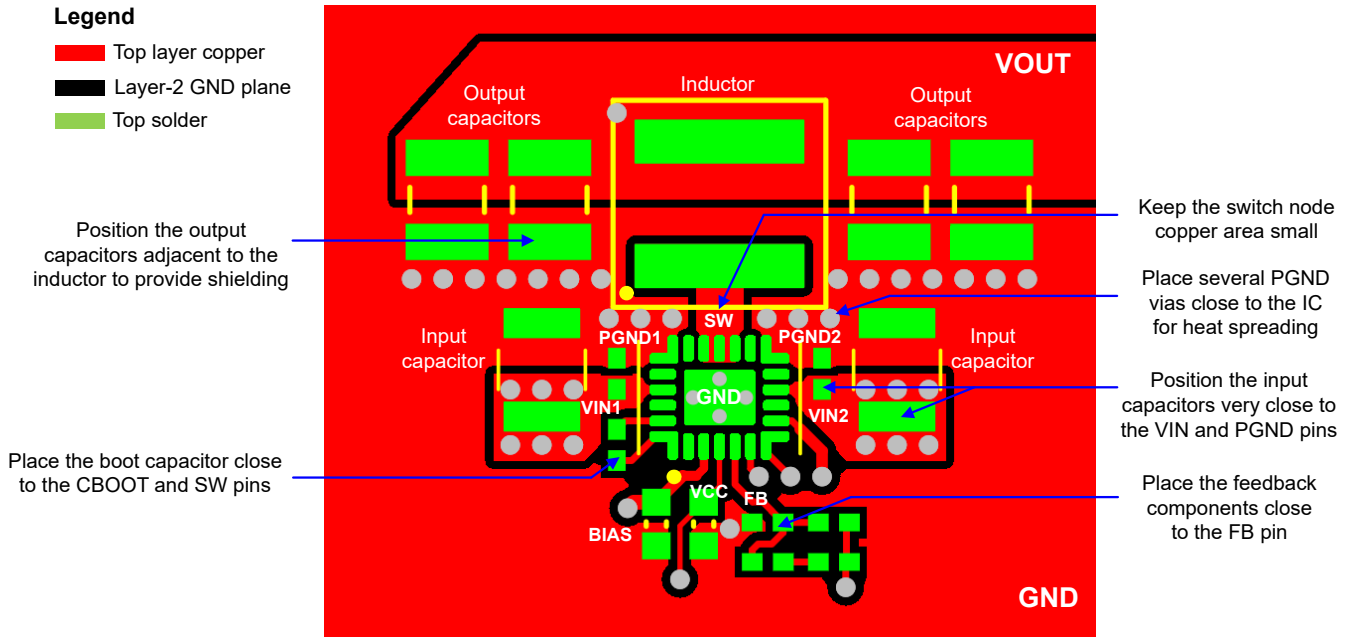
9-30. PCB Layout Example
