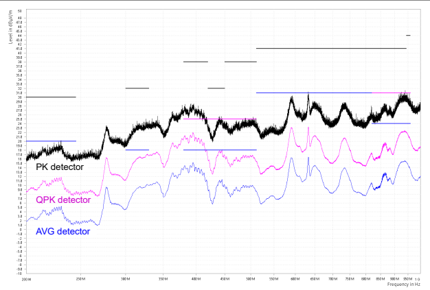
8-20. CISPR 25 Class 5 Radiated EMI, Log Antenna, Vertical Polarization, 200MHz to 1GHz
