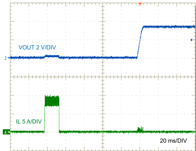
8-29. LM634x0-Q1 Short-Circuit Recovery to No Load
