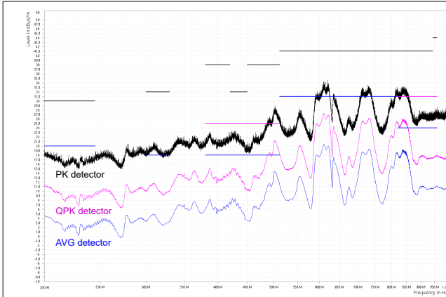
9-18. CISPR 25 Class 5 Radiated EMI, Log Antenna, Horizontal Polarization, 200 MHz to 1 GHz
