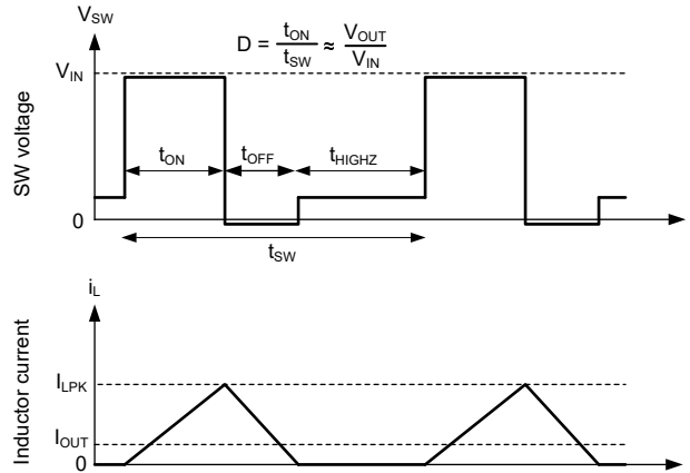
8-13. PFM Mode Operation at Light Loads
