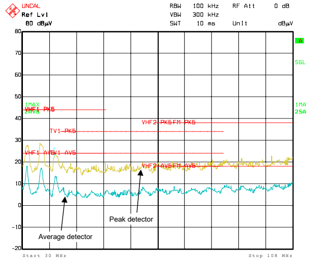
9-15. CISPR 25 Class 5 Conducted EMI, 30 MHz to 108 MHz
