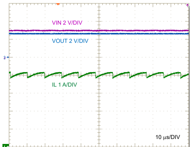
8-12. LM634x0-Q1 Frequency Foldback in Dropout, V_{IN} = 3V
