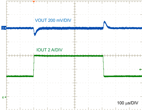
8-7. LM634x0-Q1 Load Transient, I_{OUT} = 3A to 6A
