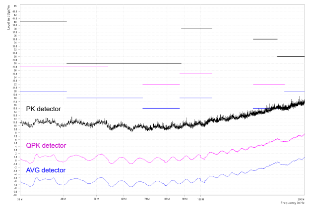
9-17. CISPR 25 Class 5 Radiated EMI, Bicon Antenna, Vertical Polarization, 30 MHz to 200 MHz
