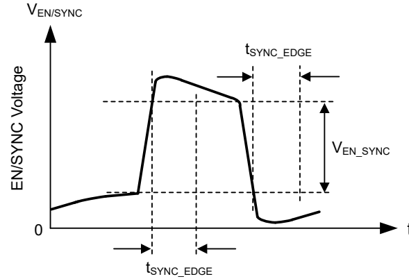
図 8-2. Typical Synchronization Waveform Applied to EN/SYNC
