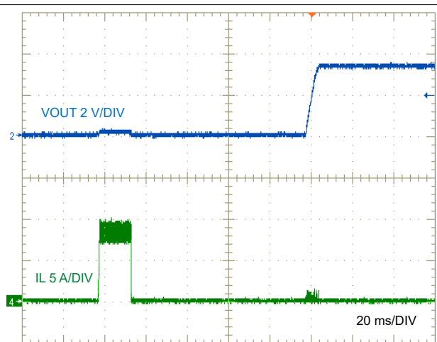
図 9-28. LM63460-Q1 Short Circuit Recovery to No Load
