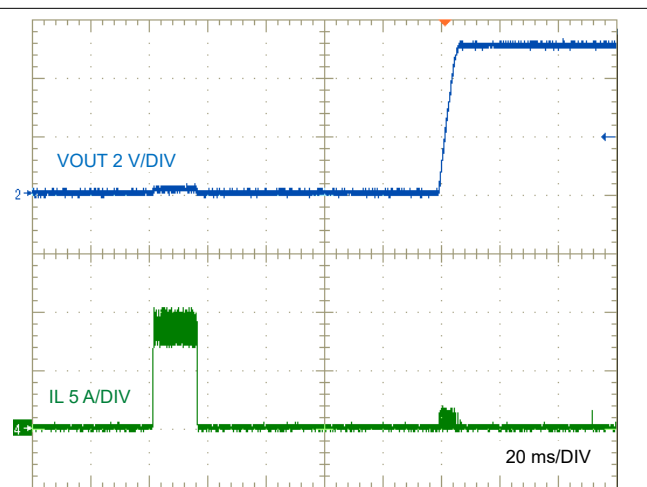
Figure 7-11. Short-Circuit Recovery
