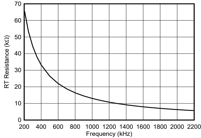
図 8-4. Setting the Switching Frequency
