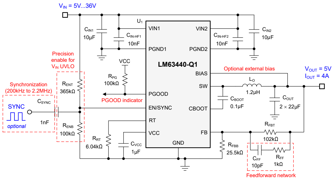
図 8-2. Application Circuit 2 – 5V, 4A at 2.1MHz
