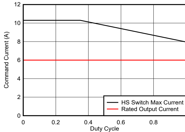
図 8-8. HS Switch Maximum Current as a Function of Duty Cycle for the LM63460-Q1
