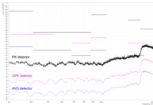
9-16. CISPR 25 Class 5 Radiated EMI, Bicon Antenna, Horizontal Polarization, 30 MHz to 200 MHz
