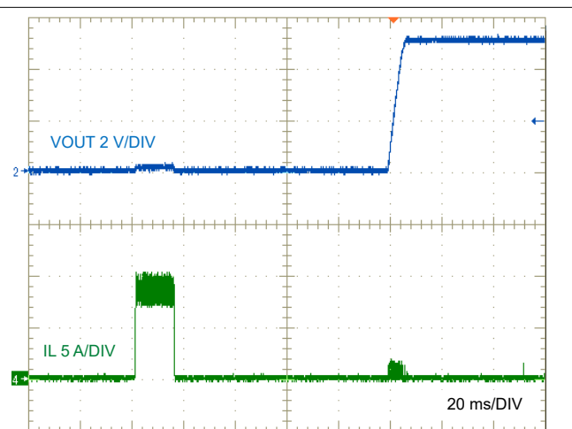
Figure 7-11. Short-Circuit Recovery
