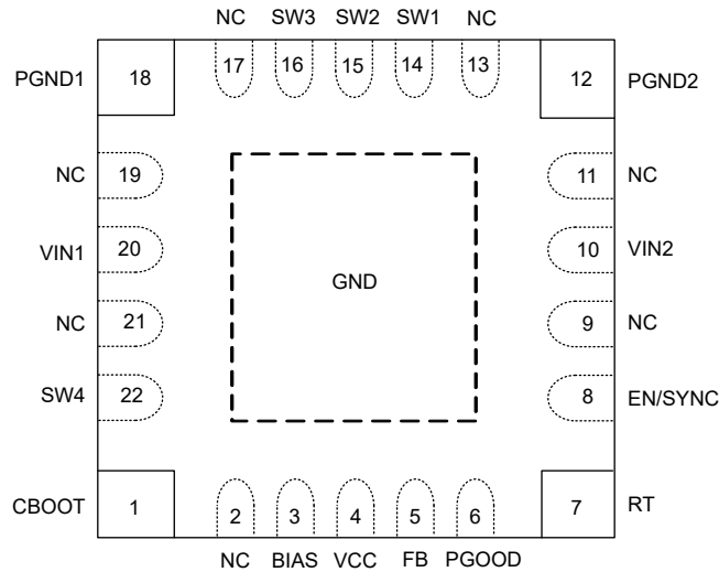
図 5-1. 22-Pin Enhanced HotRod™ QFN RYF Package (Top View)
