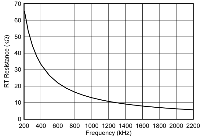
図 7-4. Setting the Switching Frequency
