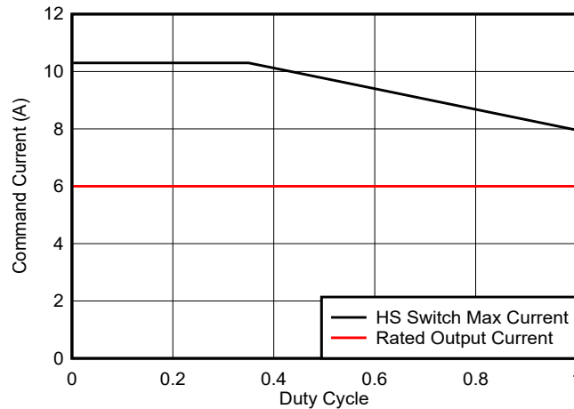
図 7-8. HS Switch Maximum Current as a Function of Duty Cycle for the LM63460-Q1
