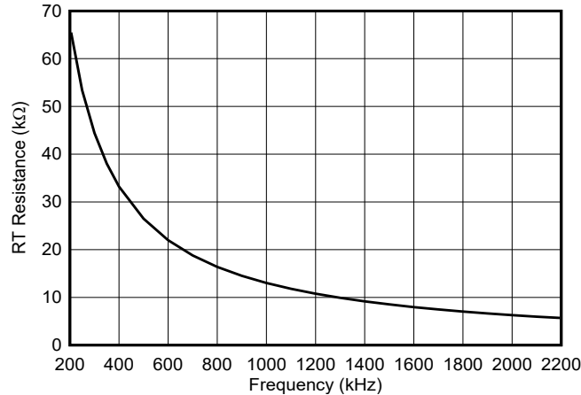
図 7-4. Setting the Switching Frequency
