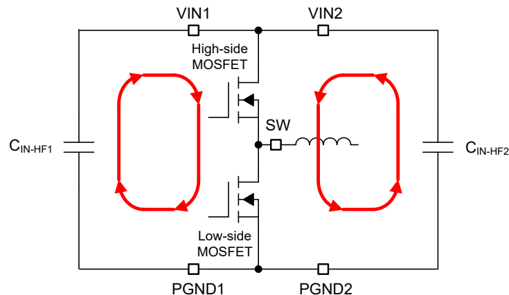
Figure 9-29. Input Current Loops
