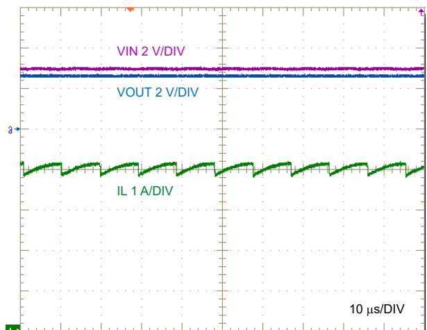
図 9-11. LM63460-Q1 Frequency Foldback in Dropout, V_{IN} = 3\text{ V}
