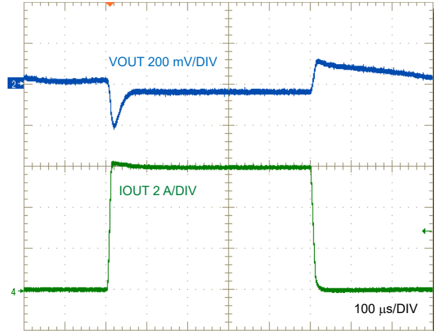
8-27. LM634x0-Q1 Load Transient, I_{OUT} = 0A \text{ to } 6A
