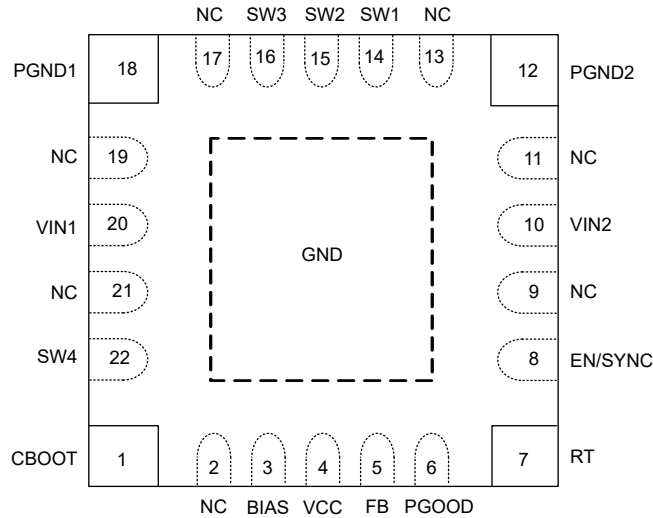
図 6-1. 22-Pin Enhanced HotRod™ QFN RYF Package (Top View)
