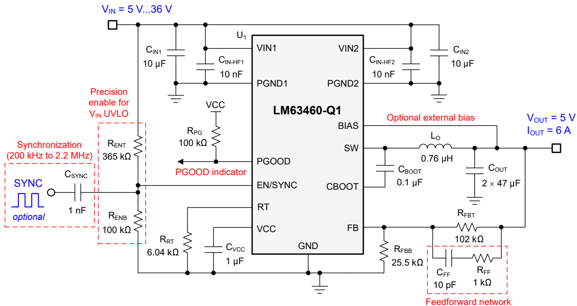
図 8-1. Application Circuit 1 – 5V, 6A at 2.1MHz
