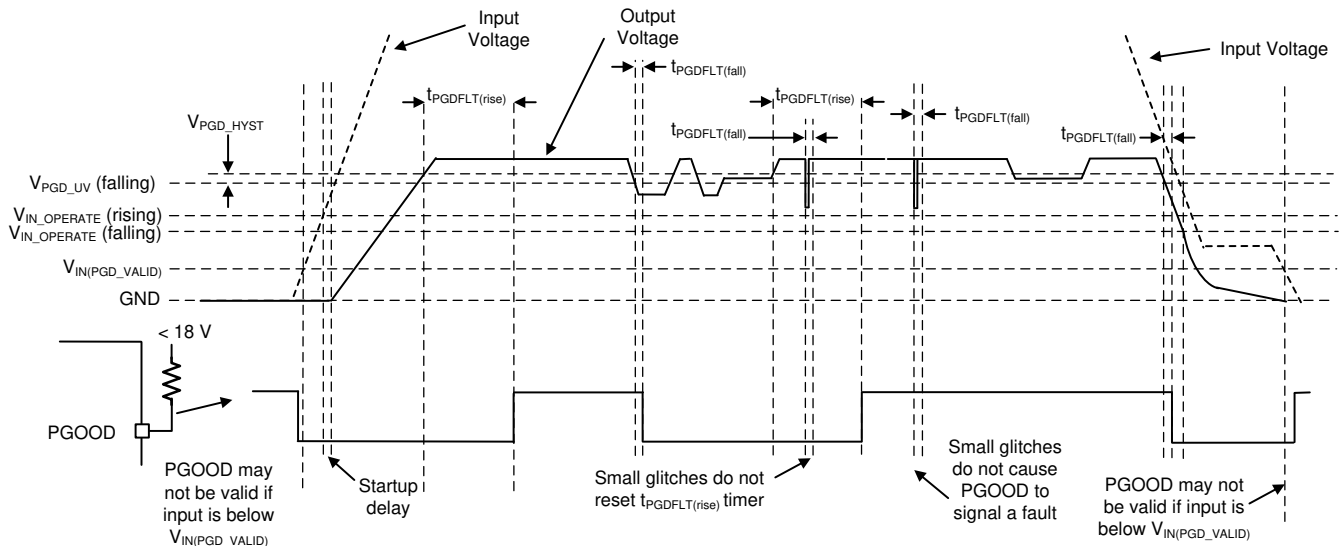
図 7-5. PGOOD Timing Diagram (Excludes OV Events)
