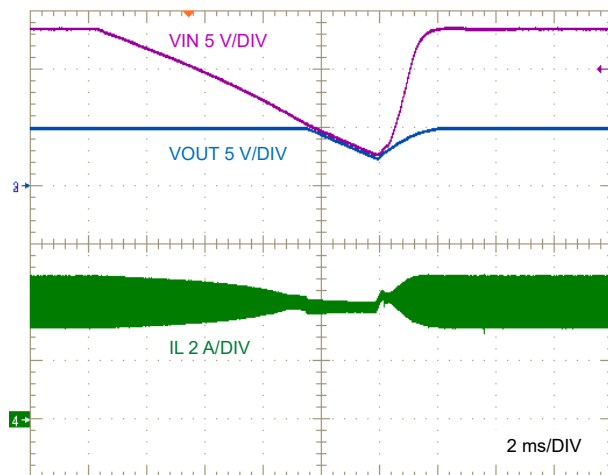
図 9-10. LM63460-Q1 Line Transient and Recovery from Dropout
