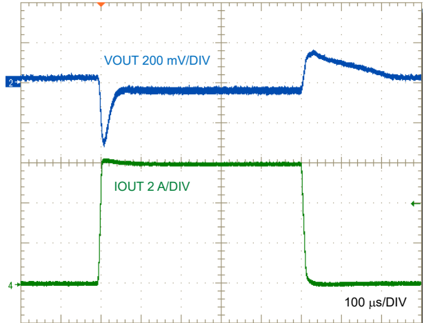
図 8-8. LM634x0-Q1 Load Transient, I_{OUT} = 0A to 6A
