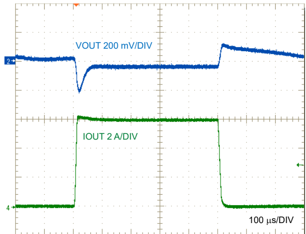
図 9-26. LM63460-Q1 Load Transient, I_{OUT} = 0 \text{ A to } 6 \text{ A}
