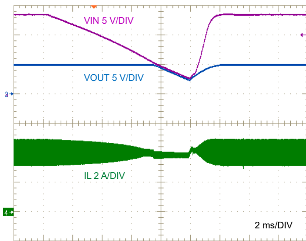
図 8-11. LM634x0-Q1 Line Transient and Recovery from Dropout
