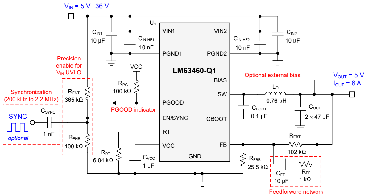
図 9-1. Application Circuit 1 – 5 V, 6 A at 2.1 MHz
