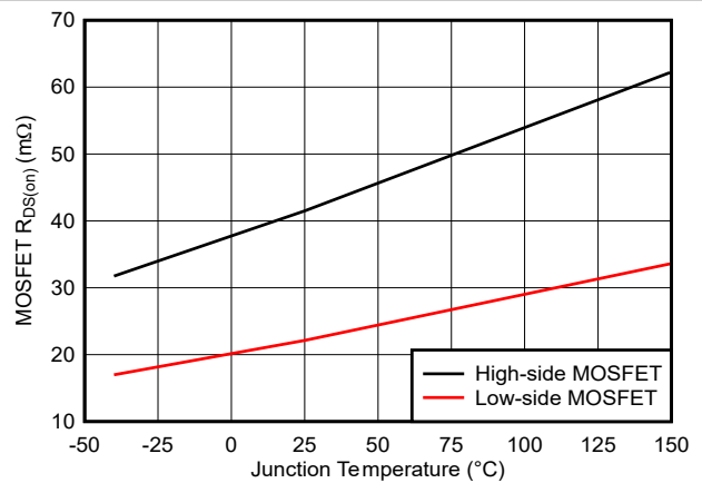
6-6. High-Side and Low-Side MOSFET R_{DS(on)}
