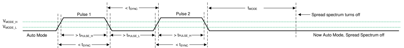
図 7-7. Spread Spectrum Disabled in AUTO Mode
