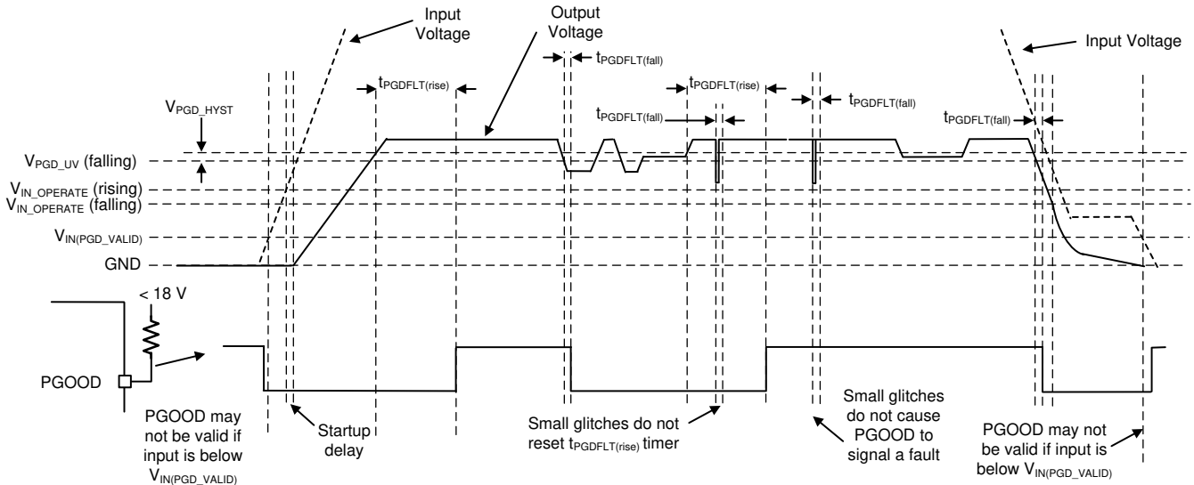
7-13. PGOOD Timing Diagram (Excludes OV Events)
