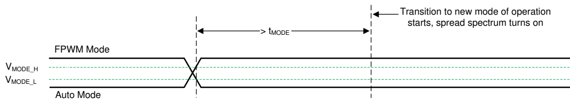
図 7-5. Transition from AUTO Mode and FPWM Mode
