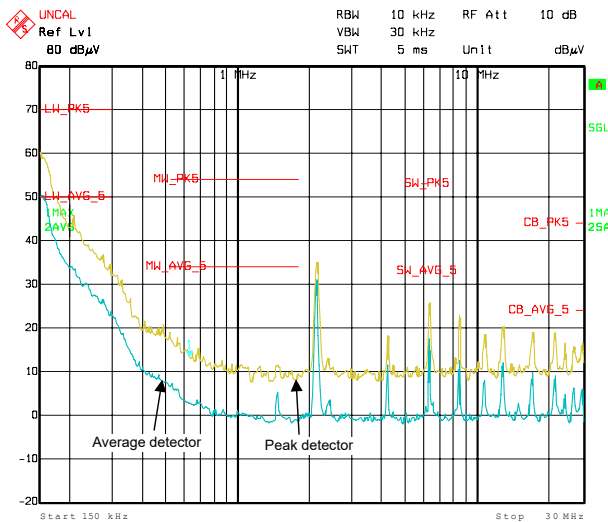
8-15. CISPR 25 Class 5 Conducted EMI, 150kHz to 30MHz
