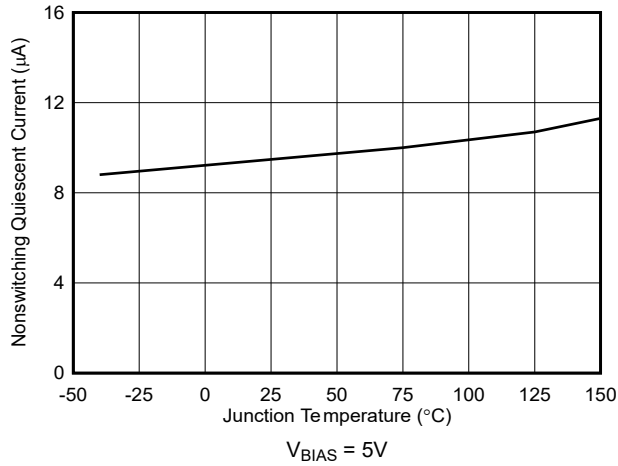
6-1. Non-Switching Input Supply Current
