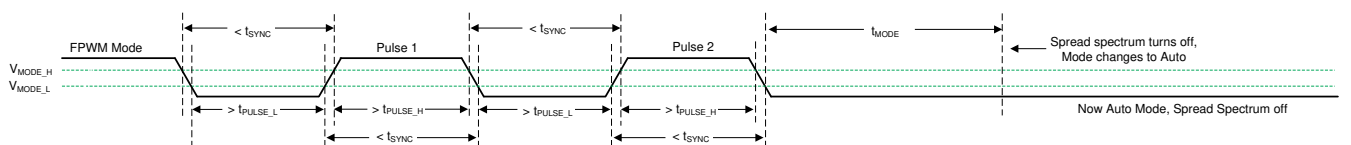
図 7-8. Spread Spectrum Disabled in Transition from FPWM Mode to AUTO Mode
