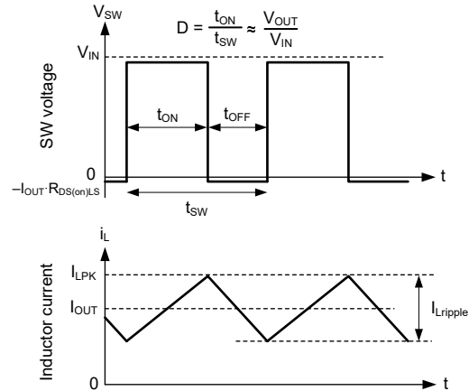
図 7-20. SW Voltage and Inductor Current Waveforms in Continuous Conduction Mode (CCM)
