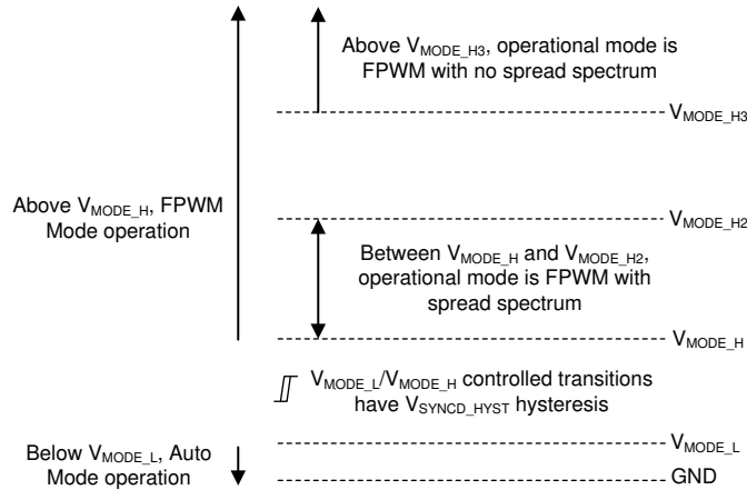
図 7-2. Level-Dependent Mode Selection Settings
