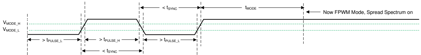
Figure 7-11. Transition from SYNC Mode to FPWM Mode
