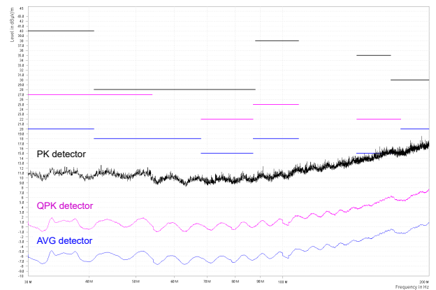
8-18. CISPR 25 Class 5 Radiated EMI, Bicon Antenna, Vertical Polarization, 30MHz to 200MHz
