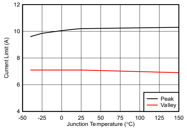
6-4. High-Side and Low-Side Current Limits
