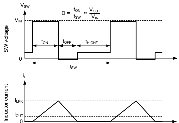
図 7-21. PFM Mode Operation at Light Loads
