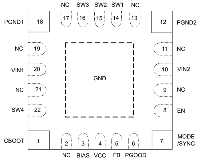
図 5-1. 22-Pin Enhanced HotRod™ VQFN-FCRLF RYF Package (Top View)
