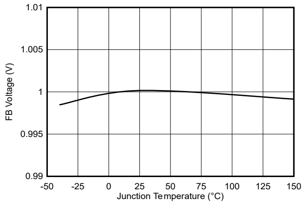
6-3. Feedback Voltage
