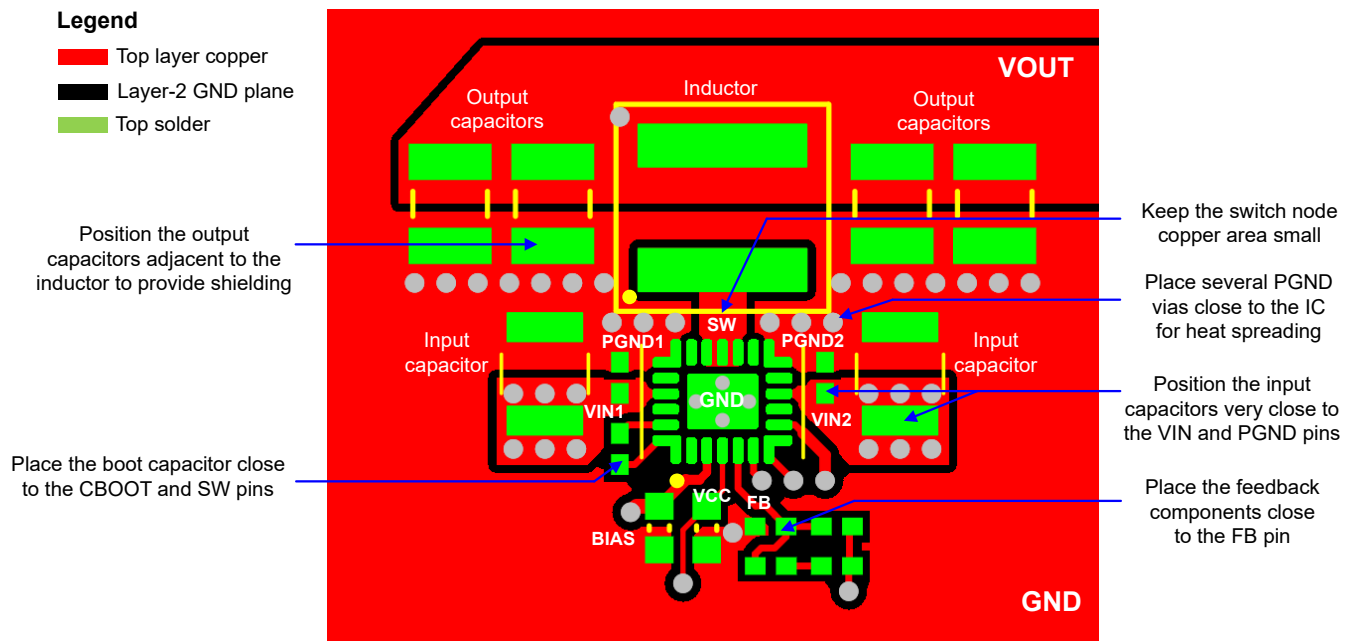
8-22. PCB Layout Example
