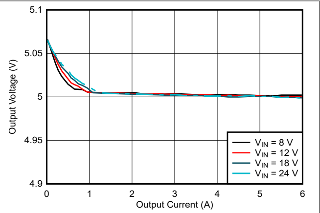
图 8-4. LM644x0-Q1 Load and Line Regulation
