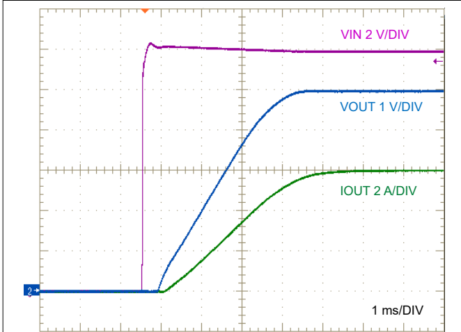
图 8-5. LM644x0-Q1 Start-Up, 6A Resistive Load
