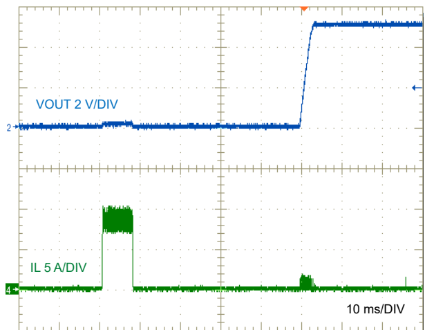
図 8-10. LM644x0-Q1 Short-Circuit Recovery to No Load
