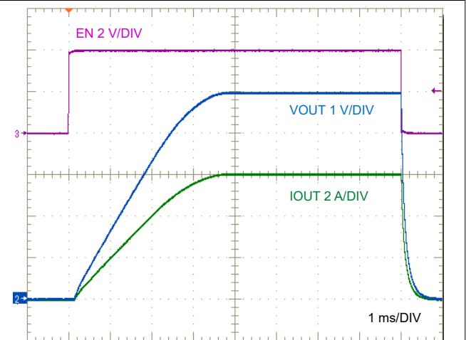
图 8-6. LM644x0-Q1 Enable On and Off, 6A Resistive Load
