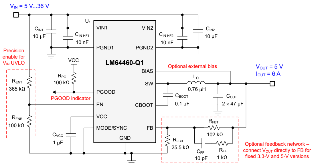
図 8-1. Application Circuit 1 – 5V, 6A at 2.1MHz
