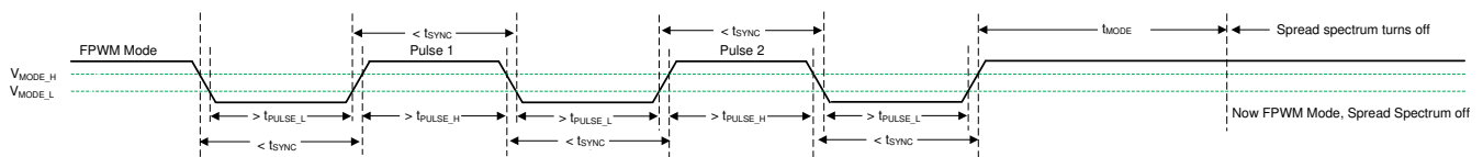
図 7-6. Spread Spectrum Disabled in FPWM Mode
