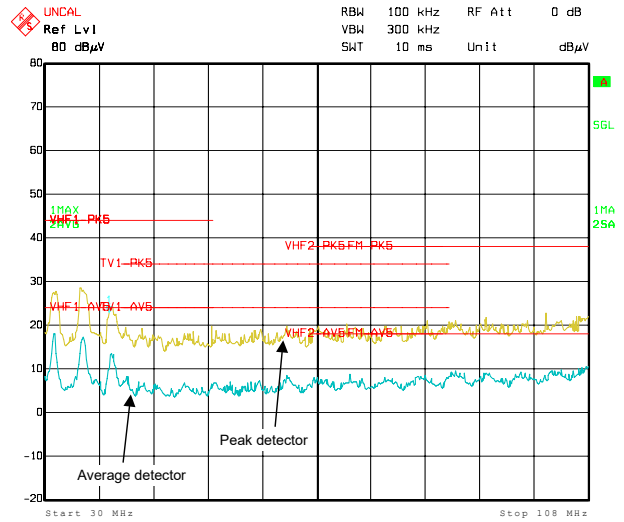
8-16. CISPR 25 Class 5 Conducted EMI, 30MHz to 108MHz
