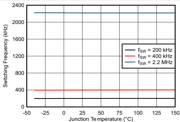
6-5. Switching Frequency Set by SYNC
