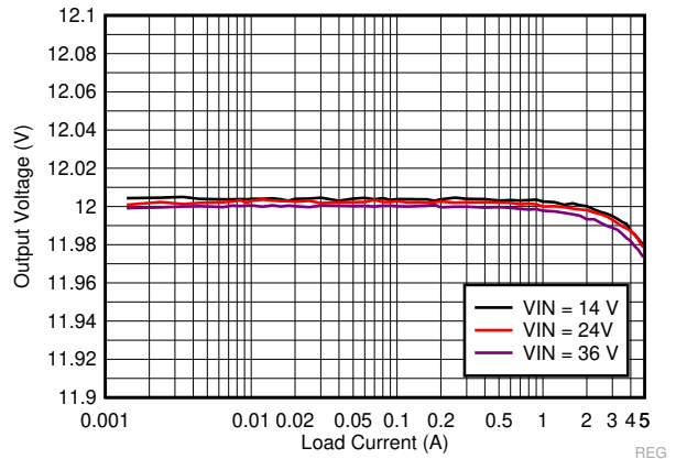
9-34. LM73605-Q1 Load and Line Regulation
