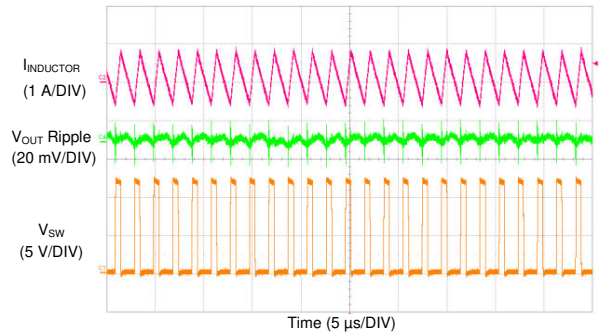
9-46. LM73606-Q1 Switching Waveform and V_{OUT} Ripple
