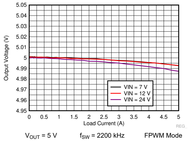
9-26. LM73605-Q1 Load and Line Regulation
