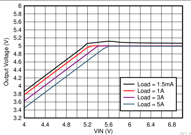
9-35. LM73606-Q1 Dropout Curve
