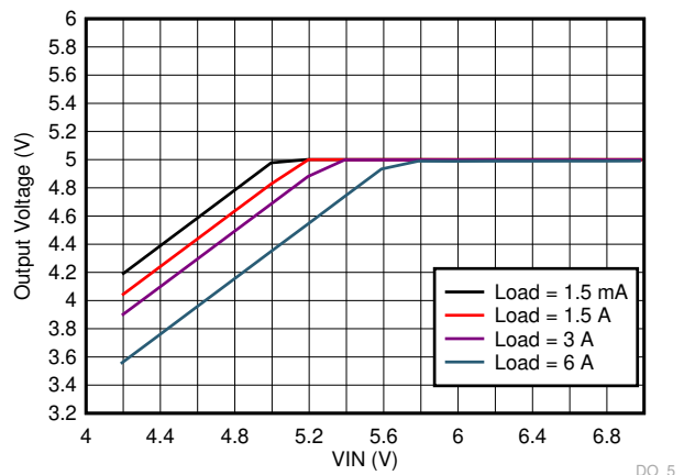
9-34. LM73605-Q1 Load and Line Regulation
