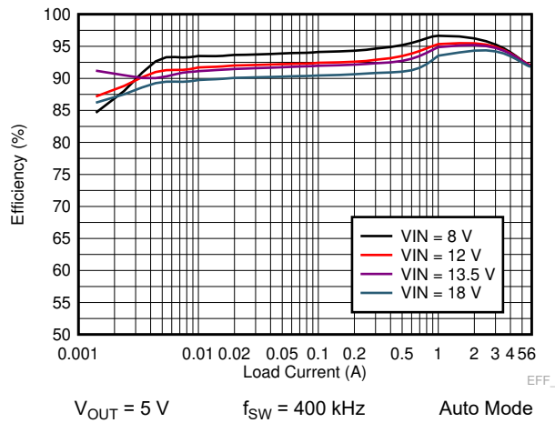
9-11. LM73606-Q1 Efficiency
