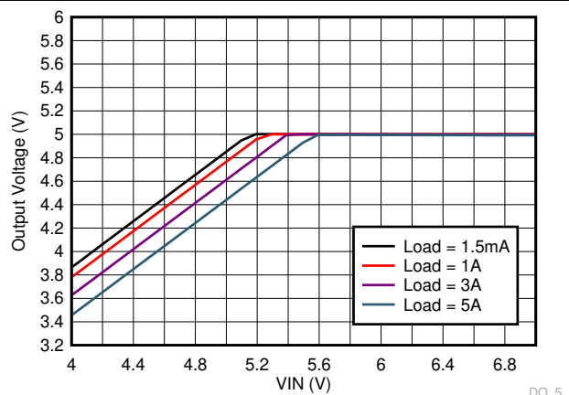
9-36. LM73606-Q1 Dropout Curve
