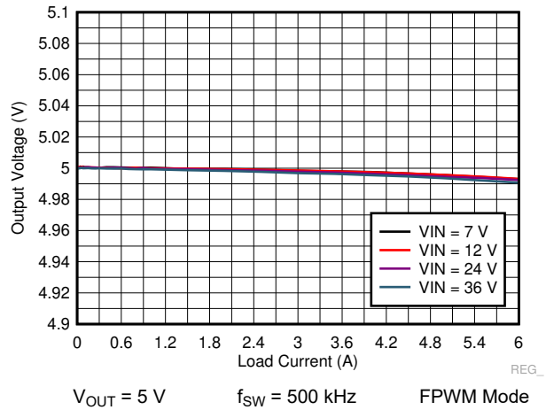
9-24. LM73606-Q1 Load and Line Regulation
