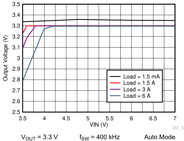
9-41. LM73606-Q1 Dropout Curve
