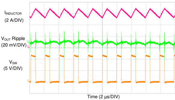
9-47. LM73606-Q1 Switching Waveform and V_{OUT} Ripple
