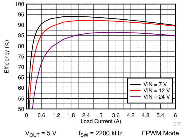
9-18. LM73606-Q1 Efficiency
