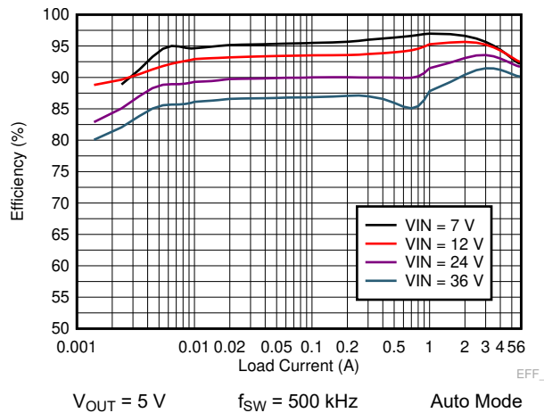
9-13. LM73606-Q1 Efficiency
