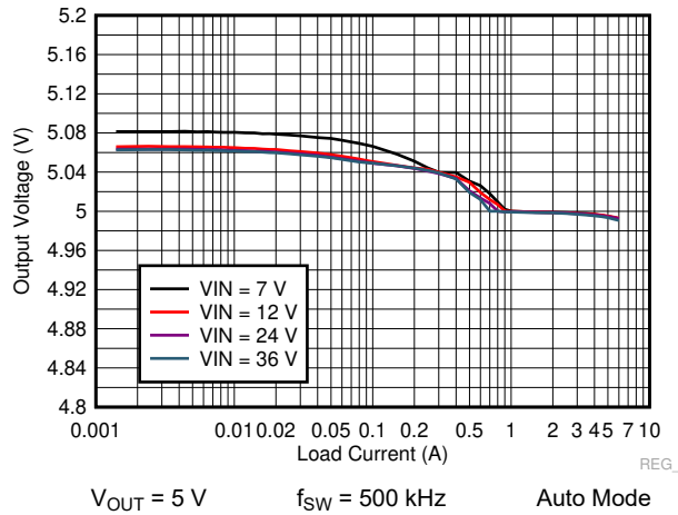
9-23. LM73606-Q1 Load and Line Regulation
