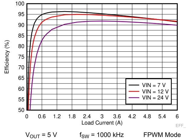
9-16. LM73606-Q1 Efficiency
