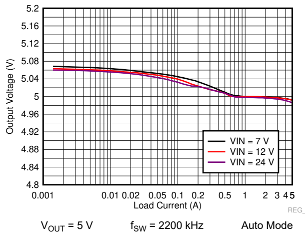
9-25. LM73605-Q1 Load and Line Regulation
