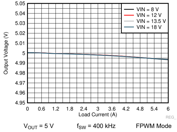
9-22. LM73606-Q1 Load and Line Regulation
