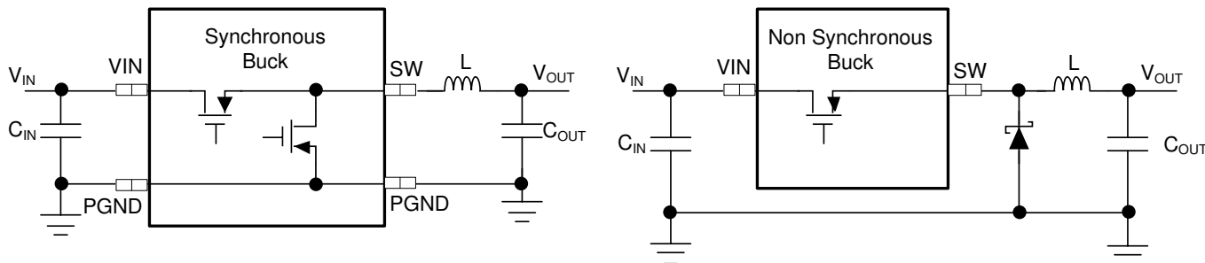
8-1. Simplified Synchronous versus Non-synchronous Buck Converters
