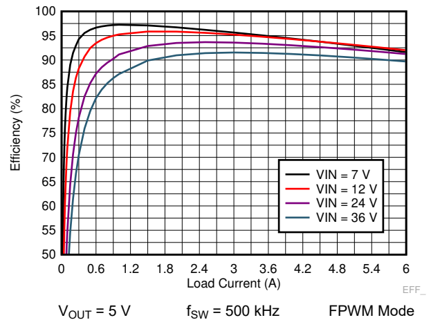
9-14. LM73606-Q1 Efficiency
