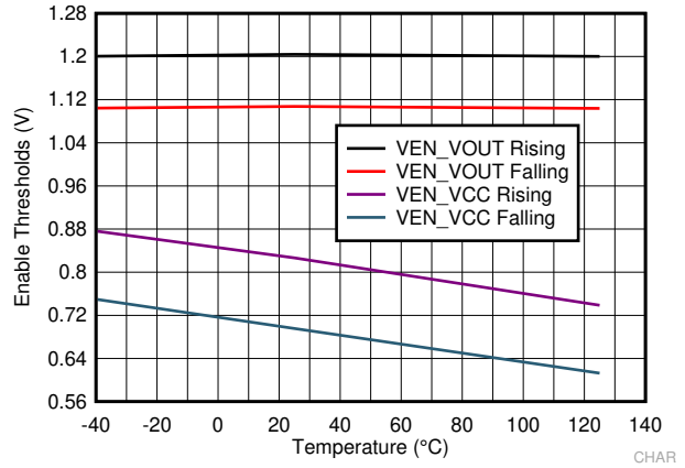
7-8. Enable Thresholds
