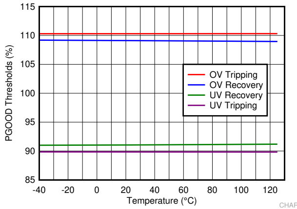
7-9. PGOOD Thresholds
