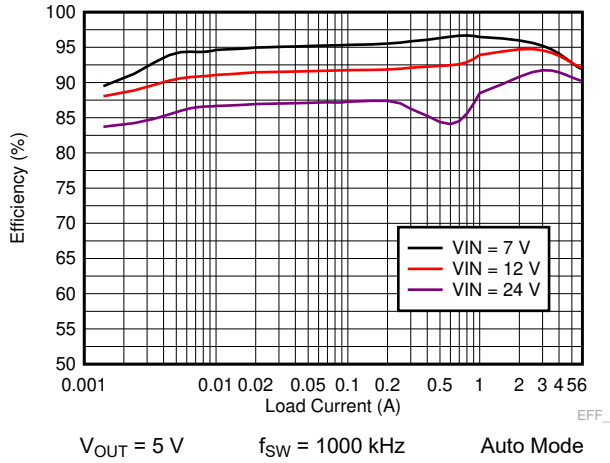
9-15. LM73606-Q1 Efficiency
