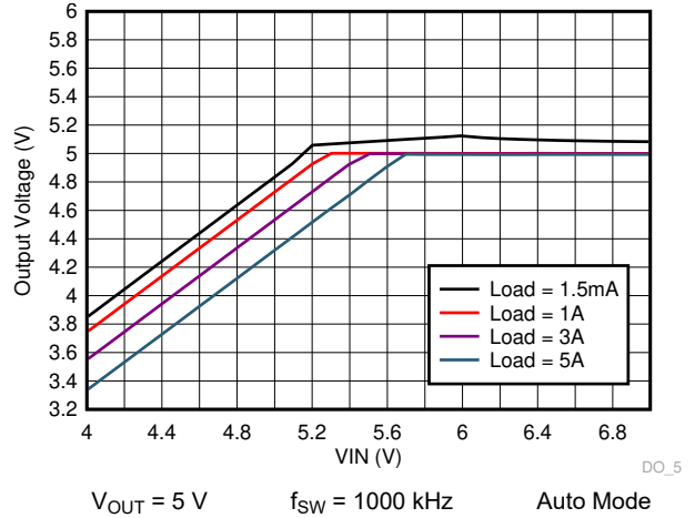
9-40. LM73605-Q1 Dropout Curve
