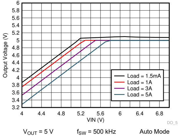
9-39. LM73605-Q1 Dropout Curve
