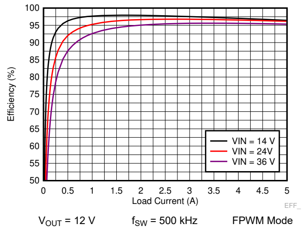
9-20. LM73605-Q1 Efficiency
