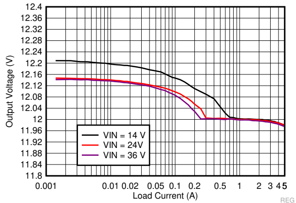
9-33. LM73605-Q1 Load and Line Regulation
