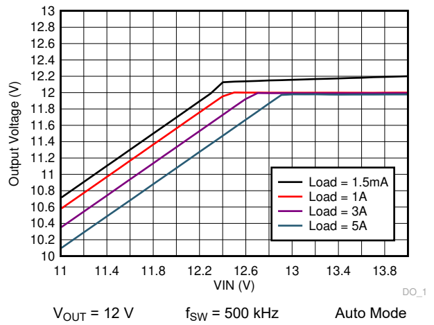
9-44. LM73605-Q1 Dropout Curve
