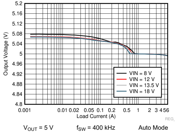
9-21. LM73606-Q1 Load and Line Regulation
