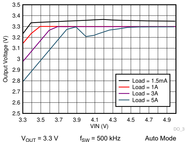
9-43. LM73605-Q1 Dropout Curve
