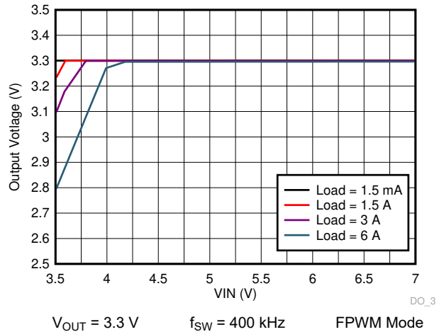
9-42. LM73606-Q1 Dropout Curve
