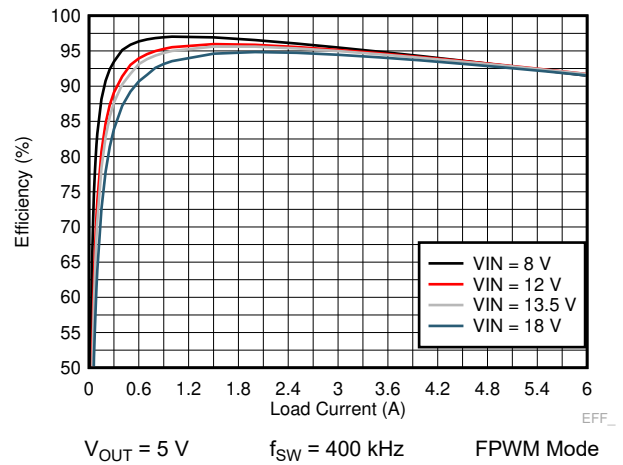
9-12. LM73606-Q1 Efficiency
