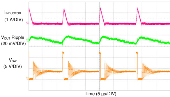
9-45. LM73606-Q1 Switching Waveform and V_{OUT} Ripple
