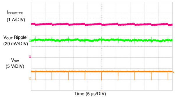
9-48. LM73606-Q1 Switching Waveform and V_{OUT} Ripple
