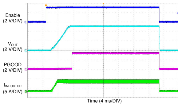
8-18. LM76005 Start-up Waveform
