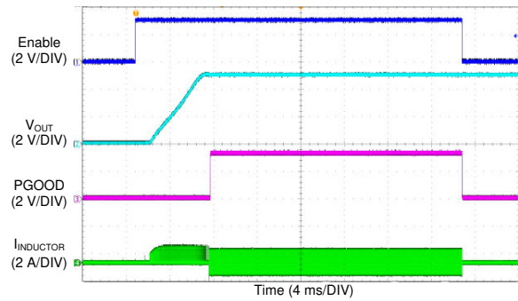
8-17. LM76005 Start-up Waveform
