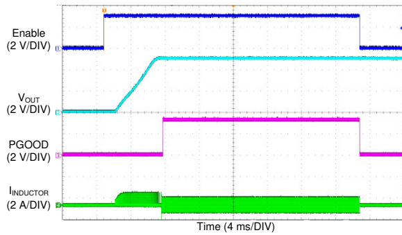
8-16. LM76005 Start-up Waveform
