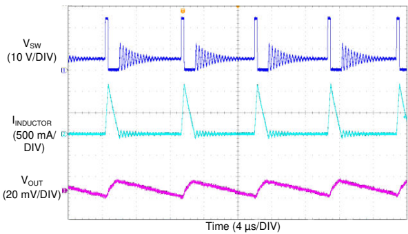
8-11. LM76005 Switching Waveform and Output Ripple
