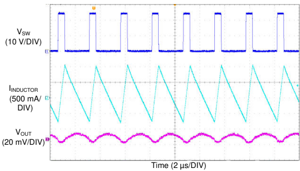
8-13. LM76005 Switching Waveform and Output Ripple
