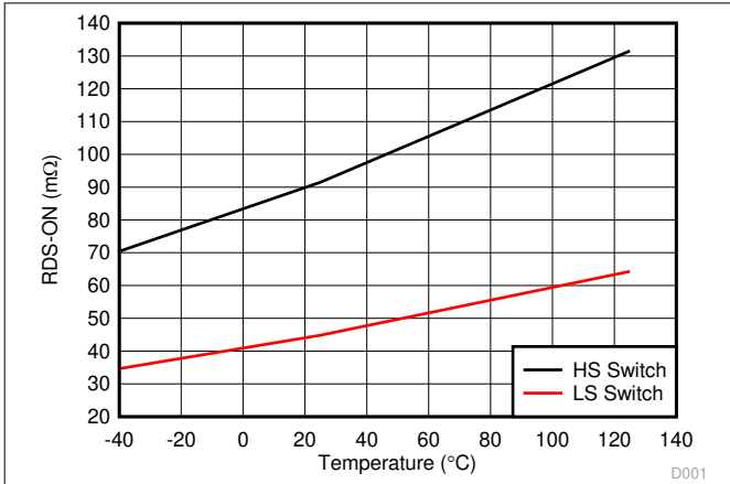
6-1. High-Side and Low-Side Switch R_{DS-ON}
