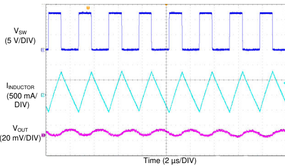
8-12. LM76005 Switching Waveform and Output Ripple
