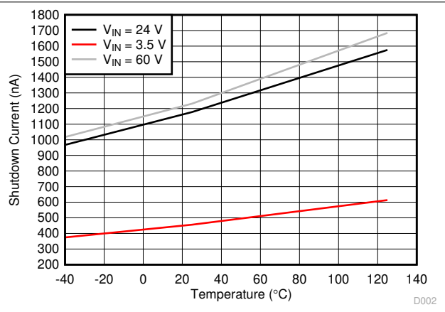
6-2. Shutdown Quiescent Current
