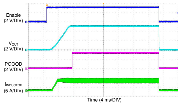
8-19. LM76005 Start-up Waveform
