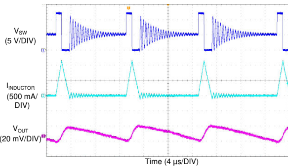
8-10. LM76005 Switching Waveform and Output Ripple
