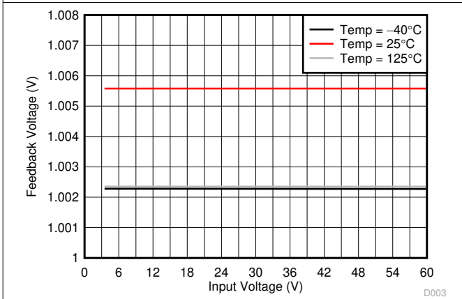
6-3. Feedback Voltage
