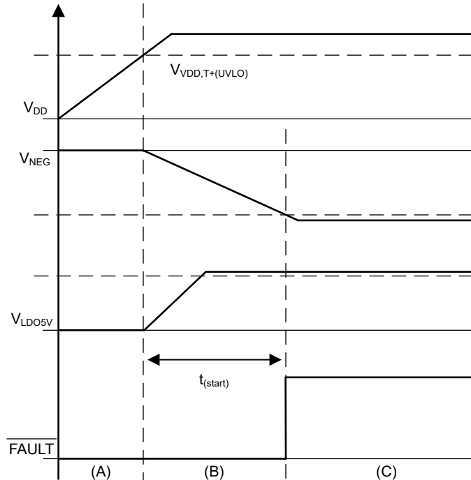
☒ 9-8. Start Up Timing Diagram
