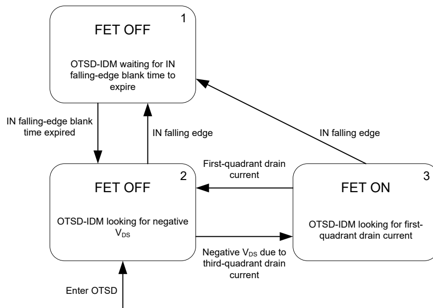
Figure 9-7. Overtemperature-Shutdown Ideal-Diode Mode (OTSD-IDM) State Machine
