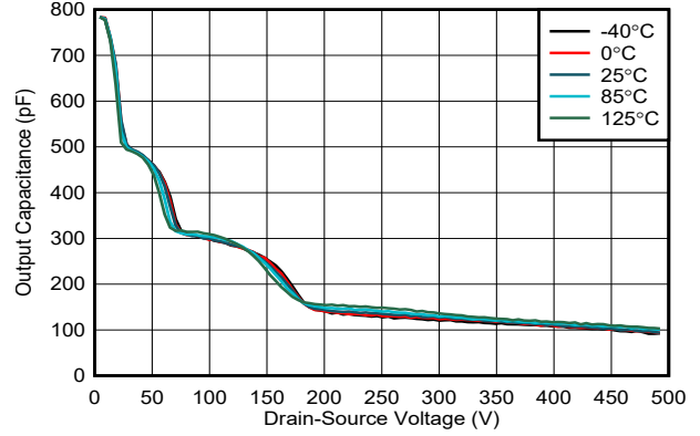
7-8. Output Capacitance vs Drain-Source Voltage
