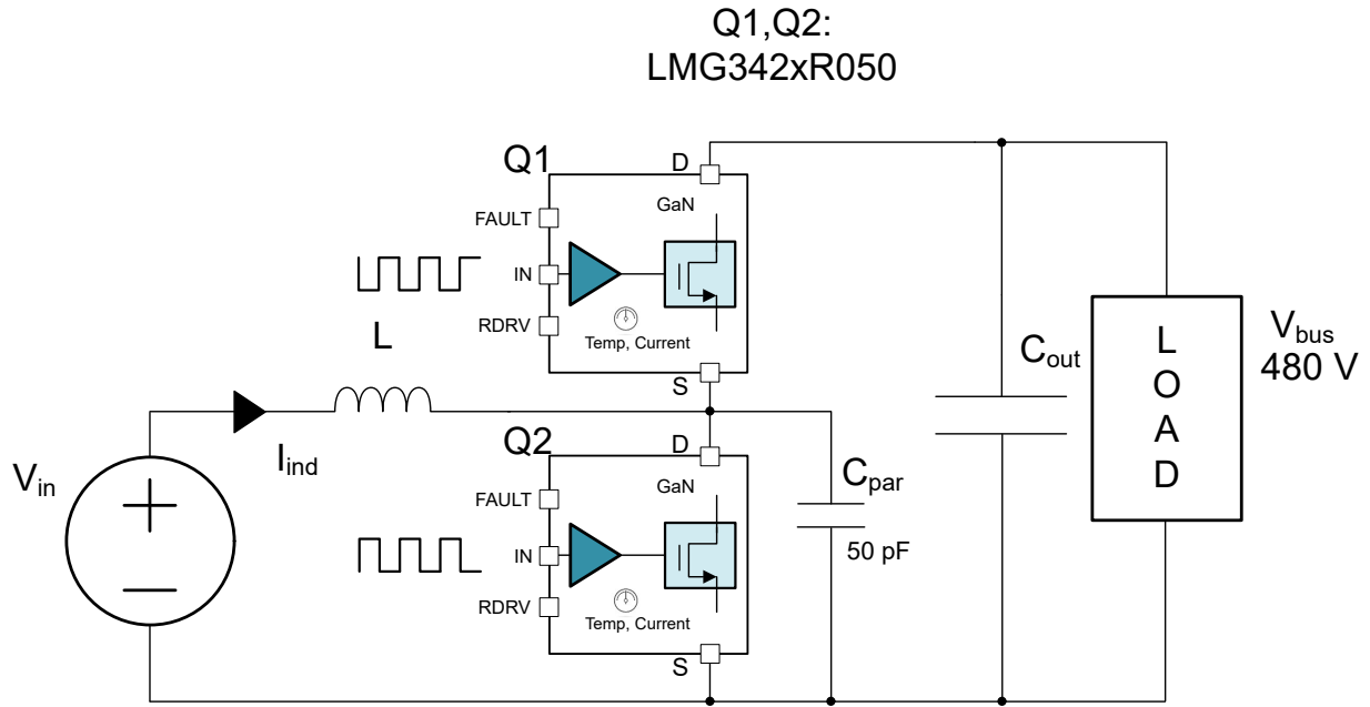
9-9. Circuit Used for SOA Curve
