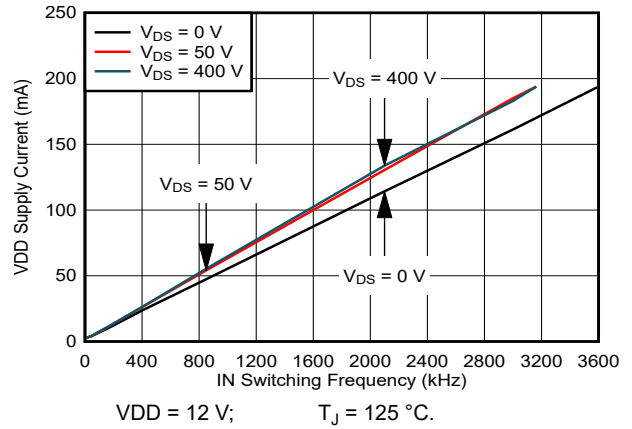
7-10. VDD Supply Current vs IN Switching Frequency
