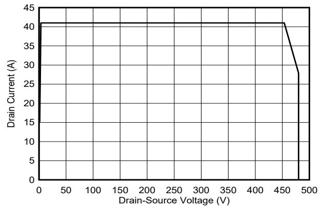
7-12. Repetitive Safe Operation Area
