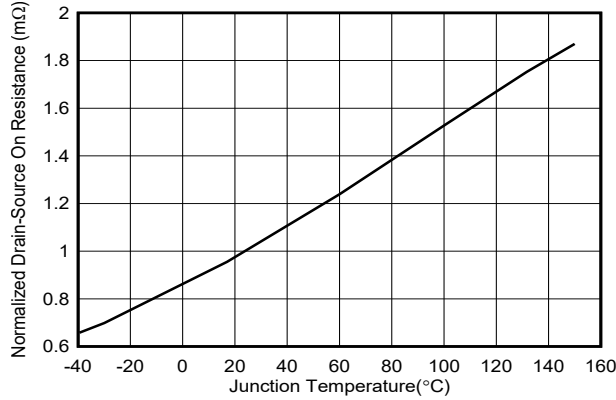
7-7. Normalized On-Resistance vs Junction Temperature
