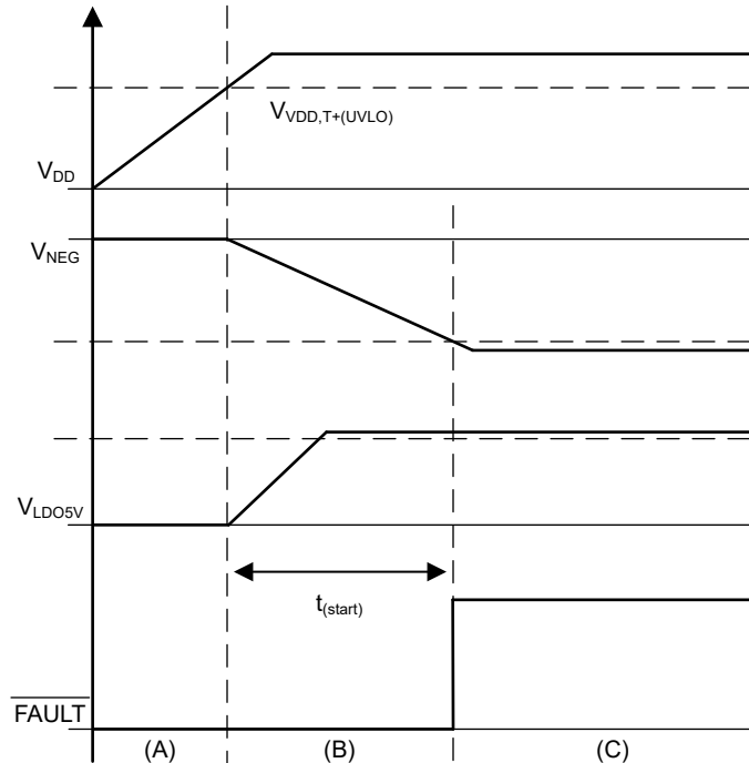
Figure 9-8. Start Up Timing Diagram
