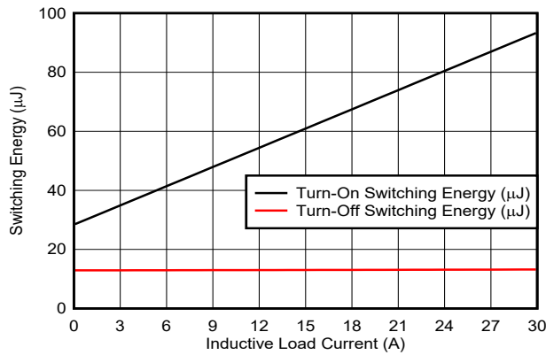
7-11. Half-Bridge Switching Energy vs Inductive Load Current
