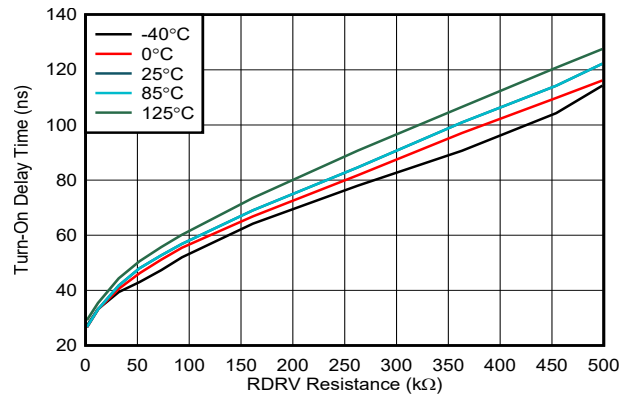
7-2. Turn-On Delay Time vs Drive Strength Resistance
