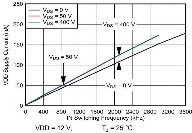
7-9. VDD Supply Current vs IN Switching Frequency
