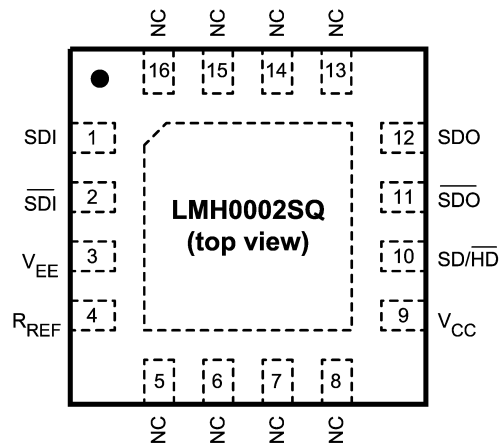
16-Pin LLP Order Number LMH0002SQ See NS Package Number SQB16A
