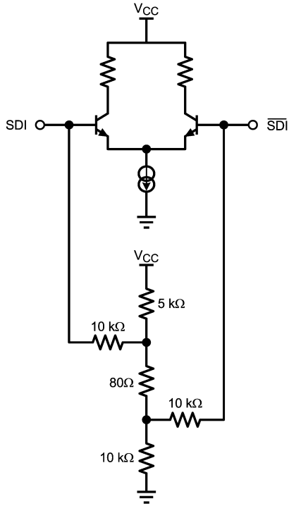
FIGURE 1. Differential Input Stage for SDI and \overline{\text{SDI}} .
