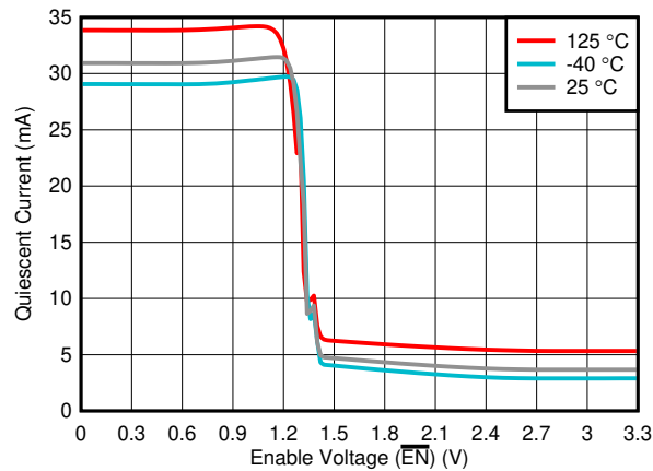
Logic switching demonstrated using \overline{EN} pin. \overline{IDC\_EN} and gain pins behave similarly.
