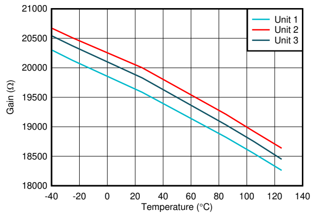
Gain = 20 kΩ
