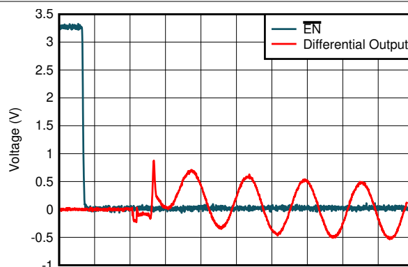
Time (25 ns/div) Gain = 20 k \Omega
