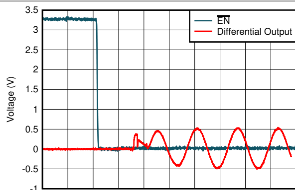
Time (25 ns/div) Gain = 2 k \Omega
