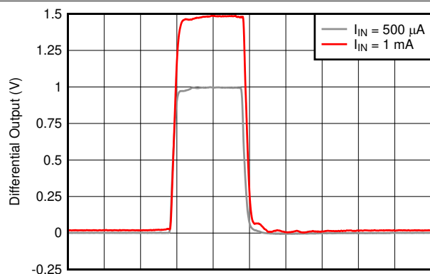
Time (5 ns/div) Gain = 2 k \Omega
