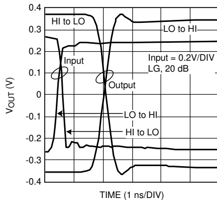
5-37. Step Response
