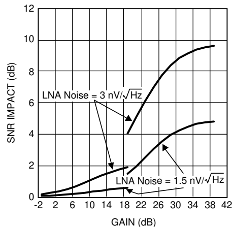
Figure 7-13. LNA Buffer SNR Impact
