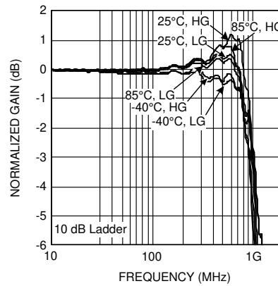
5-8. Response Over Temperature
