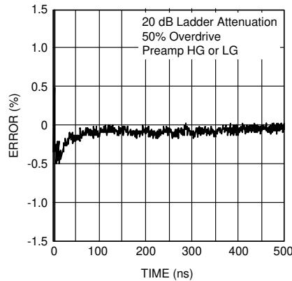
5-53. Overdrive Recovery Time (Return to Zero)
