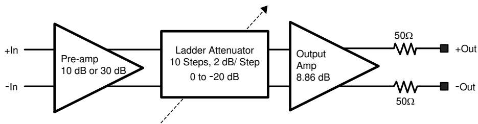
☒ 7-2. LMH6518 Signal Path Block Diagram
