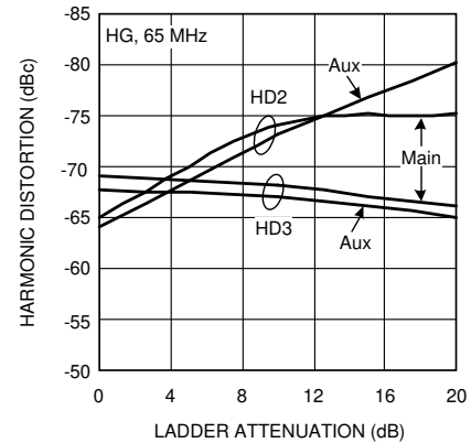
Figure 5-26. Main and Auxiliary Distortion Comparison
