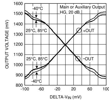
5-50. Output vs Input
