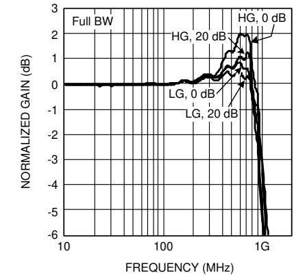
Figure 5-4. Small Signal Response (LG, 0-dB)
