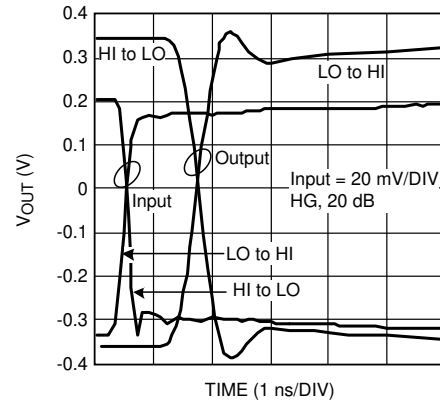
5-38. Step Response
