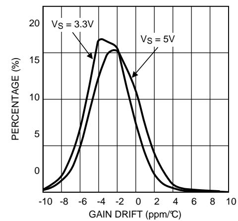
Figure 46. Gain Error Distribution at V_S = 5\text{ V} , 5000 Parts LMP8603 and LMP8603-Q1
