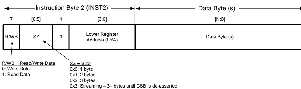
Figure 55. Register Read/Write Protocol
