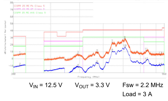
8-23. CISPR 25 Class 5 Radiated EMI, Log Antenna, Horizontal Polarization, 300 MHz - 960 MHz Orange: Peak Detect, Blue: Average Detect
