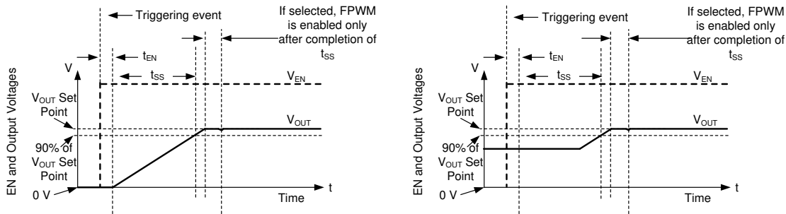
7-9. Soft Start With and Without Prebias Voltage
