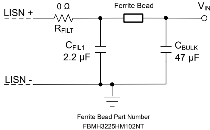
8-25. Typical Input EMI Filter
