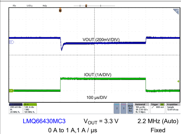
8-13. Load Transient
