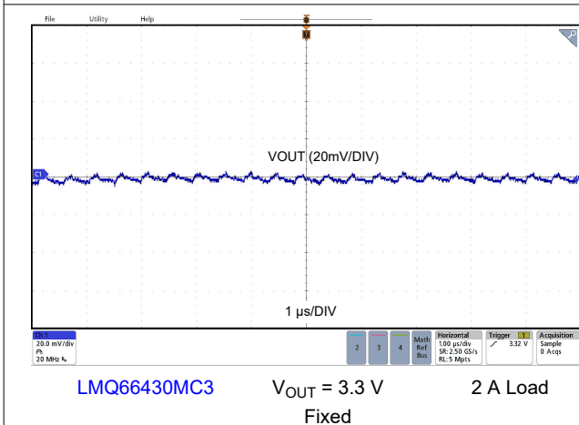
8-14. Output Voltage Ripple
