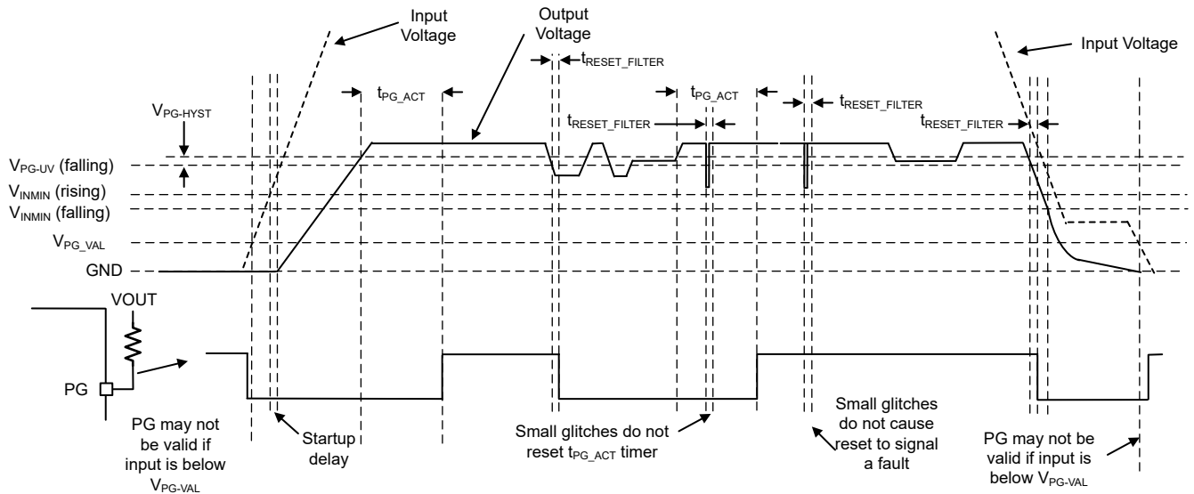
图 7-7. Power-Good Operation (OV Events Not Included)
