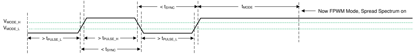
图 7-6. Transition from SYNC Mode to FPWM Mode
