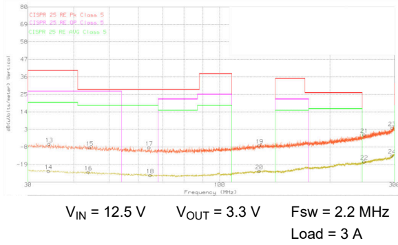
8-22. CISPR 25 Class 5 Radiated EMI, Biconical Antenna, Vertical Polarization, 30 MHz - 300 MHz Orange: Peak Detect, Yellow: Average Detect
