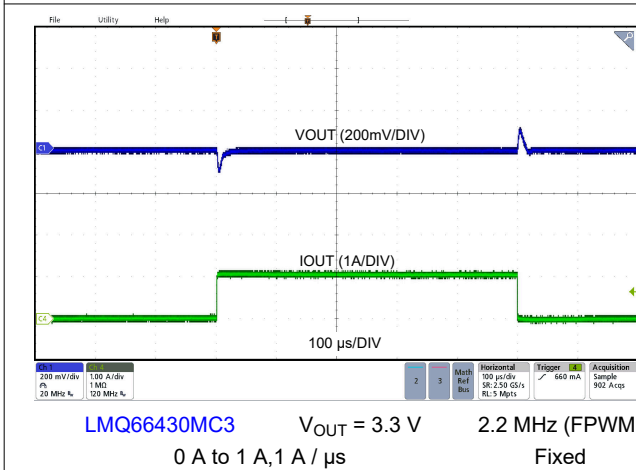
8-12. Load Transient
