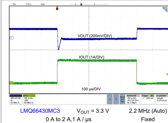
8-10. Load Transient
