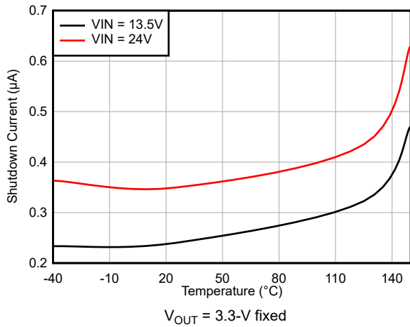
6-1. Shutdown Current Versus Temperature
