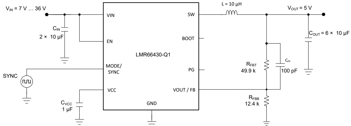
図 8-26. Application Circuit 2 - 5 V (adjustable), 3 A, 400 kHz
