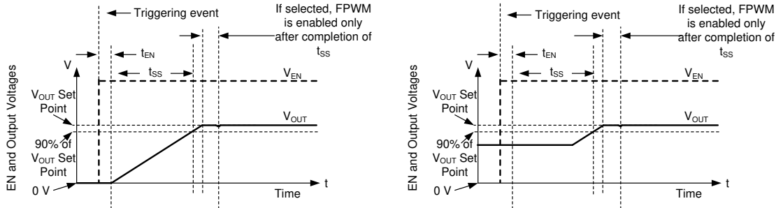
7-9. Soft Start With and Without Prebias Voltage
