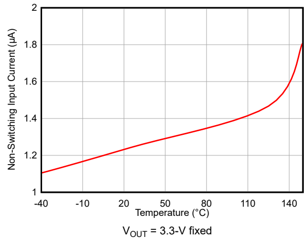
6-2. Non-Switching Input Current ( I_{QVIN(nonsw)} ) Versus Temperature
