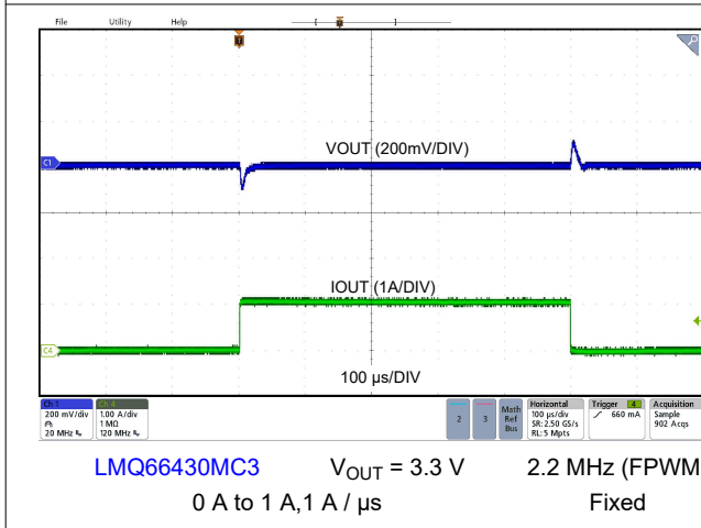
8-12. Load Transient
