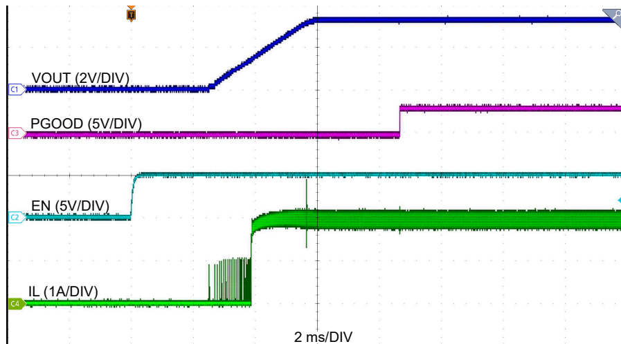
☒ 7-3. Enable Start-Up V_{IN} = 24\text{ V} , V_{OUT} = 3.3\text{ V} , I_{OUT} = 2\text{ A}
