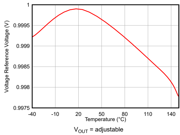
6-4. Feedback Voltage Accuracy Versus Temperature
