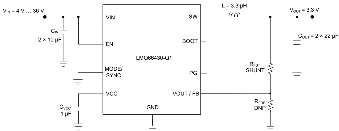
☒ 8-1. Application Circuit 1 - 3.3 V (fixed), 3 A, 2.2 MHz
