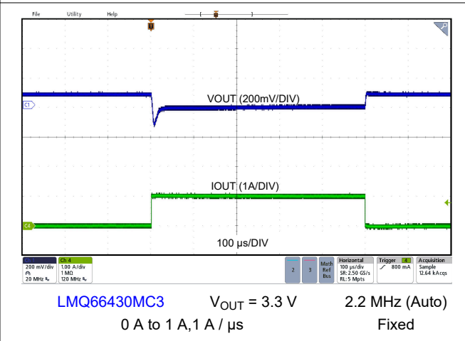
8-13. Load Transient
