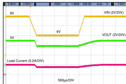
7-11. Typical Output Recovery from Dropout from 8 V to 4 V
