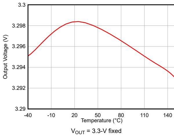
6-3. Output Voltage Accuracy Versus Temperature
