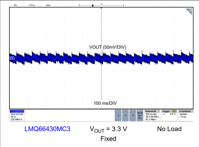
8-15. Output Voltage Ripple
