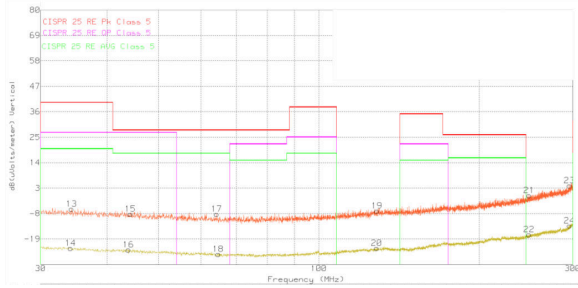
8-22. CISPR 25 Class 5 Radiated EMI, Biconical Antenna, Vertical Polarization, 30 MHz - 300 MHz Orange: Peak Detect, Yellow: Average Detect
