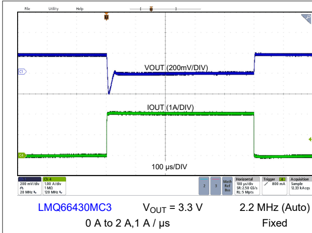
8-10. Load Transient
