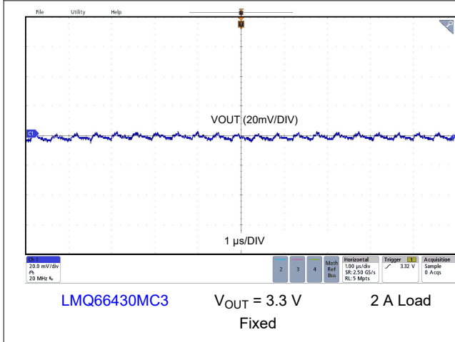
8-14. Output Voltage Ripple
