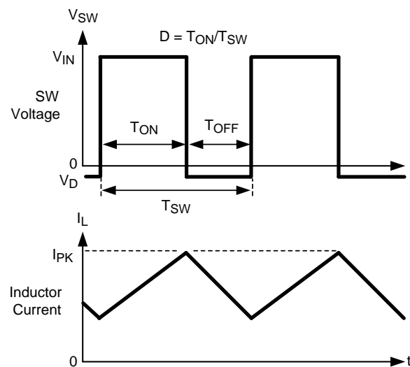
Figure 13. Typical Waveforms
