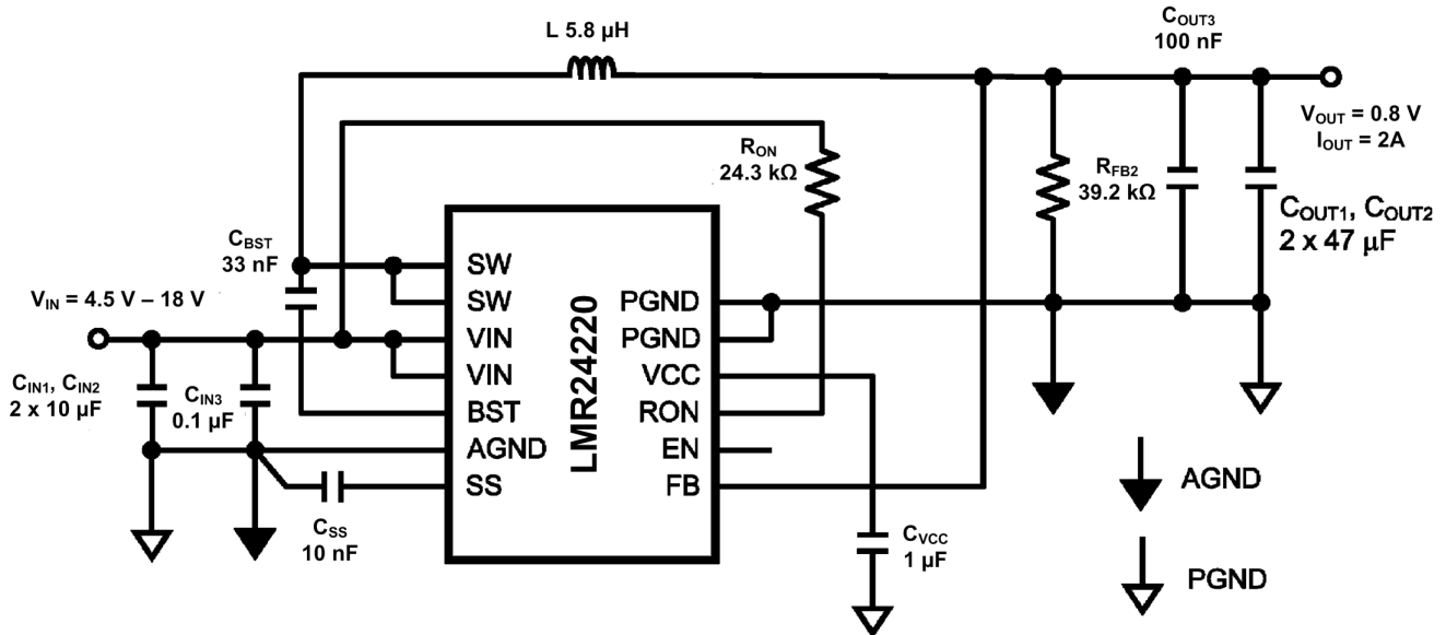
Figure 26. Typical Application Schematic For V_{OUT} = 0.8 V
