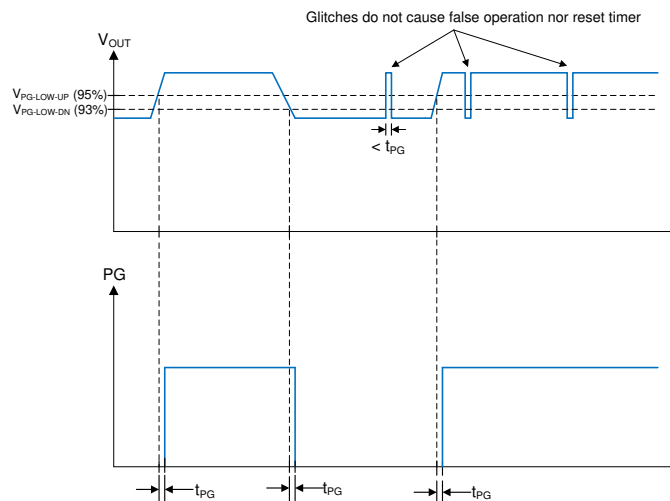
Figure 8. Power-Good-Timing Behavior
