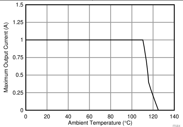
Figure 20. Maximum Output Current versus Ambient Temperature
