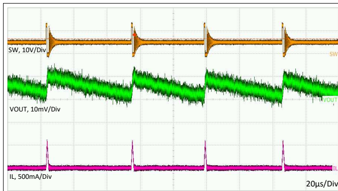
Figure 13. Typical PFM Switching Waveforms V_{IN} = 12\text{ V} , V_{OUT} = 5\text{ V} , I_{OUT} = 10\text{ mA}
