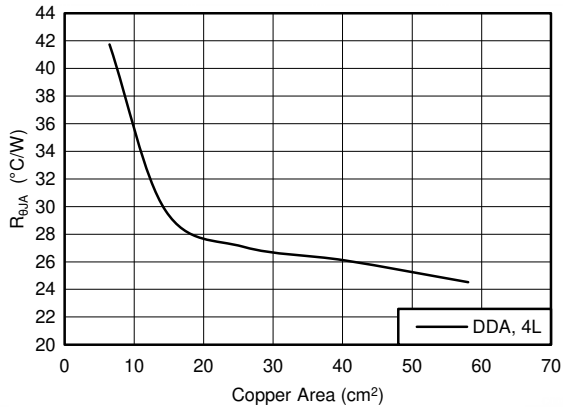
Figure 19. Typical R θJA versus Copper Area for a Four-Layer Board and the HSOIC (DDA) Package
