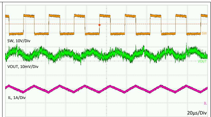
Figure 14. Typical PWM Switching Waveforms V_{IN} = 12\text{ V} , V_{OUT} = 5\text{ V} , I_{OUT} = 1\text{ A} , f_s = 400\text{ kHz}
