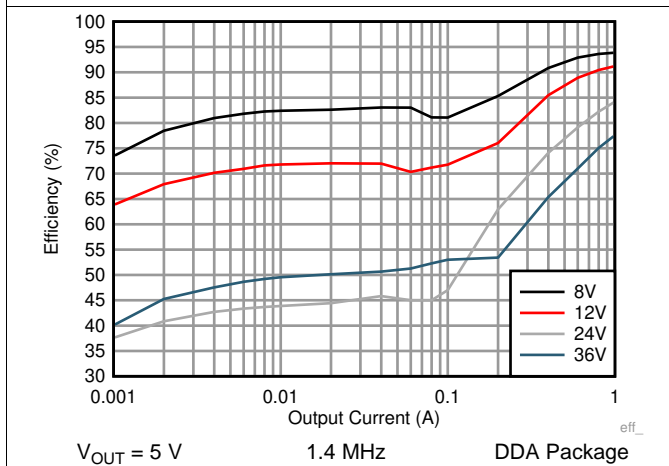
Figure 24. Efficiency
