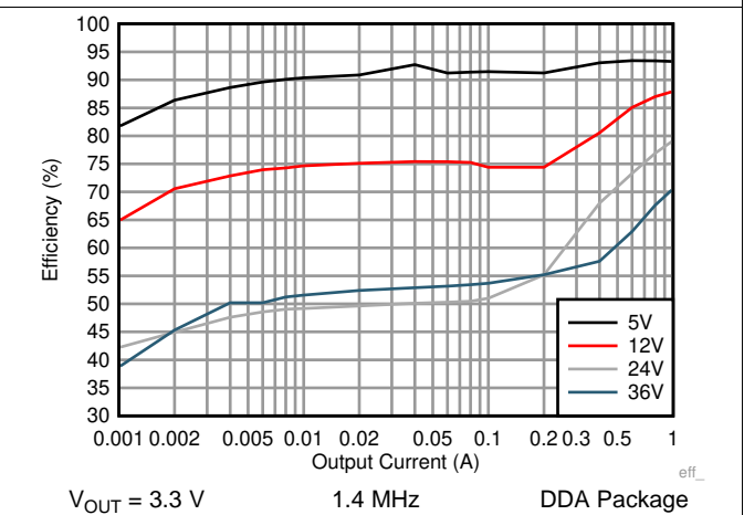
Figure 25. Efficiency
