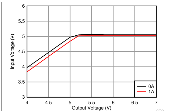
Figure 15. Overall Dropout Characteristic V_{OUT} = 5\text{ V}
