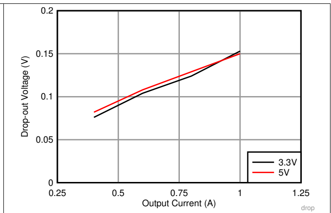
Figure 16. Typical Dropout Voltage versus Output Current in Frequency Foldback f_{sw} = 140\text{ kHz}
