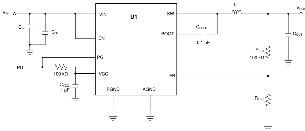
图 36. Circuit for Application Curves
