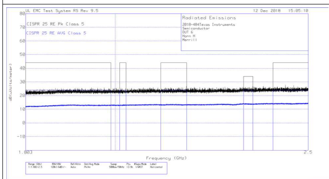
☒ 39. Radiated EMI Log Horizontal vs. CISPR25 Limits
