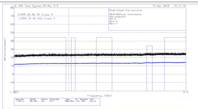
☒ 40. Radiated EMI Horn Vertical vs. CISPR25 Limits
