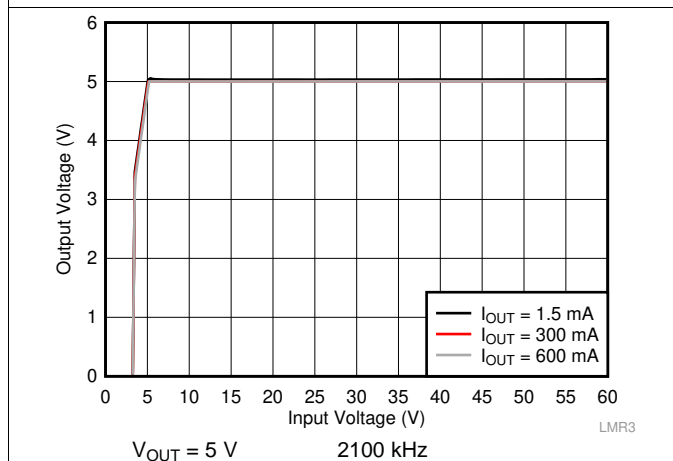
图 47. Line Regulation
