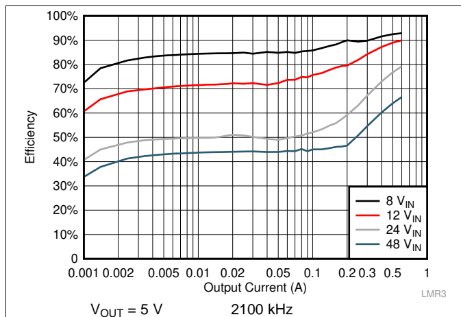
图 43. Efficiency
