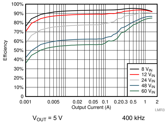
10-4. Efficiency
