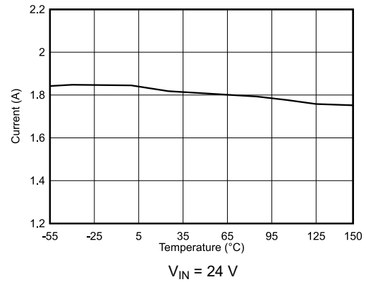
8-4. Low Side Current Limit
