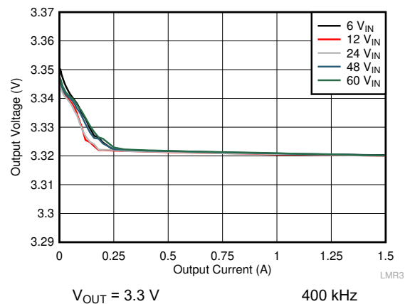
10-7. Load Regulation
