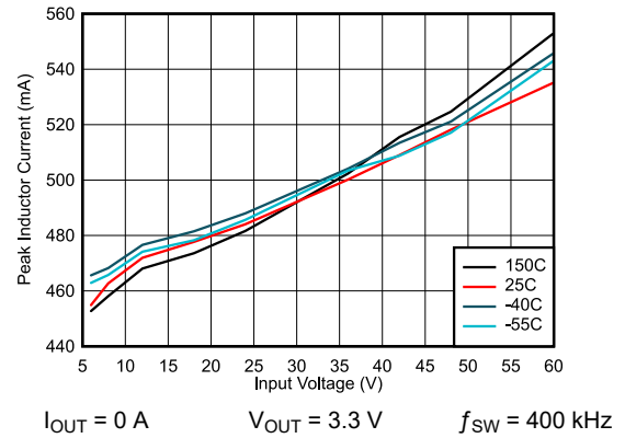
8-6. I_{PEAK-MIN}
