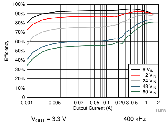
10-5. Efficiency
