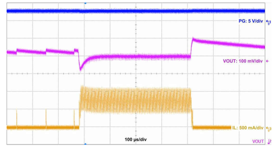
10-17. Load Transient
