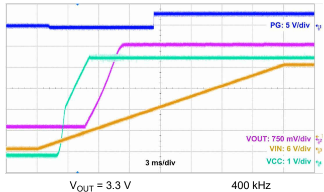
10-15. Start-Up Waveform
