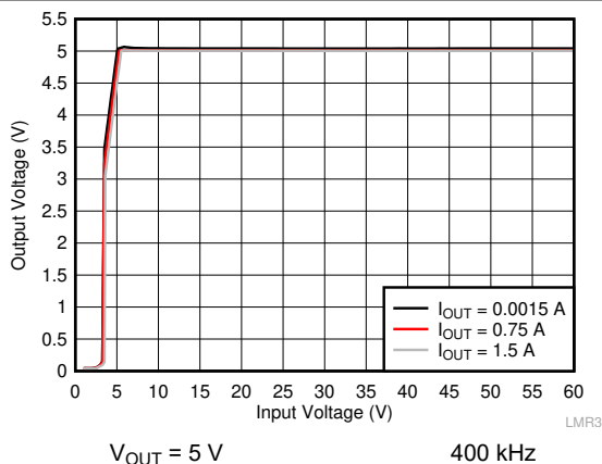
10-8. Line Regulation
