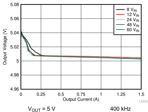
10-6. Load Regulation
