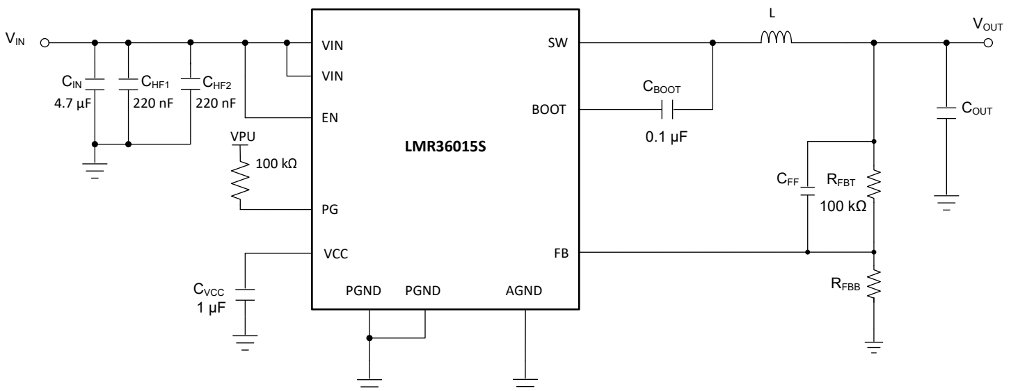
☒ 10-1. Example Applications Circuit
