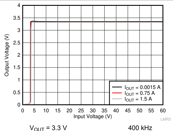
10-9. Line Regulation
