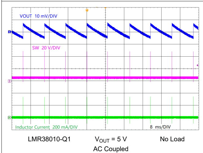
8-5. PFM Switching
