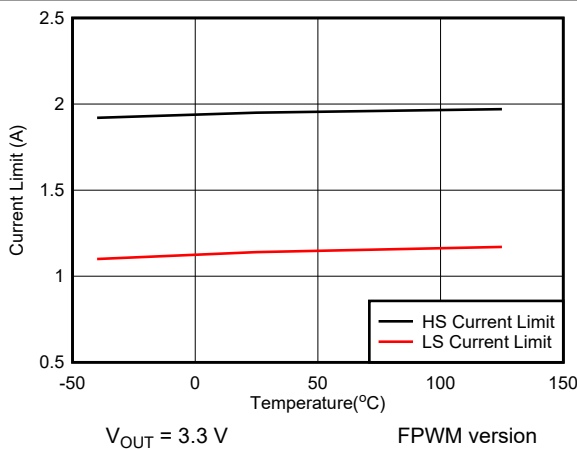
6-5. High-Side and Low-Side Current Limit vs Temperature
