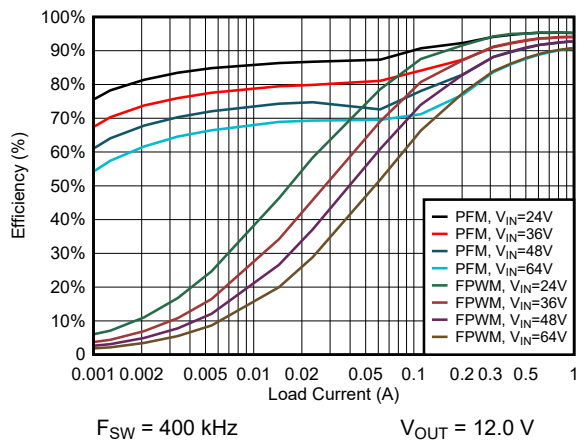
6-1. Efficiency vs Load Current
