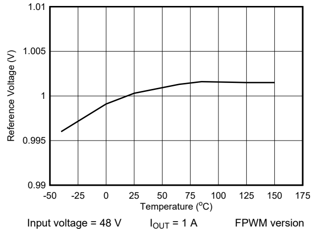
6-4. Reference Voltage vs Temperature
