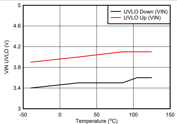
6-6. V_{IN} UVLO vs Temperature
