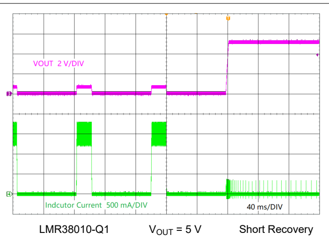
8-8. Short-Circuit Recovery
