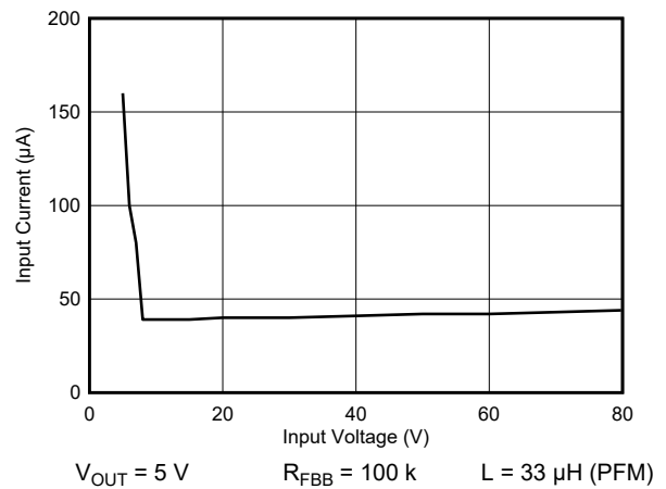
6-2. No Load Input Current vs Input Voltage
