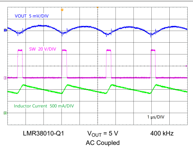
8-6. Full Load Switching
