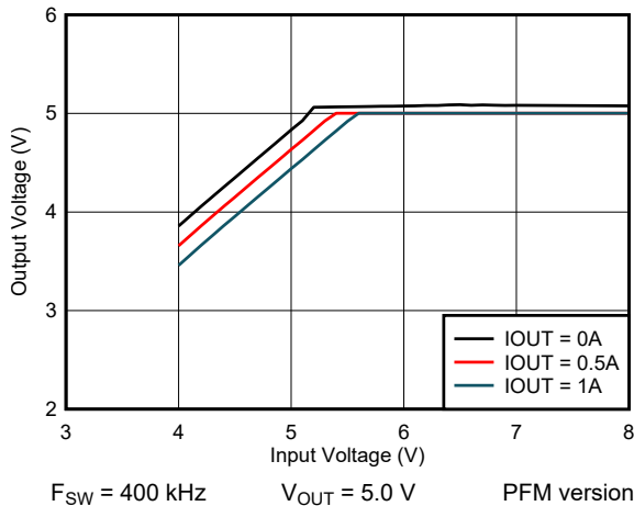
6-3. 5-V Dropout
