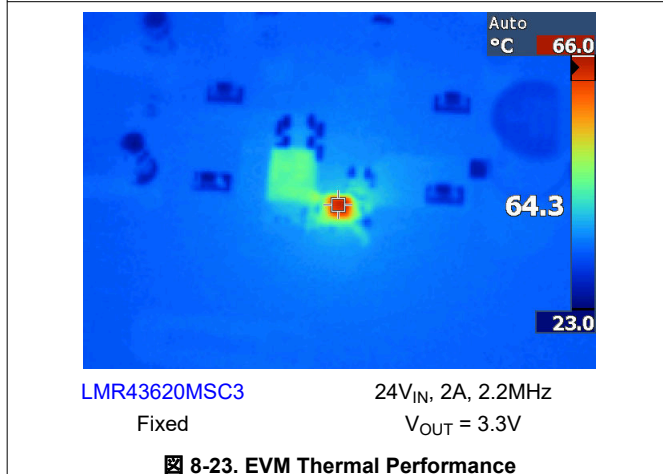
8-23. EVM Thermal Performance
