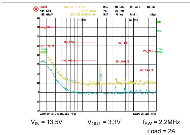
8-25. Typical CISPR 25 Conducted EMI 150kHz–30MHz Yellow: Peak Detect, Blue = Average Detect
