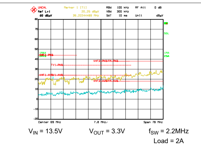
8-26. Typical CISPR 25 Conducted EMI 30MHz–108MHz Yellow: Peak Detect, Blue = Average Detect
