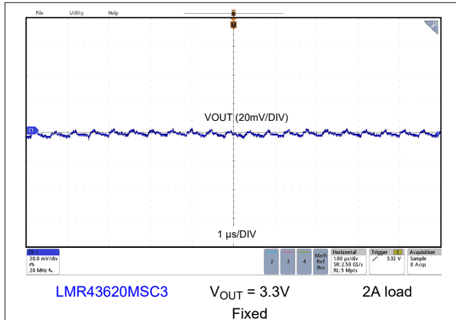
8-21. Output Voltage Ripple
