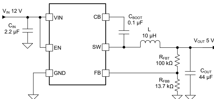
図 9-1. Application Circuit
