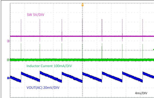
☒ 8-3. Ripple at No Load
