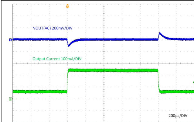
☒ 8-7. Load Transient (60mA – 240mA)
