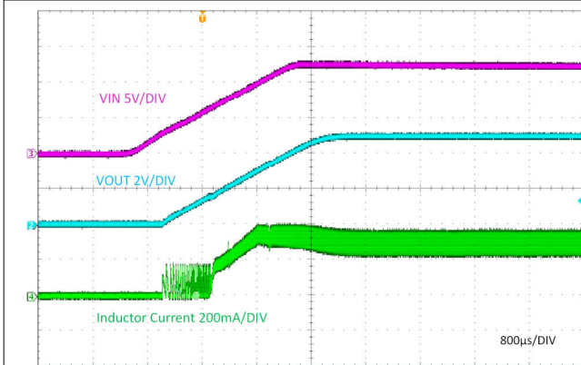
☒ 8-5. Start-Up by V_{IN}
