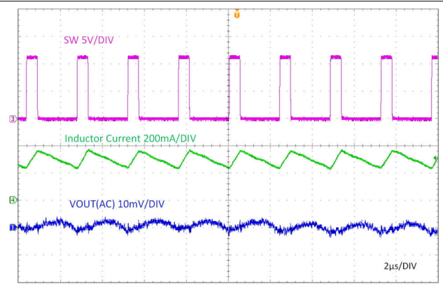
☒ 8-4. Ripple at Full Load
