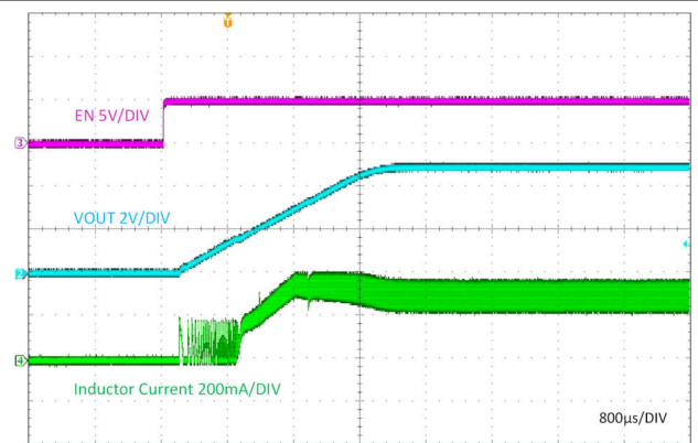
☒ 8-6. Start-Up by EN
