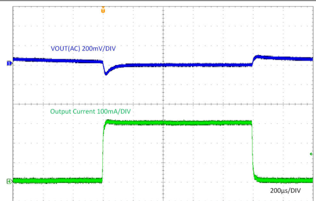
☒ 8-8. Load Transient (0mA – 300mA)
