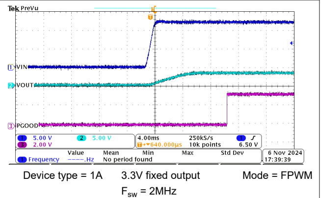
Figure 8-5. Start-up
