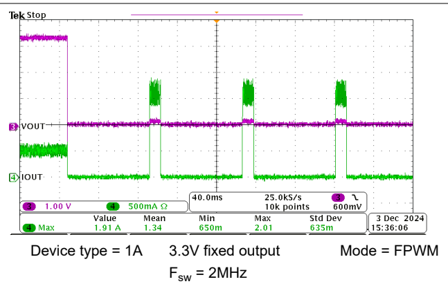
Figure 8-9. Short-Circuit Applied
