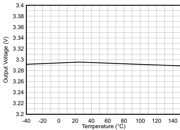
3.3V Fixed Output Figure 6-5. Output Voltage vs Temperature
