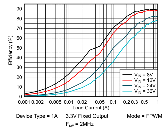
Figure 8-2. Efficiency
