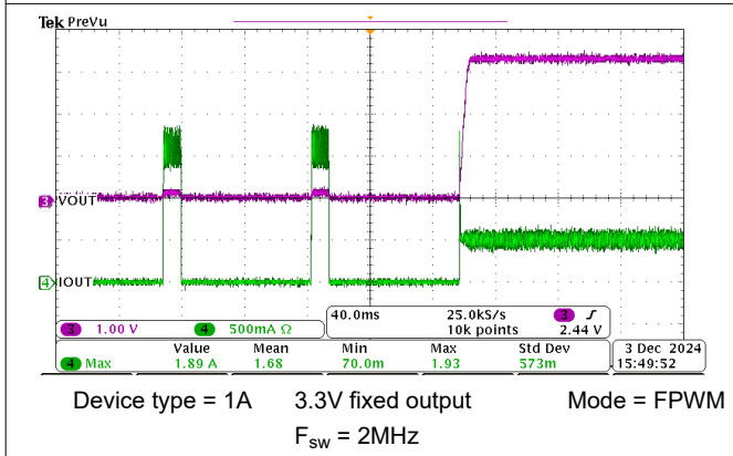
Figure 8-10. Short-Circuit Recovery
