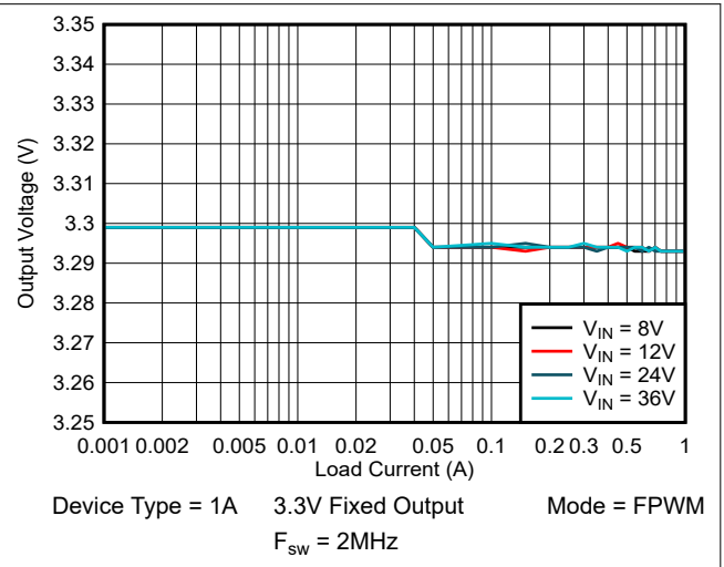
Figure 8-3. Load Regulation
