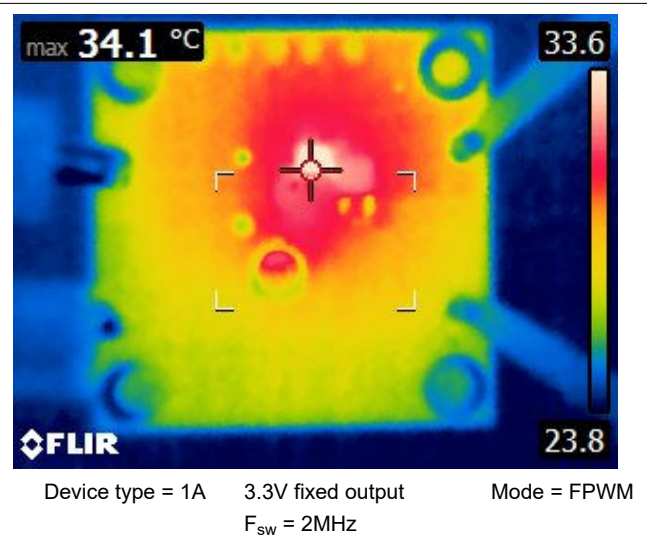
Figure 8-11. Thermal Performance
