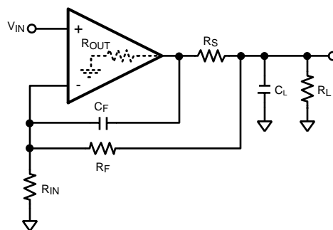
Figure 35. In-the-Loop Compensation
