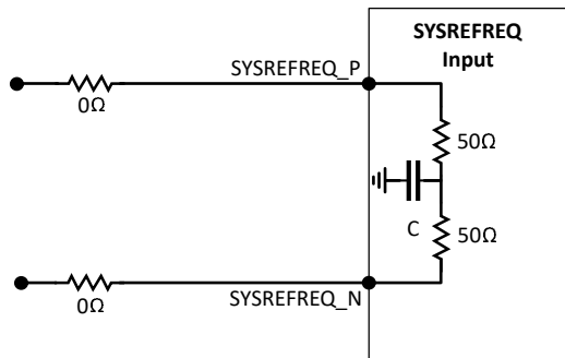
図 7-4. DC-Coupled Differential Input
