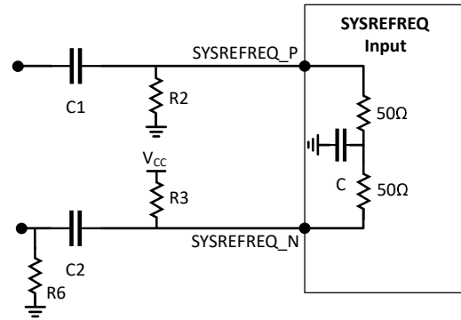
図 7-3. AC-Coupled, Single-Ended Input
