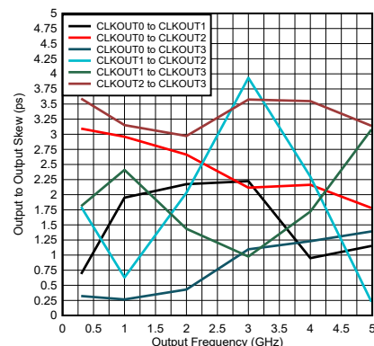
図 5-15. Output to Output Skew (ps)
