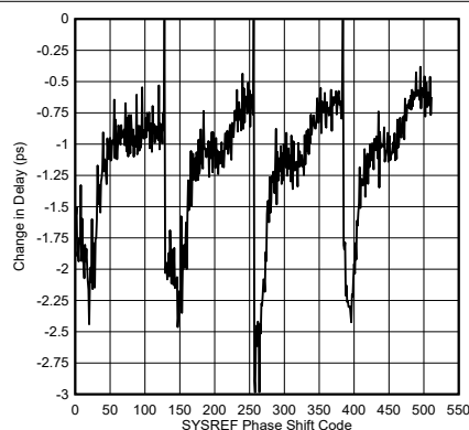
図 5-16. SYSREF Delta Delay vs. Code
