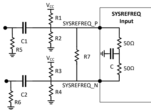
図 7-1. SYSREFREQ Input Circuit Recommendations
