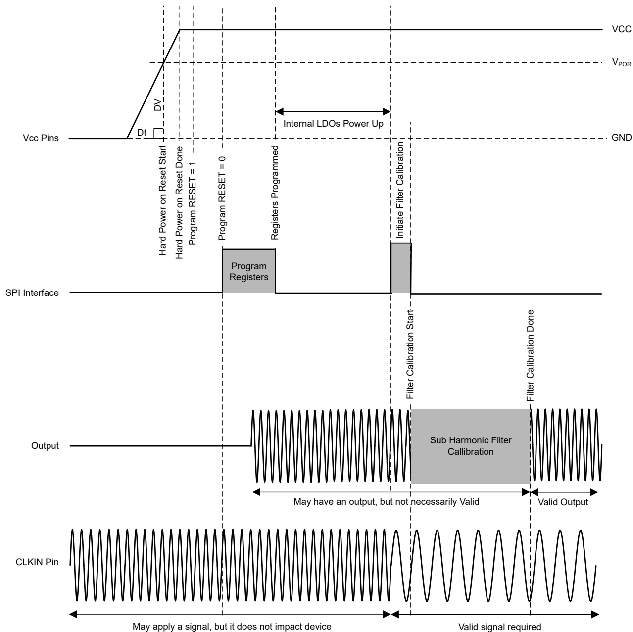
図 7-11. Power-Up Timing
