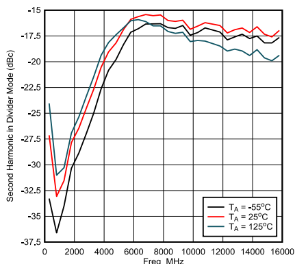
図 5-14. Second Harmonic in Divider Mode (Single-Ended Input)
