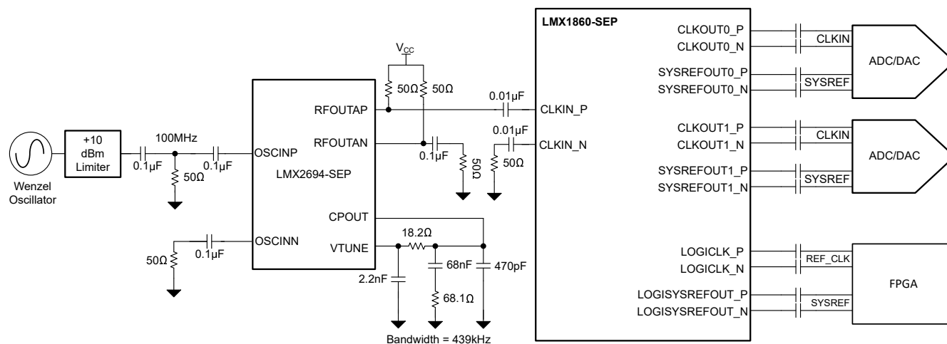
図 7-10. Typical JESD Clocks Block Diagram
