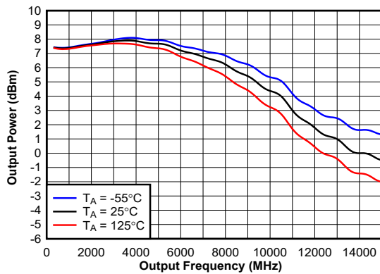
図 5-10. Buffer Mode Single-Ended Output Power
