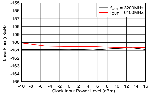
図 5-8. Noise Floor in Multiply x2 Mode
