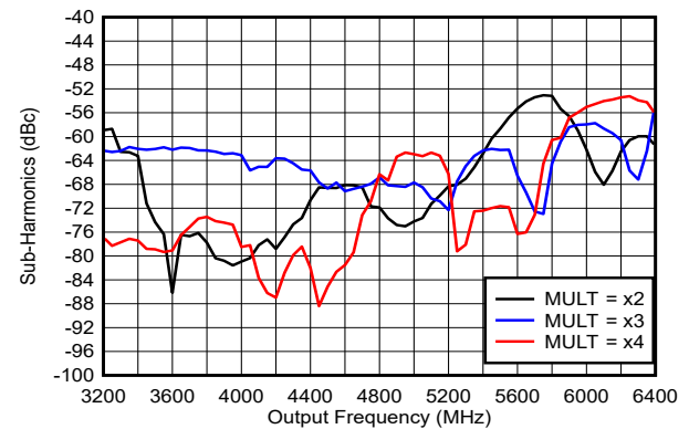
図 5-13. Multiplier Sub-Harmonics (Harmonic Frequency = Output Frequency / M)
