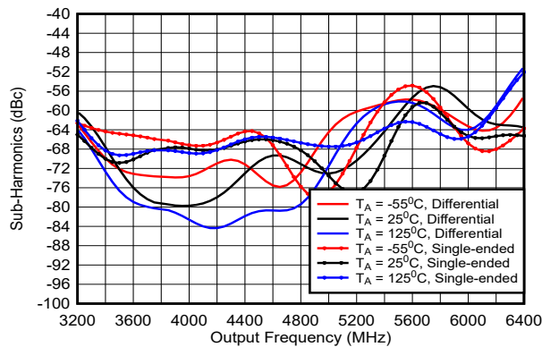
図 5-12. Multiplier 1/2 Sub-Harmonic in X2 Mode
