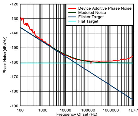
Figure 5-6. Flicker Noise
