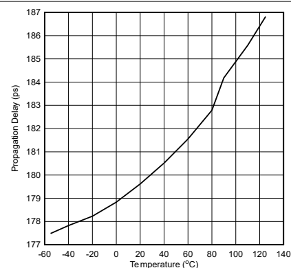
図 5-18. Propagation Delay
