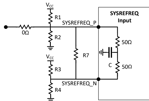
図 7-5. DC-Coupled, Single-Ended Input
