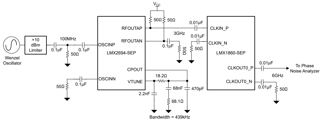
図 7-7. Typical Application Schematic
