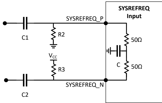
図 7-2. AC-Coupled Differential Input
