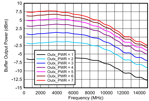
図 5-9. Buffer Mode Single-Ended Output Power
