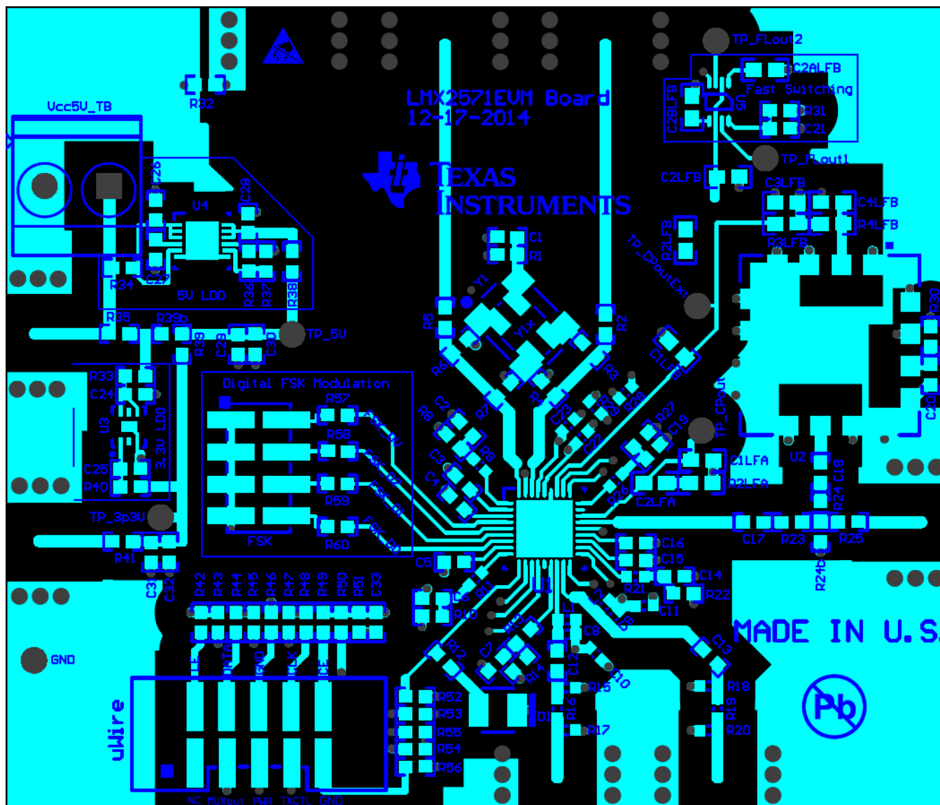
Figure 87. Layout Example
