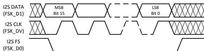
Figure 18. FSK I2S Mode Timing
