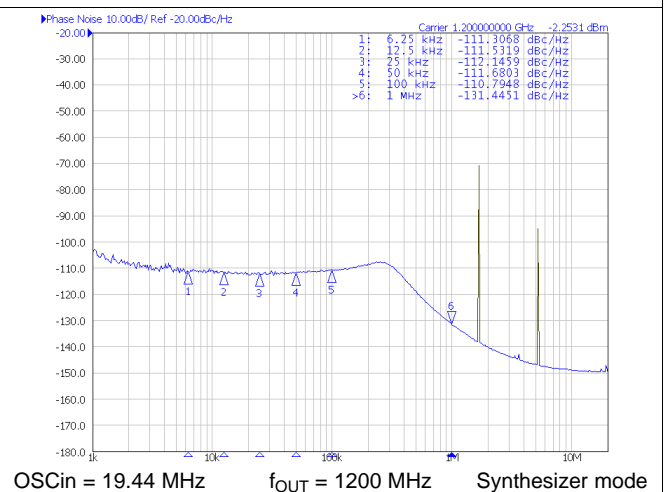
Figure 5. Typical Close Loop Phase Noise
