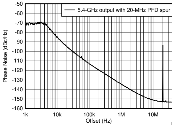
6-14. Typical PFD Spur for 5.4-GHz Output
