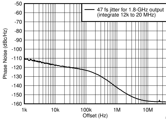
6-8. Integrated Jitter (47 fs) - 1.8-GHz Output
