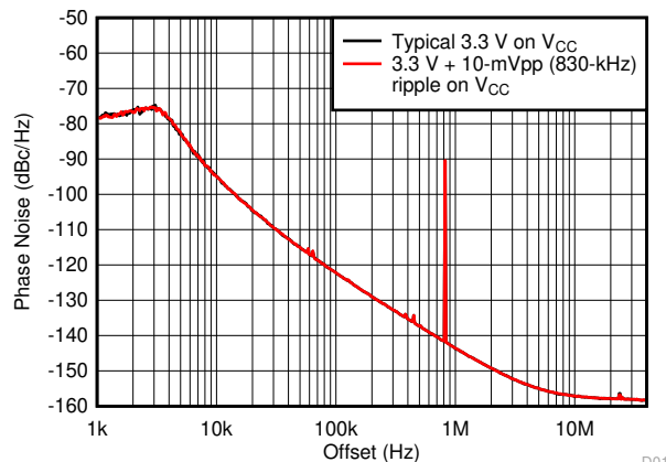
6-11. Impact of Supply Ripple on 1.8-GHz Output Phase Noise
