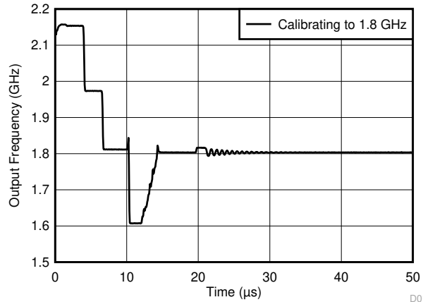
6-15. 20-µs Frequency Change Time to 1.8 GHz With Fast Calibration
