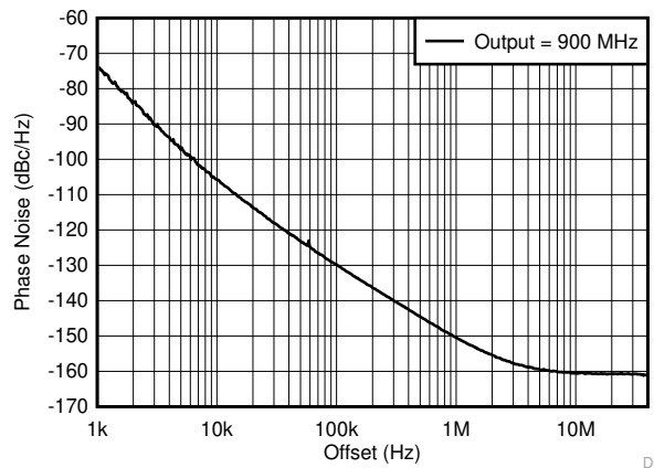
6-3. 900-MHz Output - Open-Loop Phase Noise
