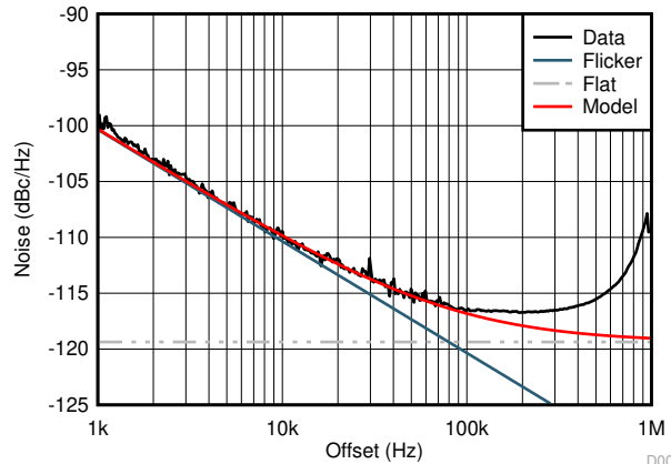
6-9. 5.4-GHz Output Wide Loop Bandwidth – Showing PLL Performance
