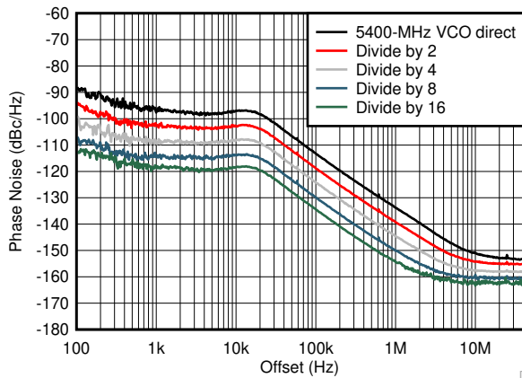
6-16. Impact of Channel Divider Settings on Phase Noise
