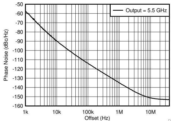
6-7. 5.5-GHz Output - Open-Loop Phase Noise
