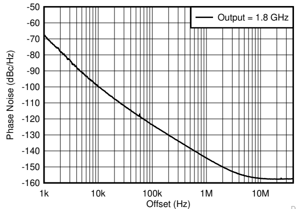
6-5. 1.8-GHz Output - Open-Loop Phase Noise
