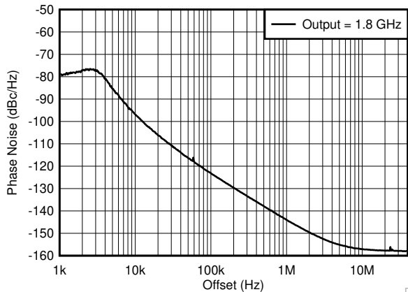
6-4. 1.8-GHz Output - Closed-Loop Phase Noise
