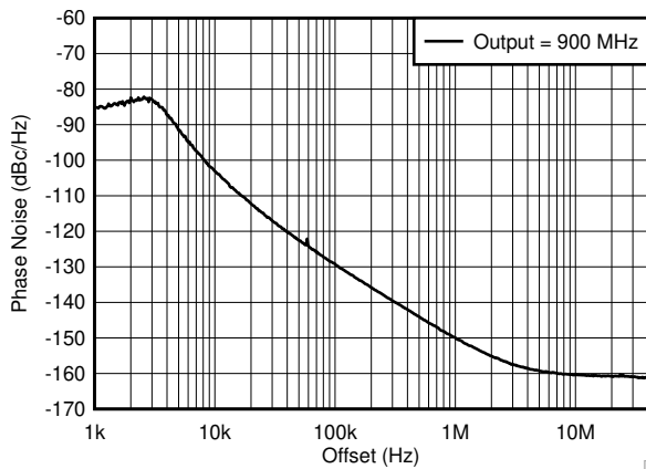
6-2. 900-MHz Output - Closed-Loop Phase Noise
