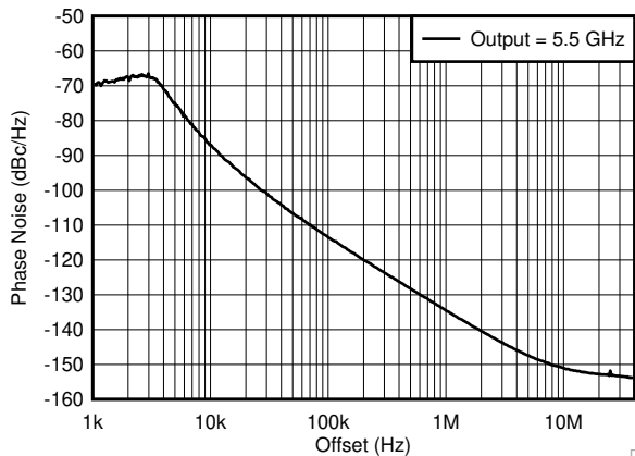
6-6. 5.5-GHz Output - Closed-Loop Phase Noise
