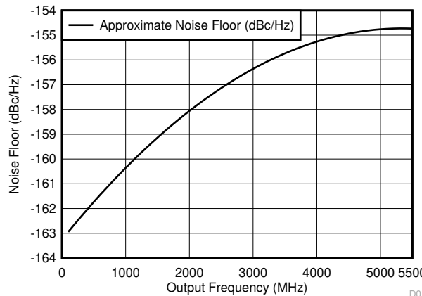
6-17. Noise Floor Variation With Output Frequency
