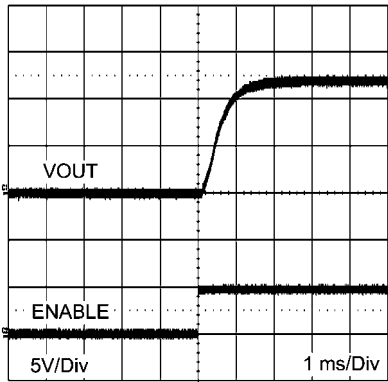
Startup V_{IN} = 24V I_{OUT} = 2A
