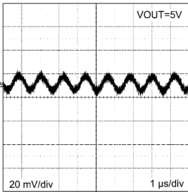
Output Ripple
