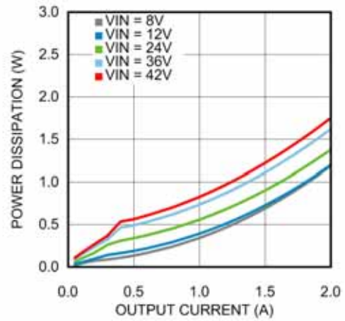
Power Dissipation V_{OUT} = 5.0V T_{AMB} = 25^\circ C
