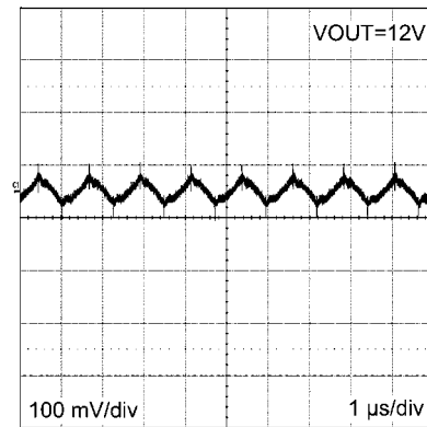
Output Ripple
