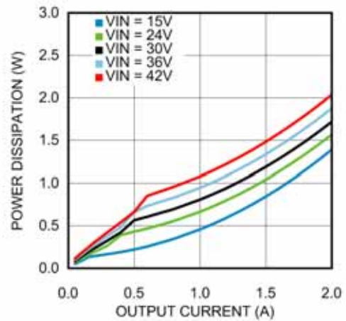
Power Dissipation V_{OUT} = 12V T_{AMB} = 25^\circ C
