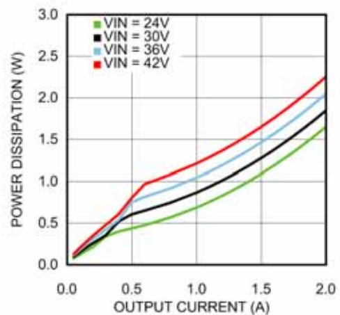
Power Dissipation V_{OUT} = 15V T_{AMB} = 25^\circ C
